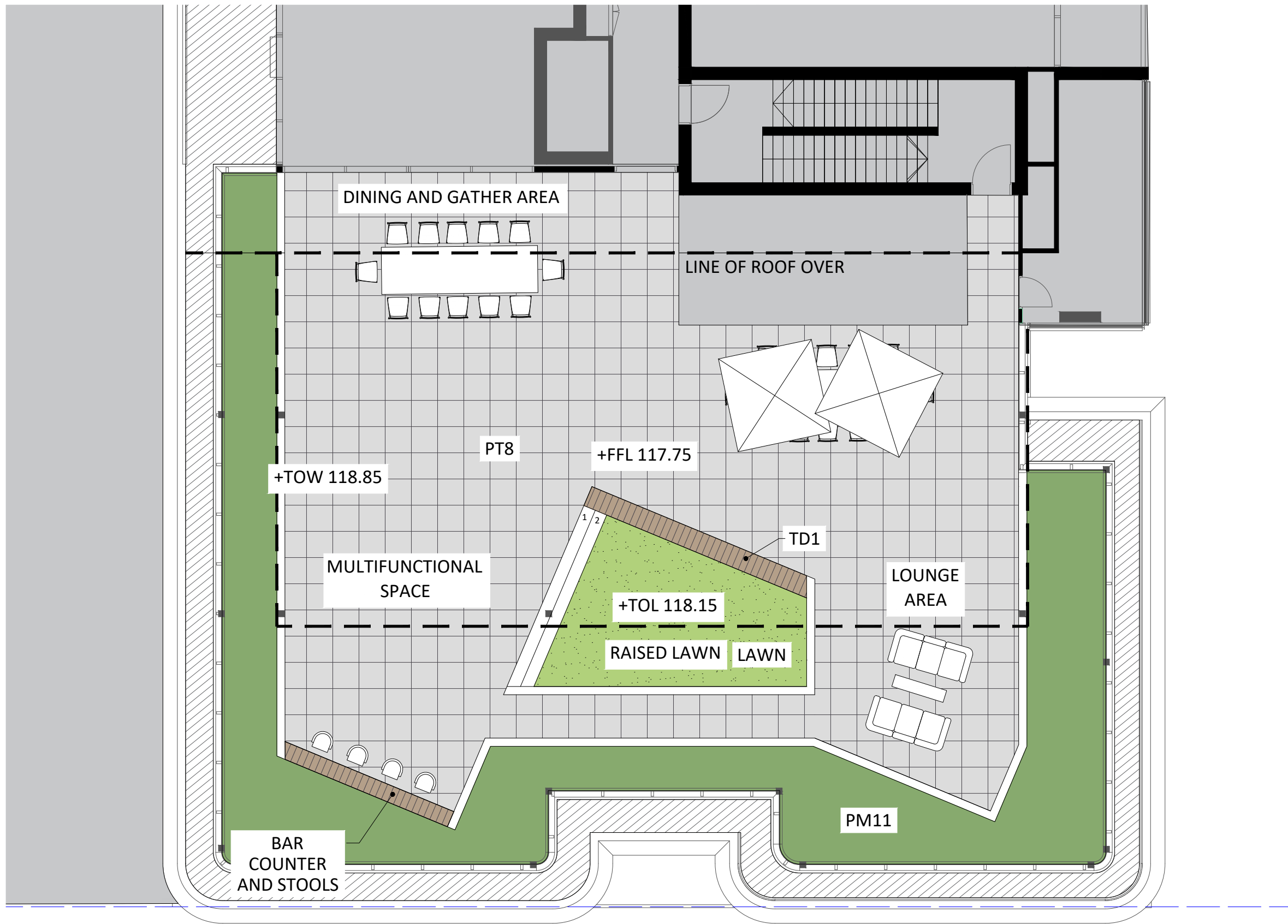
C 0103 BUILDING C ROOFTOP - PLAN SCALE 1:100
