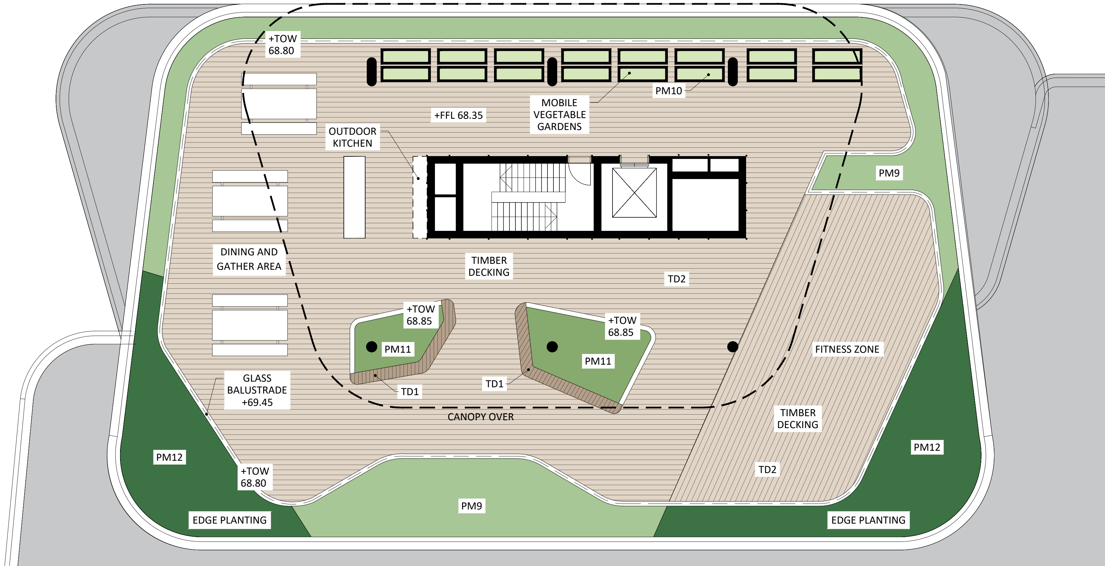
B 0103 BUILDING B ROOFTOP - PLAN SCALE 1:100
