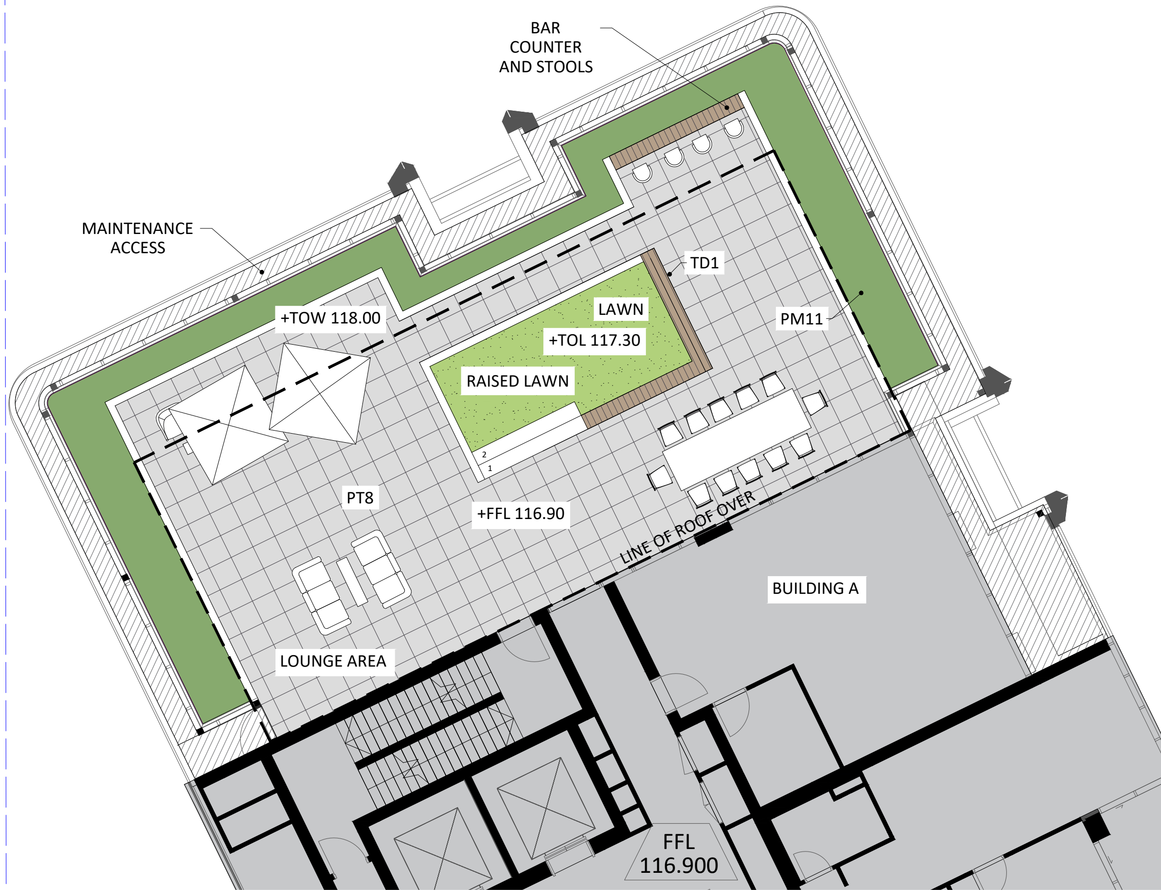
A 0103 BUILDING A ROOFTOP - PLAN SCALE 1:100
