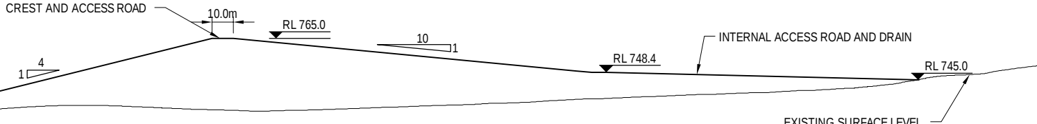
SCALE 1:2500
