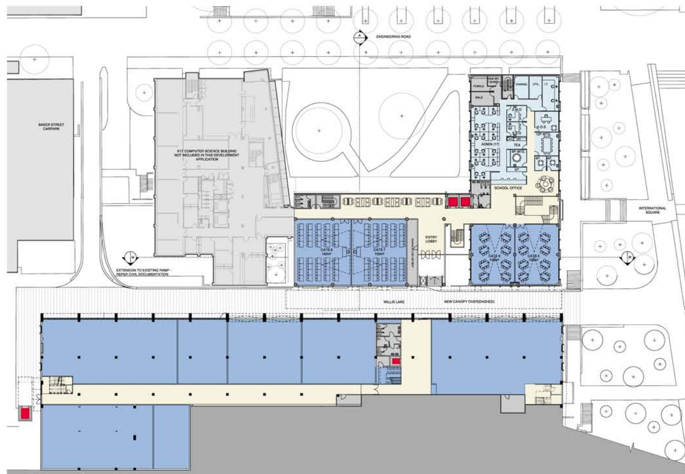
Level 01 Plan 1: 800 @ A3
