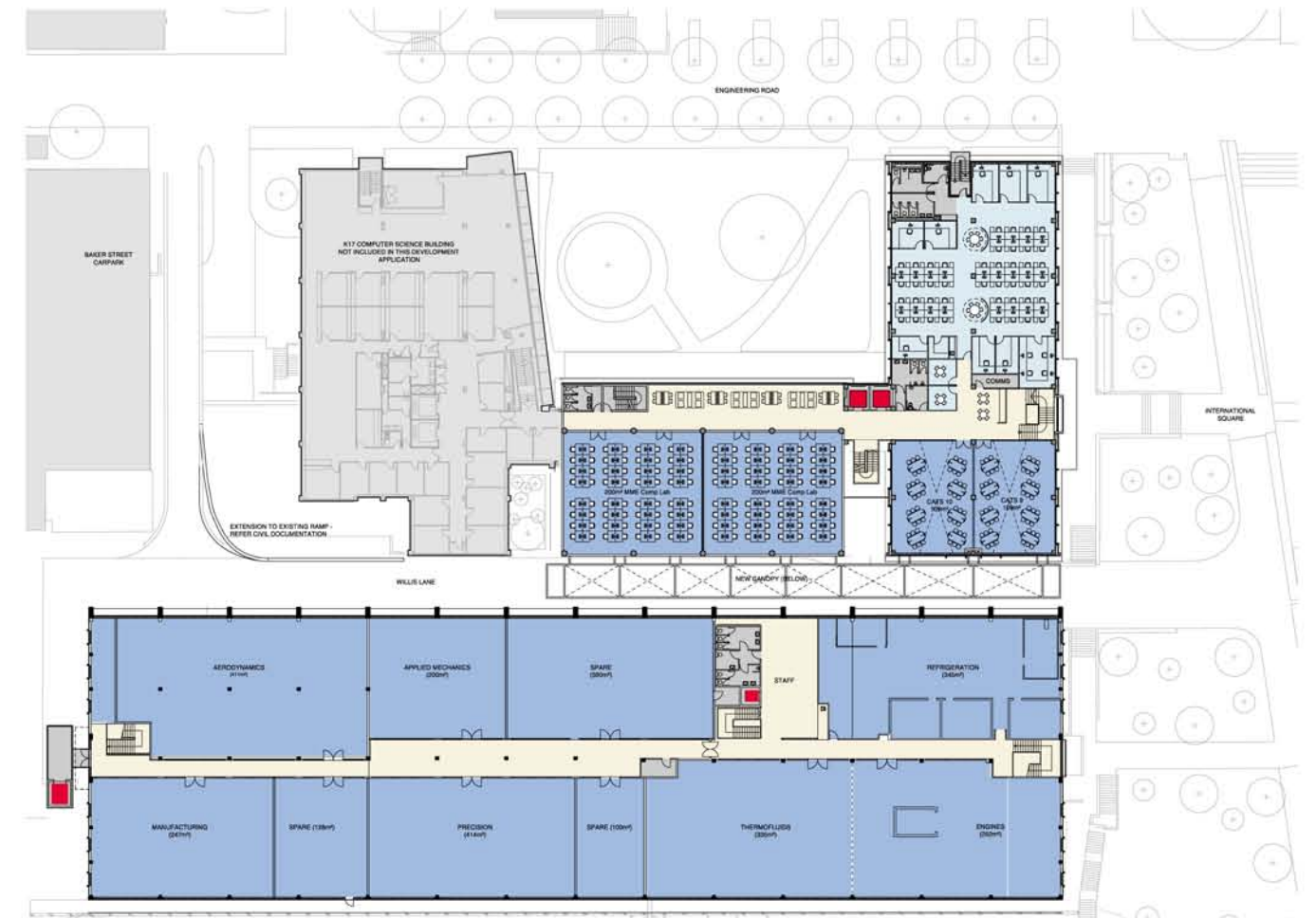
Level 02 Plan 1: 800 @ A3
