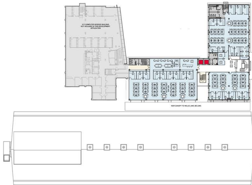
Level 04 Plan 1: 800 @ A3
