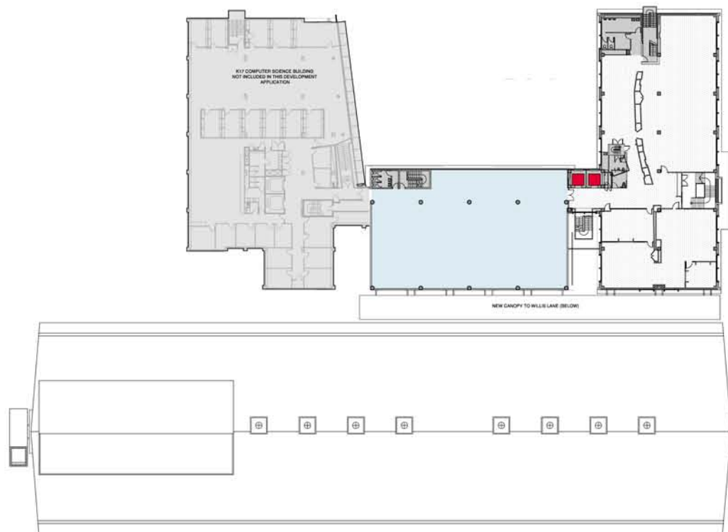
Level 05 Plan 1: 800 @ A3
