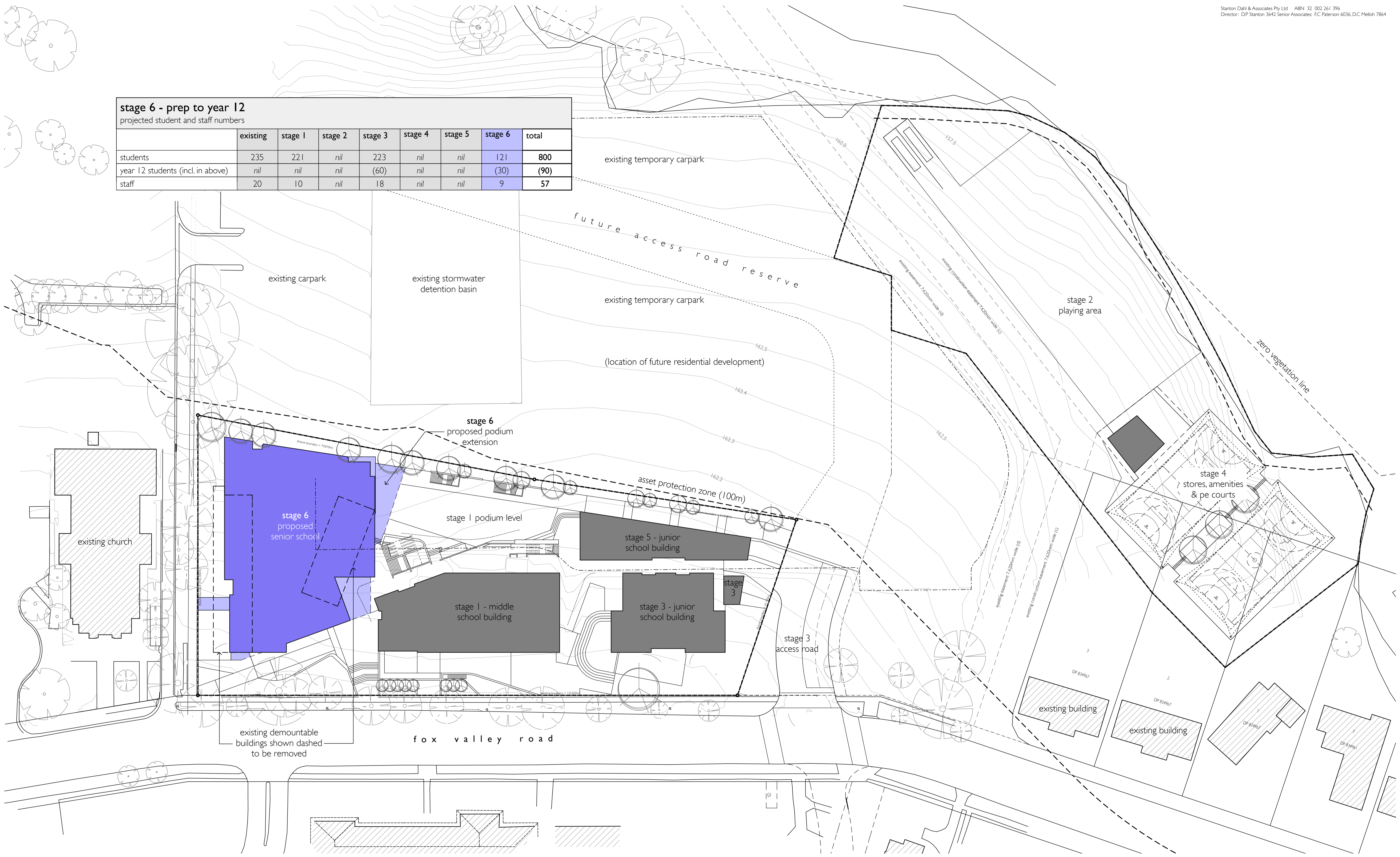
01 staging plan - stage 6 1:400
