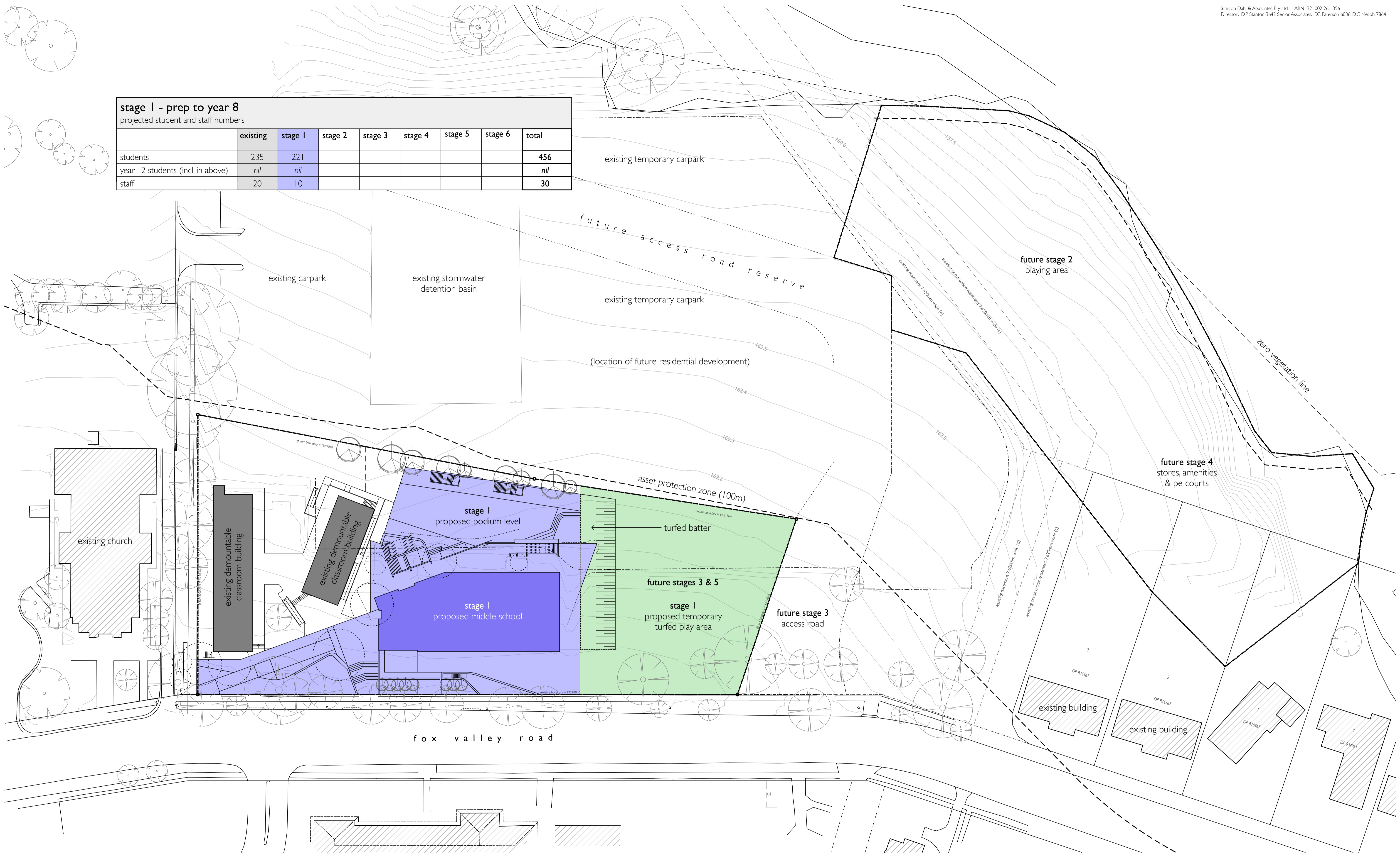
01 staging plan - stage 1 1:400
