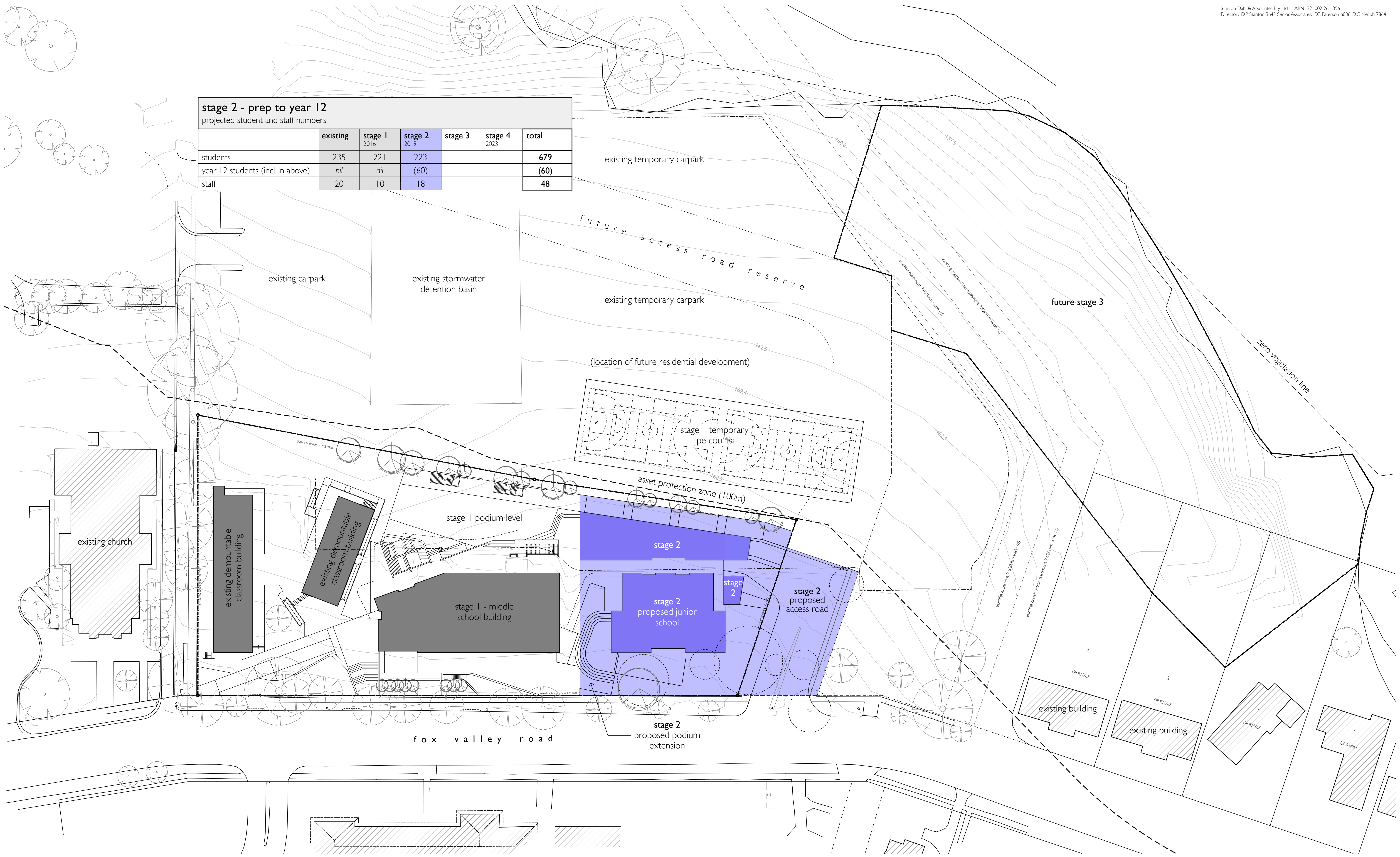
01 staging plan - stage 2 1:400
