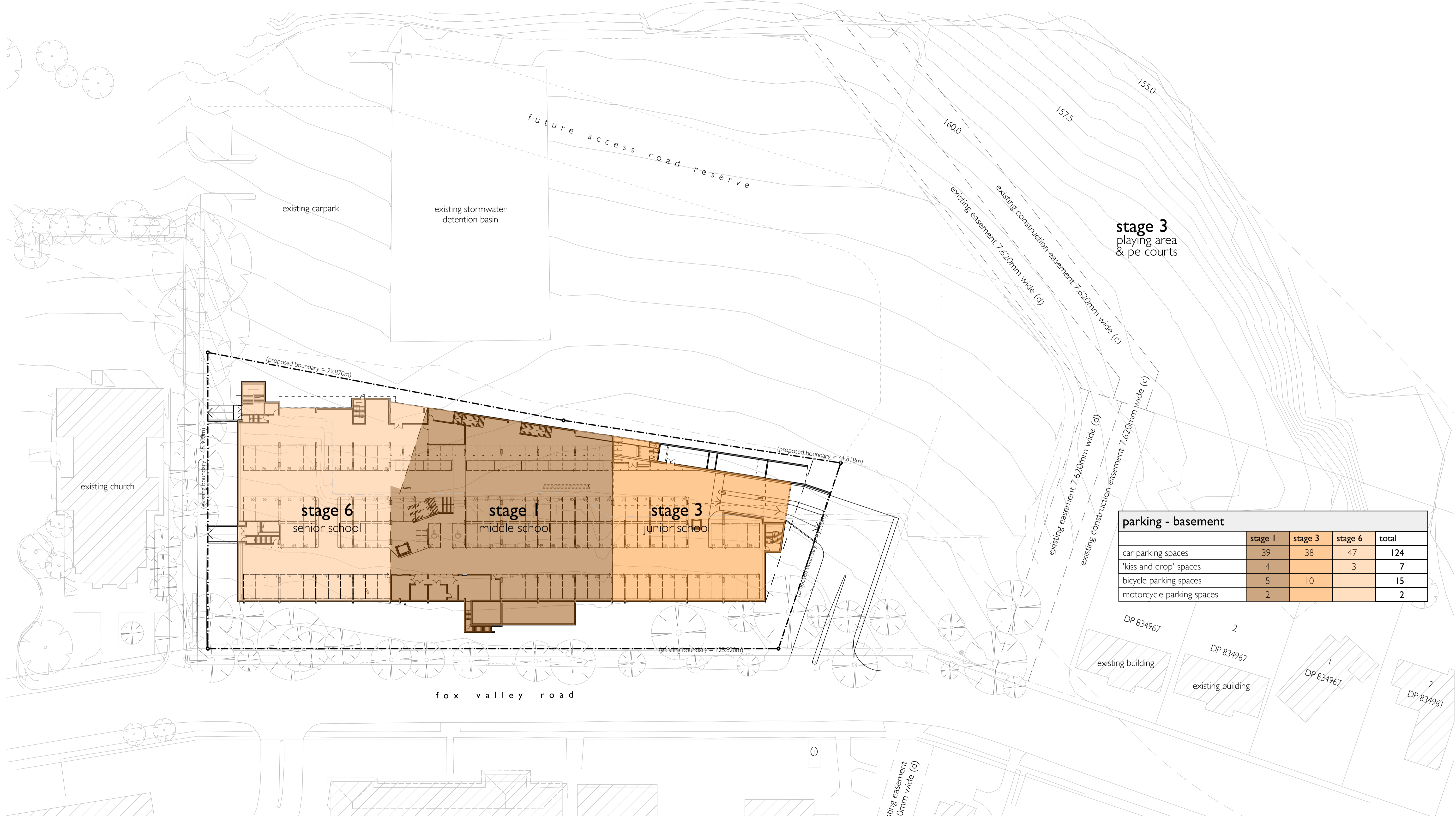
01 basement plan - staging and parking 1:400
