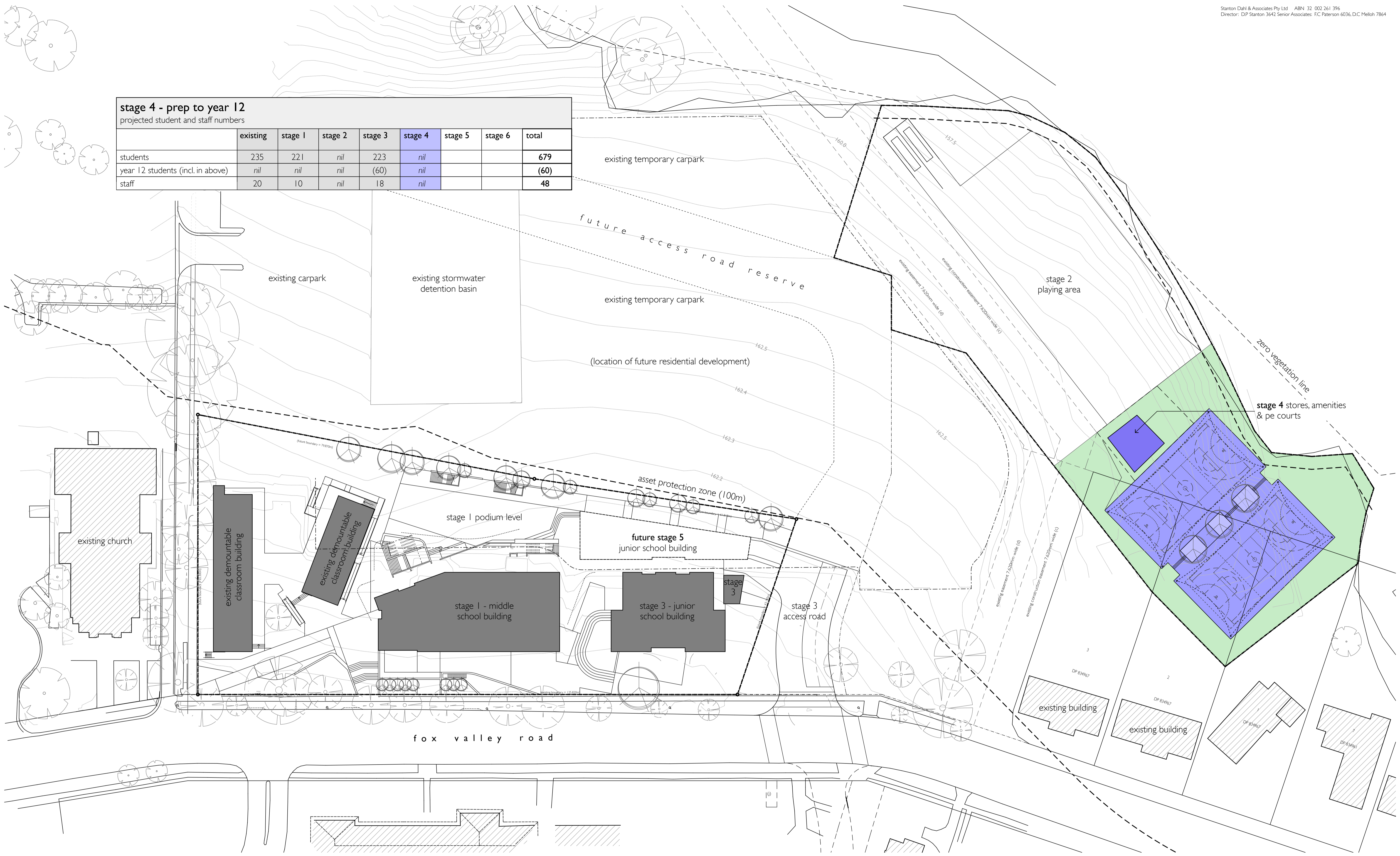
01 staging plan - stage 4 1:400
