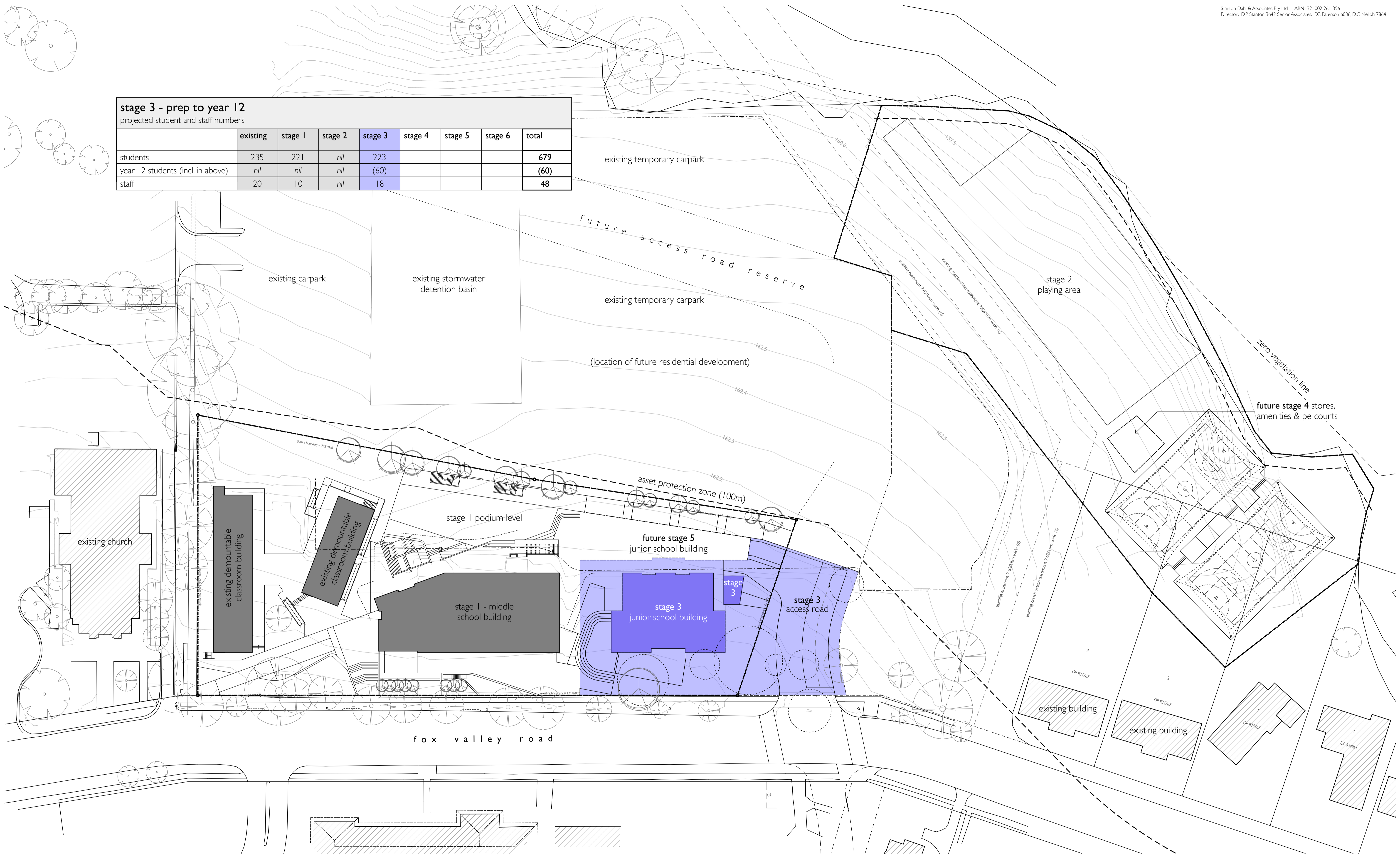
01 staging plan - stage 3 1:400
