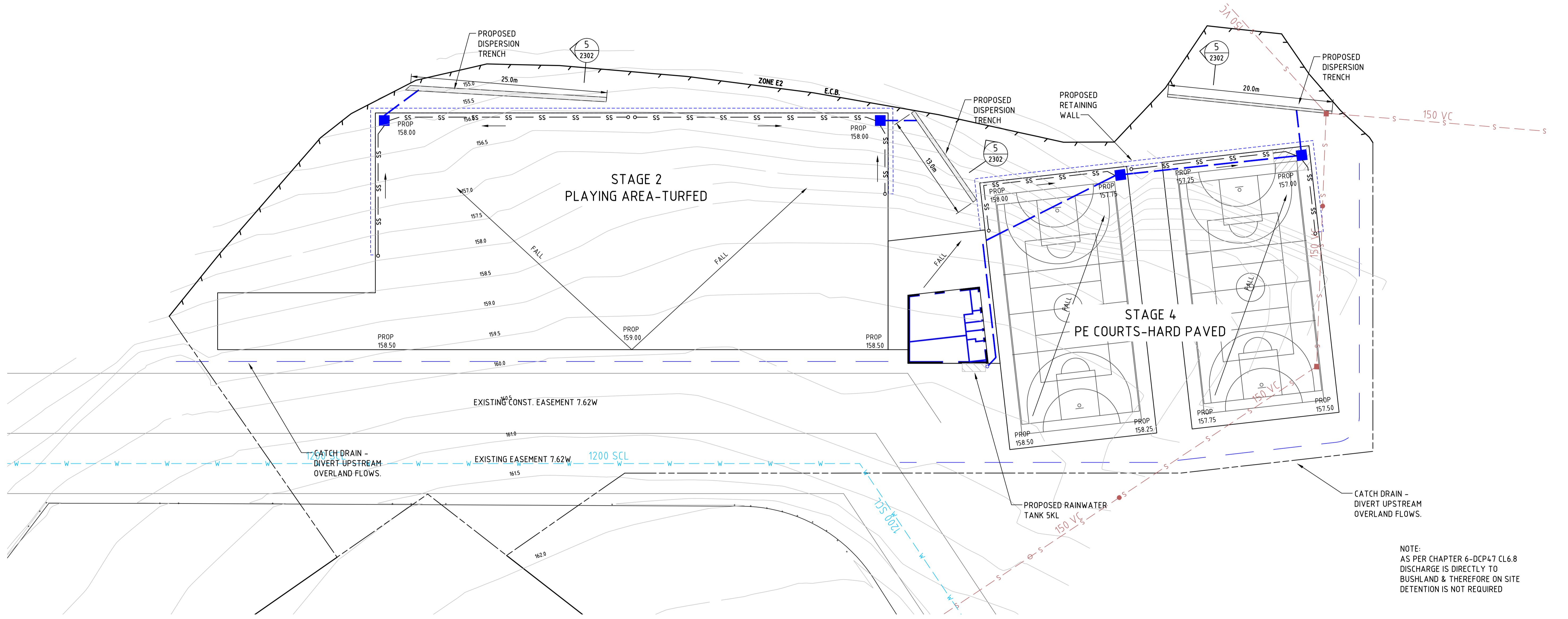
PLAN SCALE:1:250
