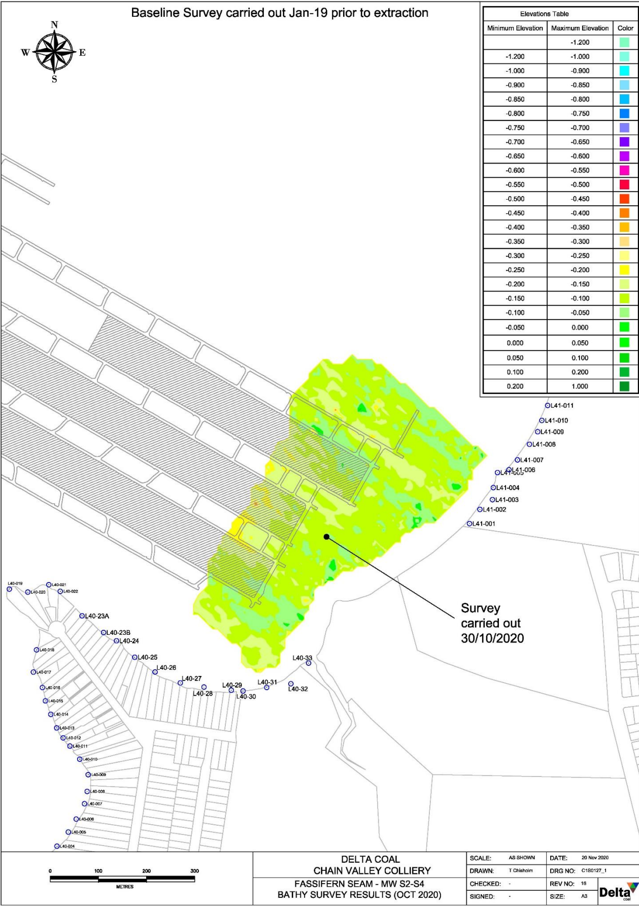
Figure 1: Bathymetric Survey Data S2-S4 October 2020
