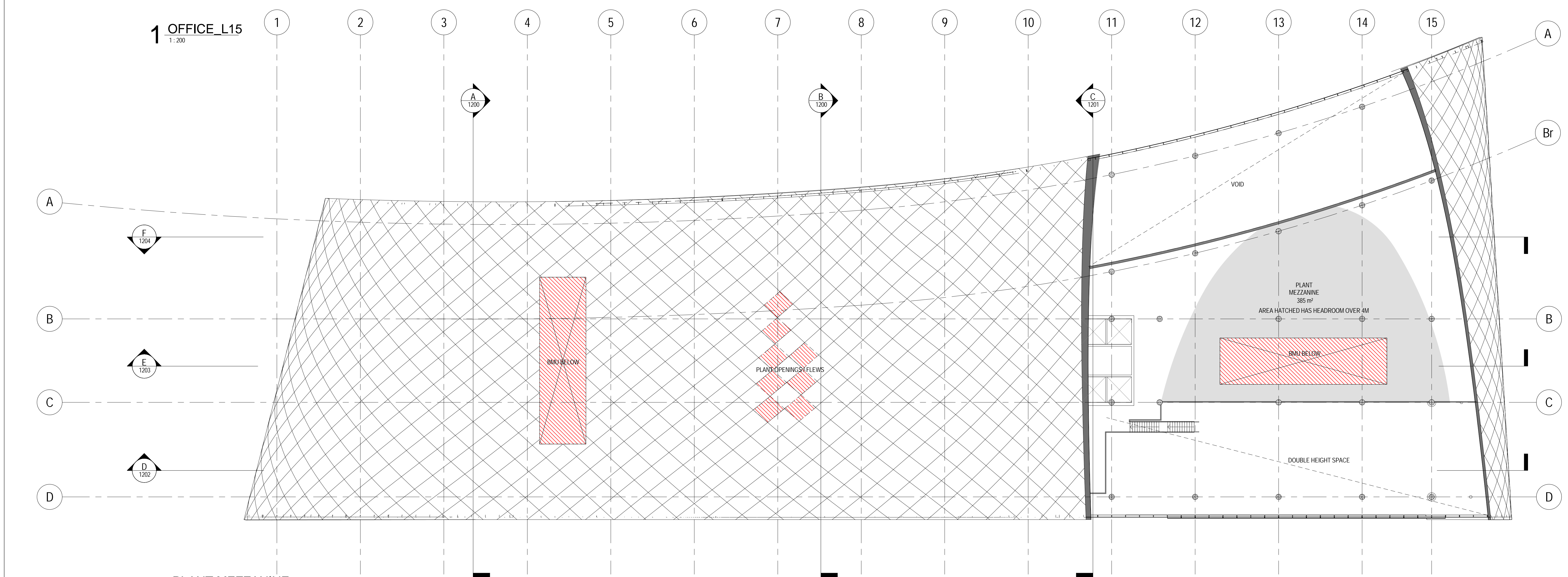
2 PLANT MEZZANINE 1:200
