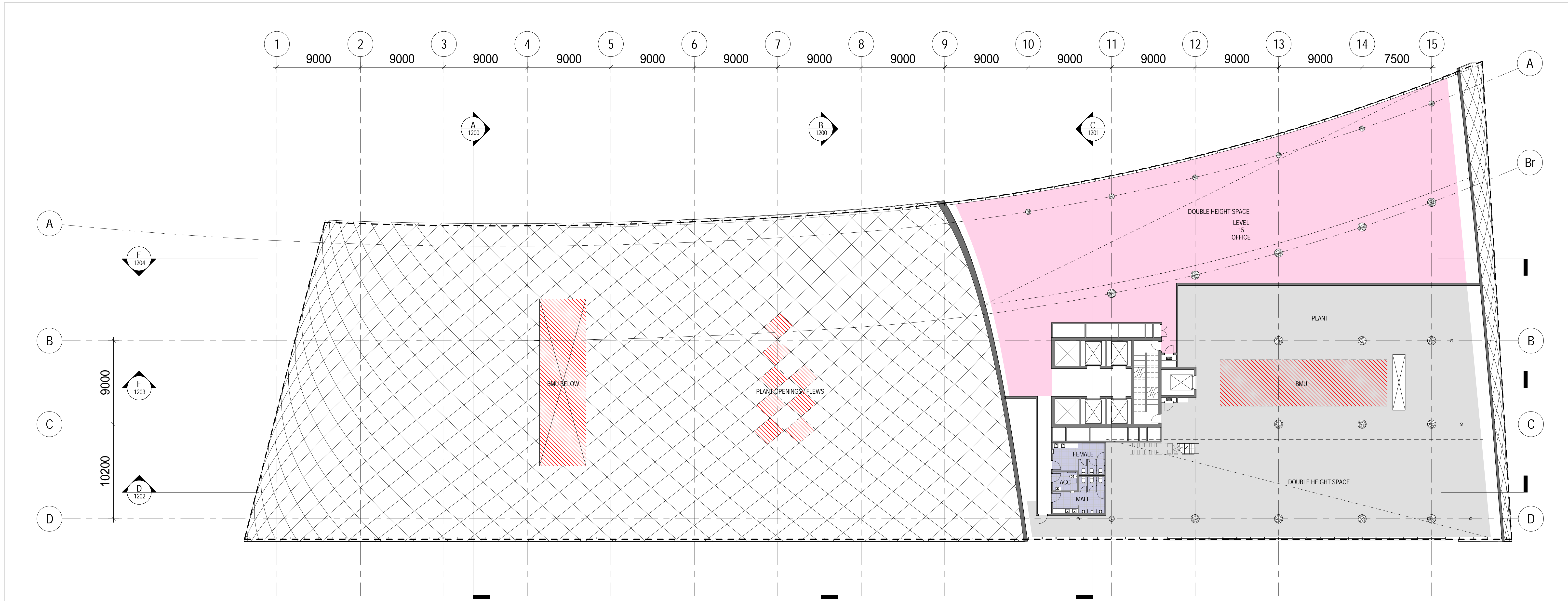
1 OFFICE_L15 1:200
