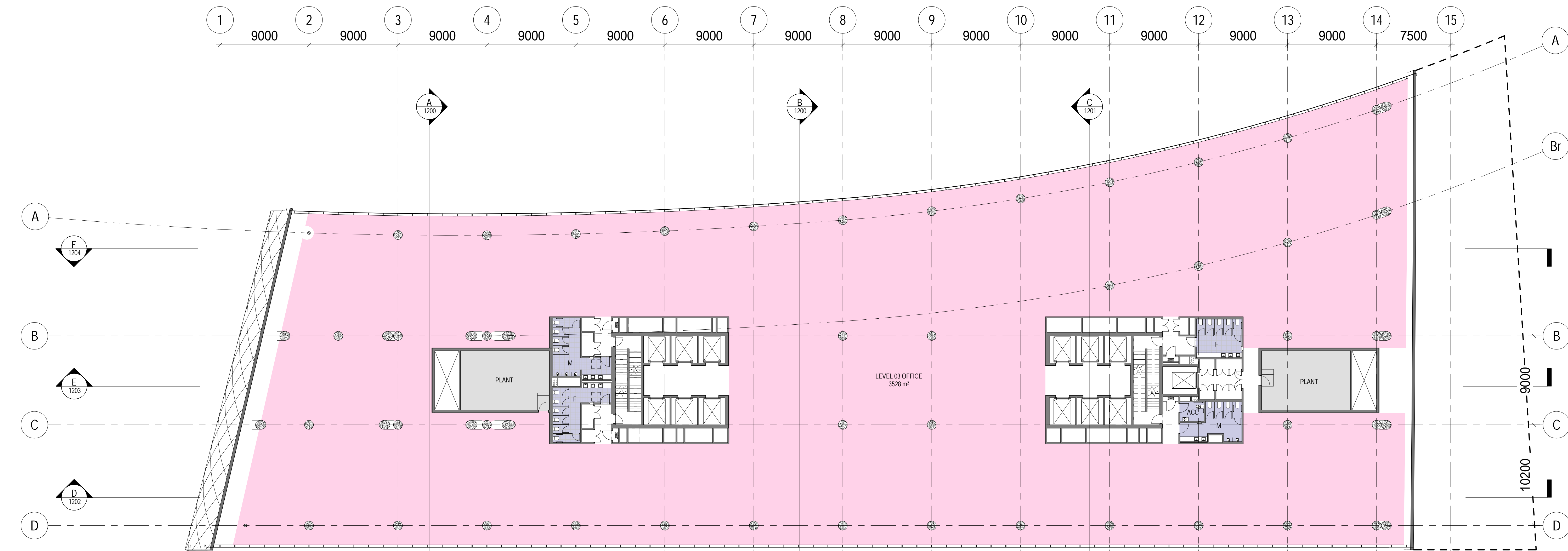
1 OFFICE_L03 1:200
