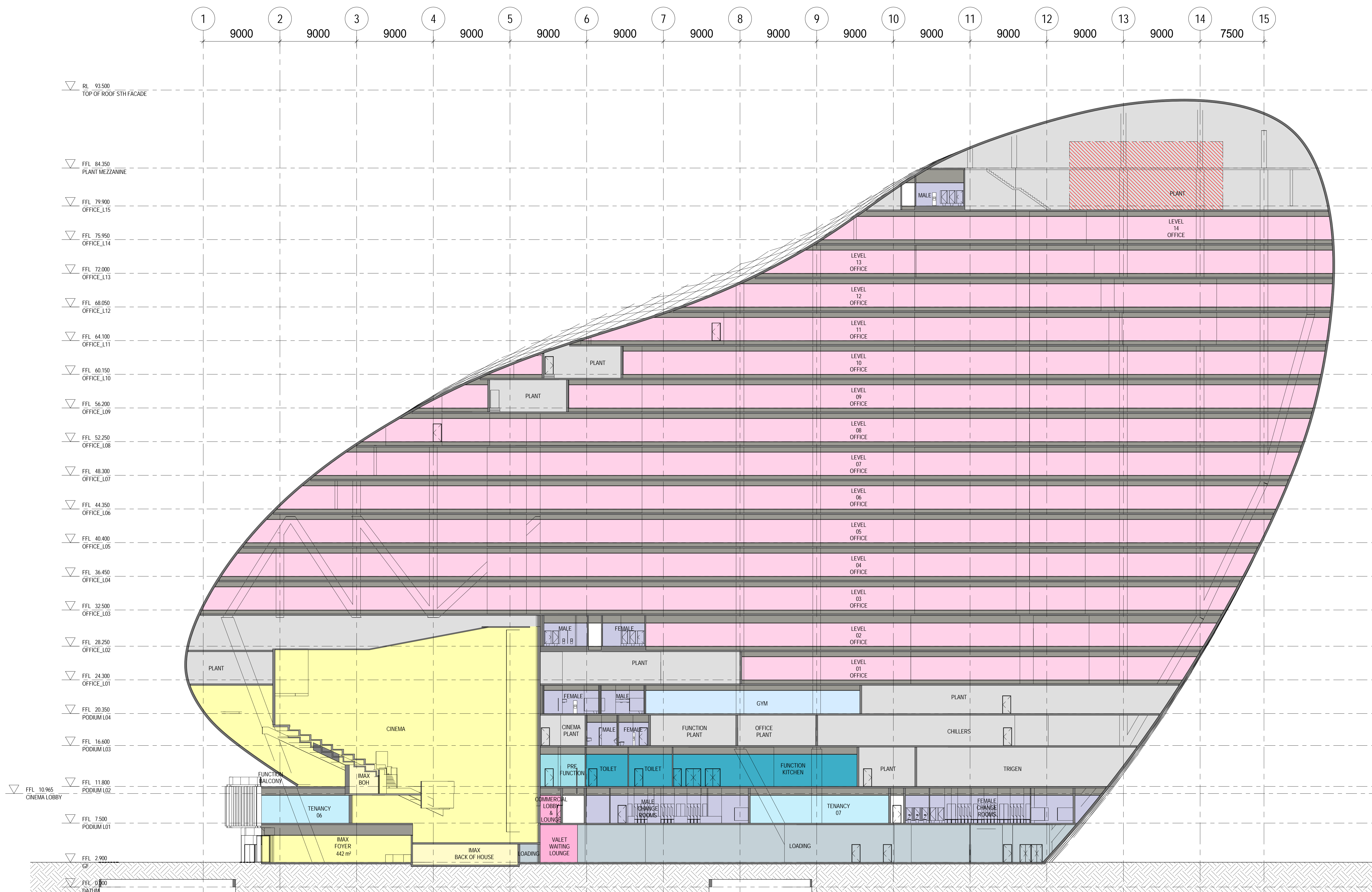
D SECTION 1:200
