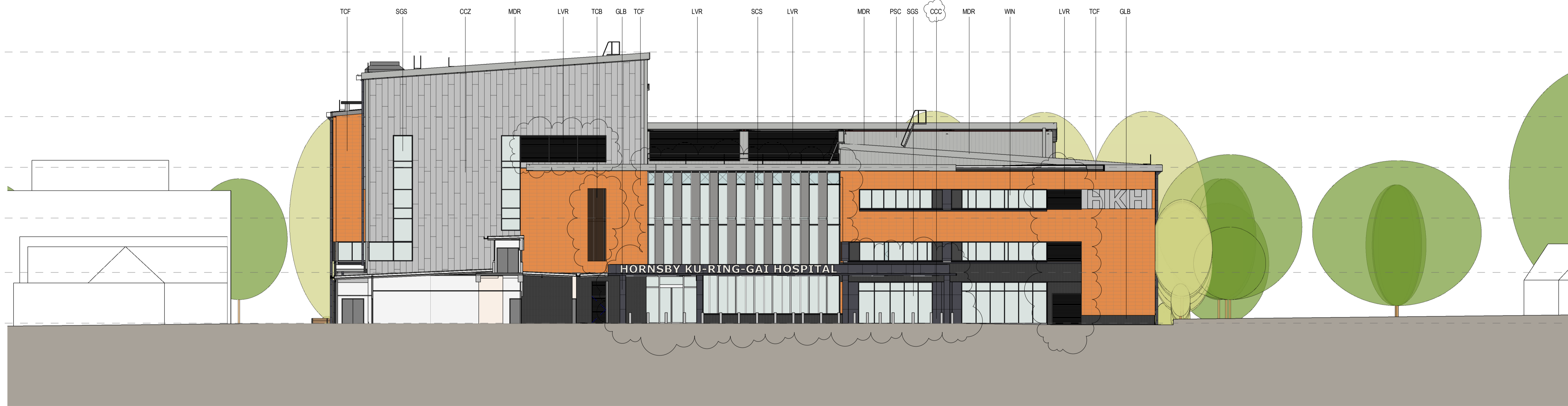
2 WEST ELEVATION B-B 1:200
