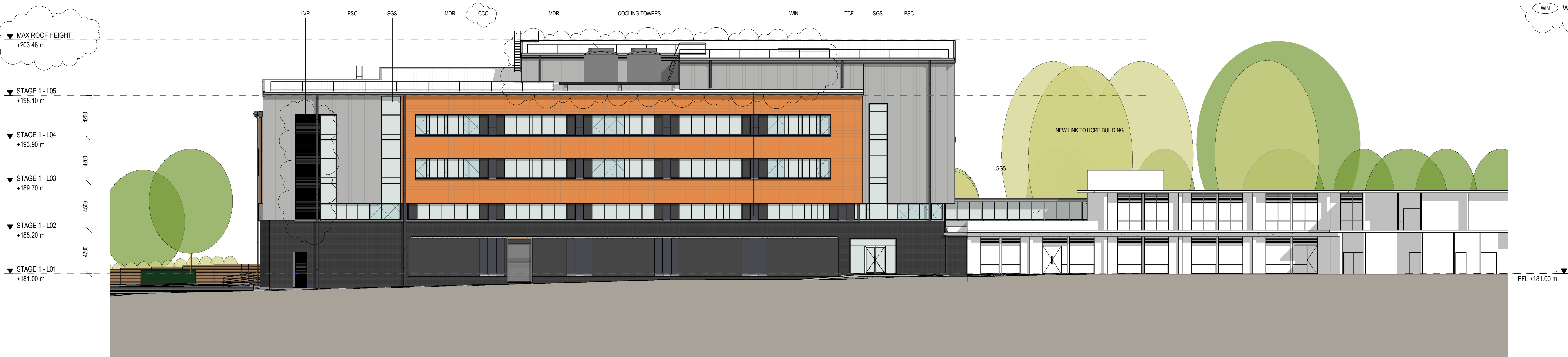
2 NORTH ELEVATION D-D 1:200
