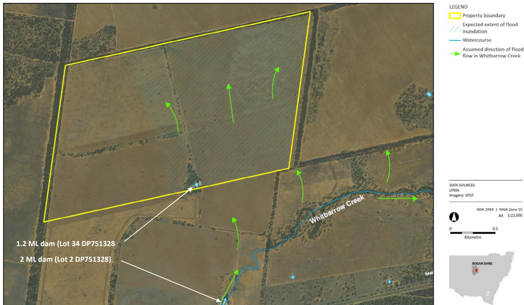
Figure 6-2 Inundation zones at the solar plant site.
