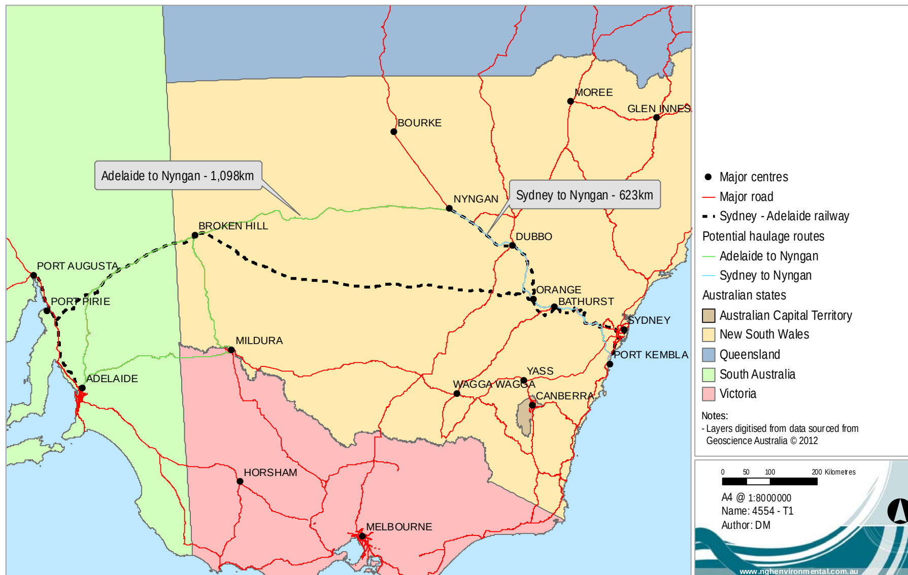
Figure 7-4 Road haulage route options.
