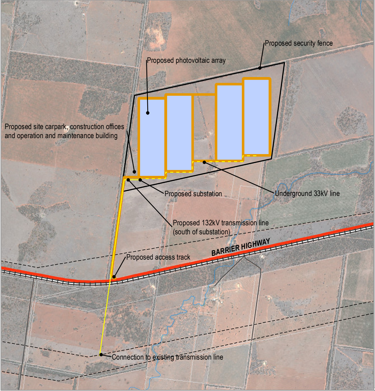
SITE LAYOUT
