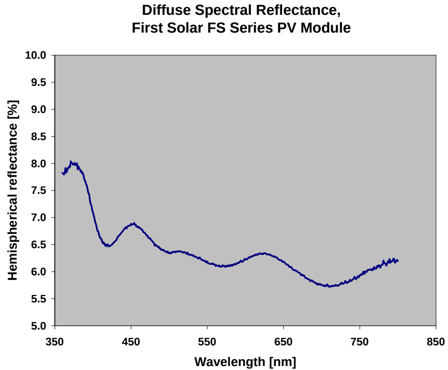
Figure 2. Diffuse spectral reflectance, as measured with a spectrophotometer with an integrating sphere attachment.
