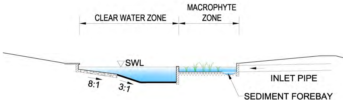
PLATE 6.3 TYPICAL SECTION THROUGH A WET POND
