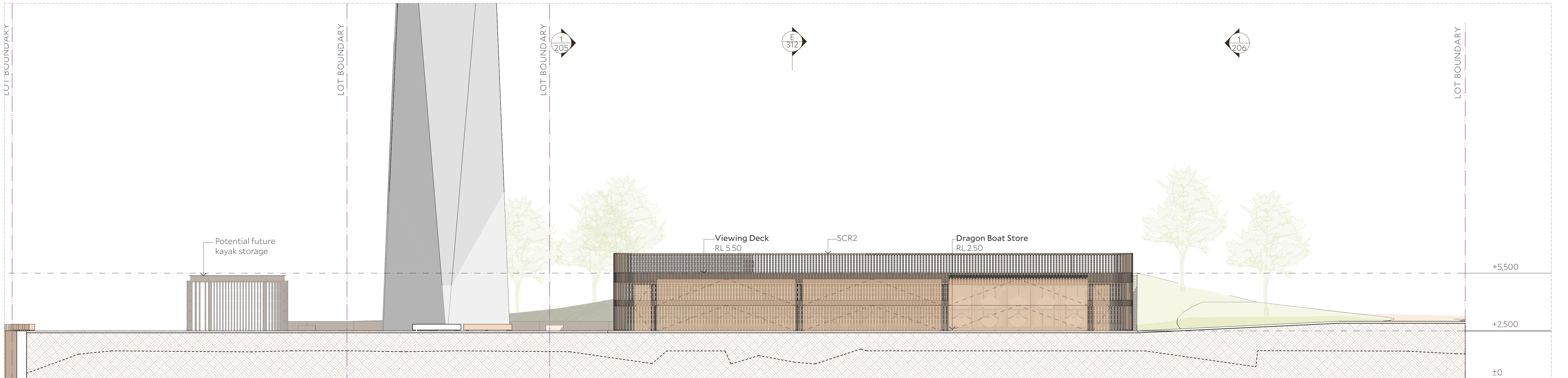
2 South Facade 1:100
