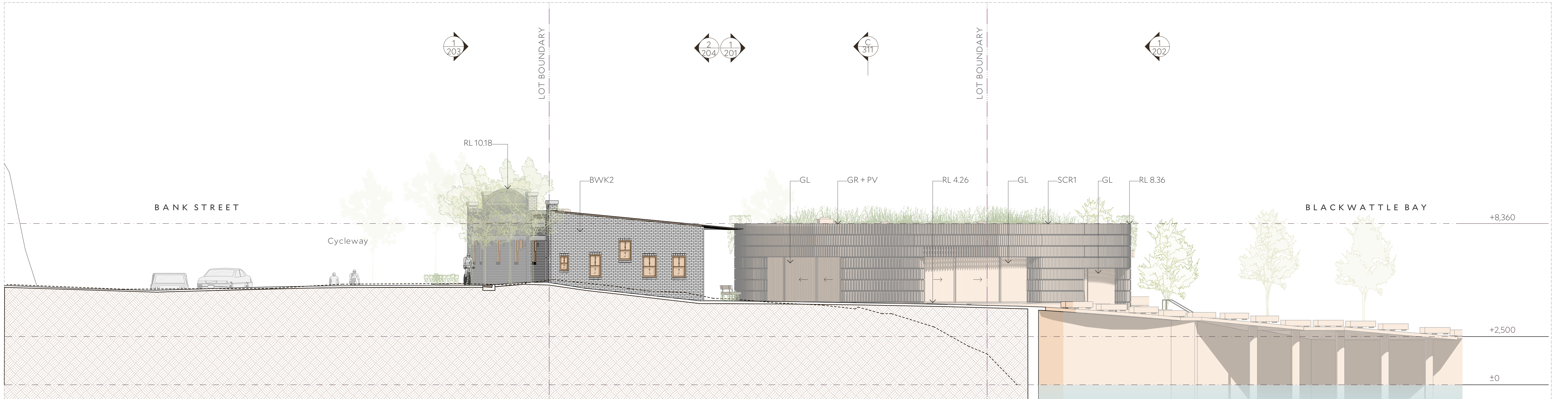
1 West Facade 1:100
