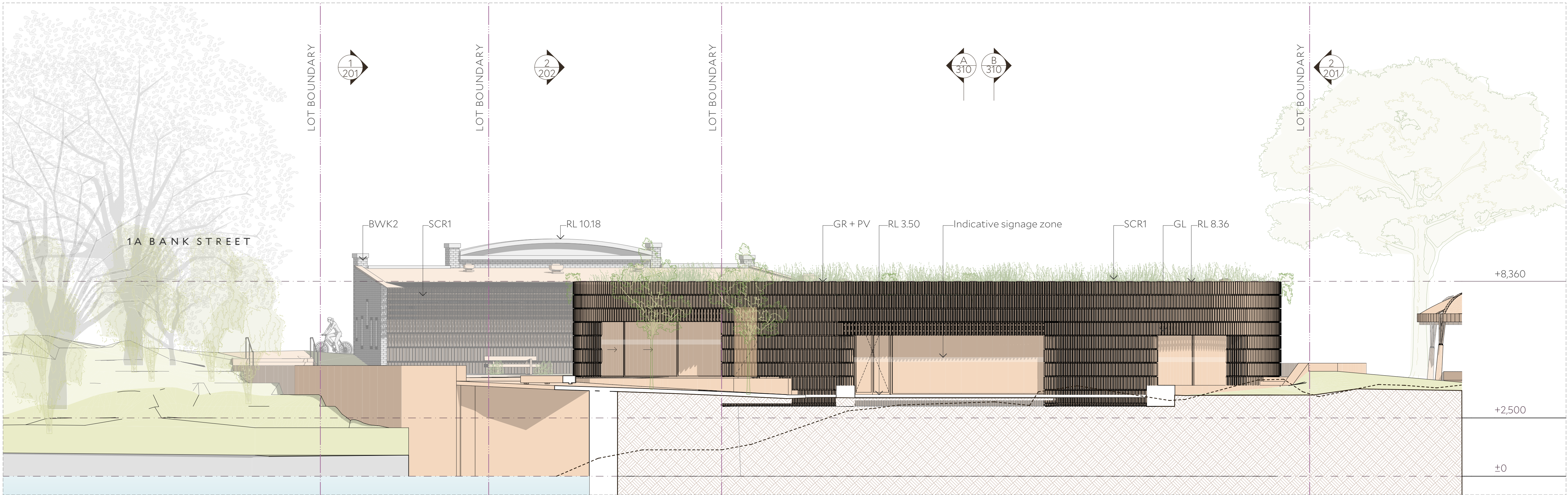
1 Blackwattle Bay (South) Facade 1:100
