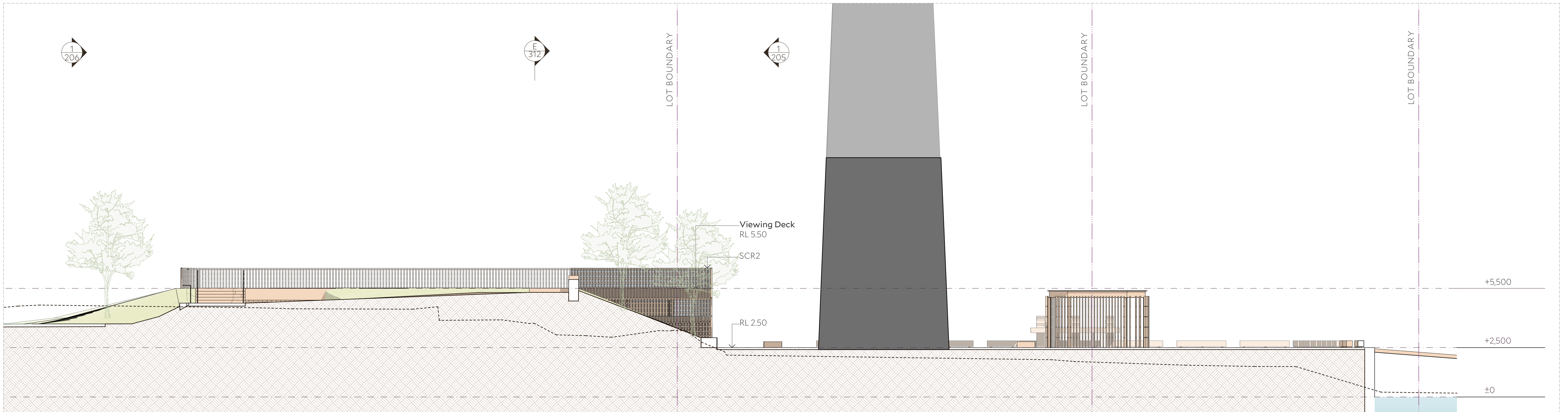
2 Buried (North) Facade 1:100
