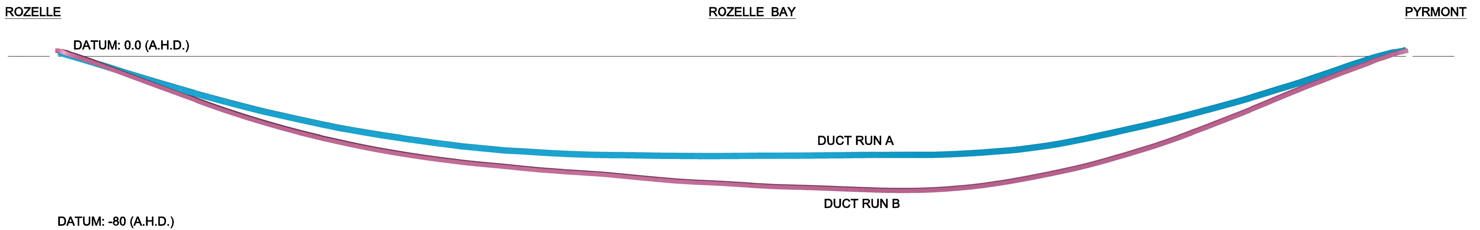
LONGSECTION A-A SUBMARINE BORE - DUCT RUNS A & B - VERTICAL TOLERANCE
