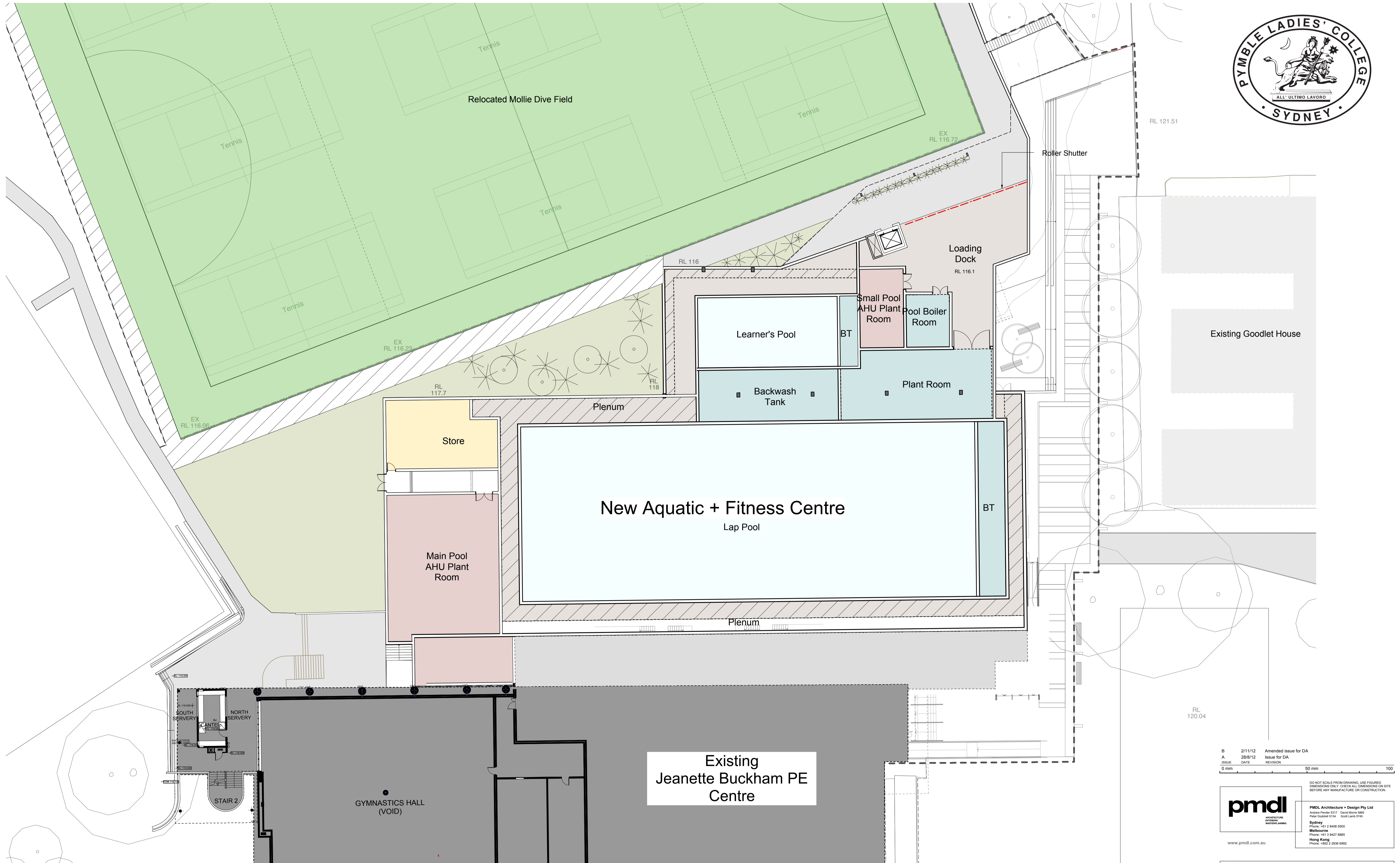
01 LOWER GROUND FLOOR PLAN Aquatic + Fitness Centre Scale 1:200
