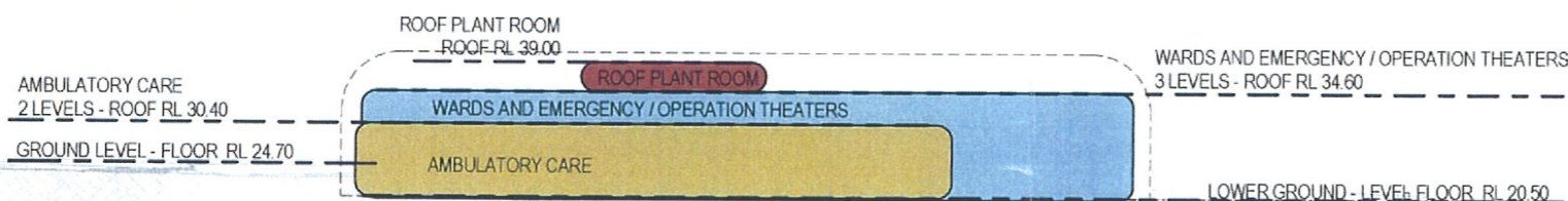
3 SK_103 1:500 PLANNING ELEVATION SOUTH
