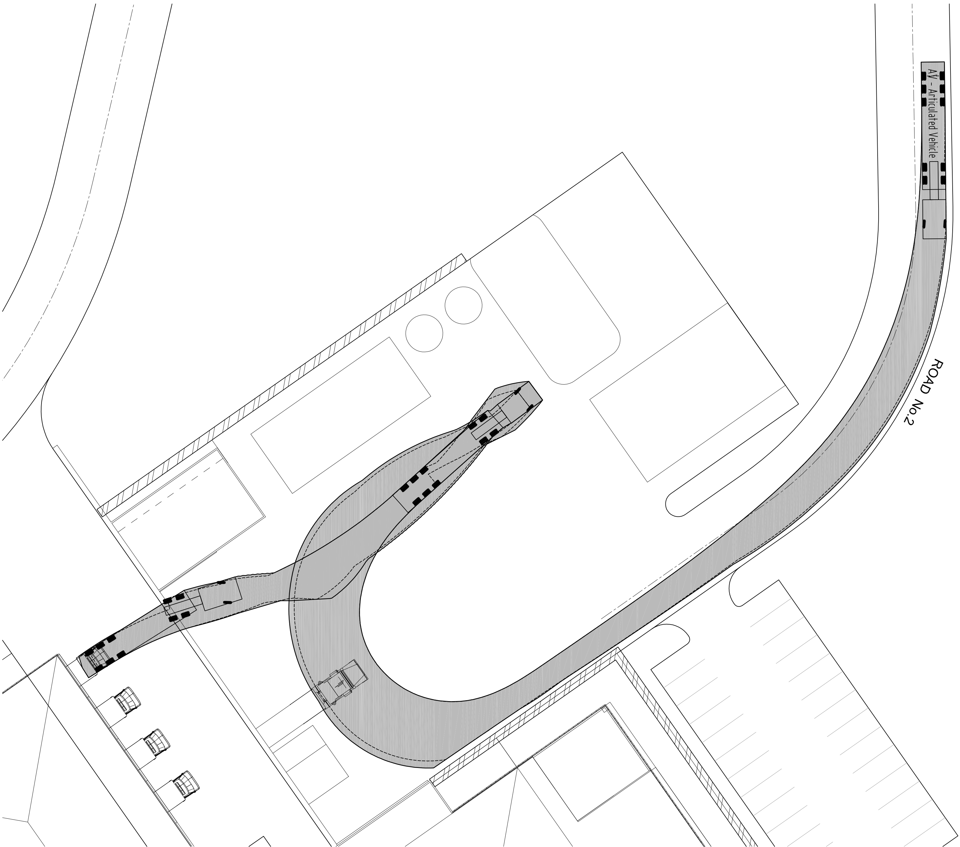
TURNING MOVEMENT - LOADING DOCK (19.0m ARTICULATED VEHICLE)
