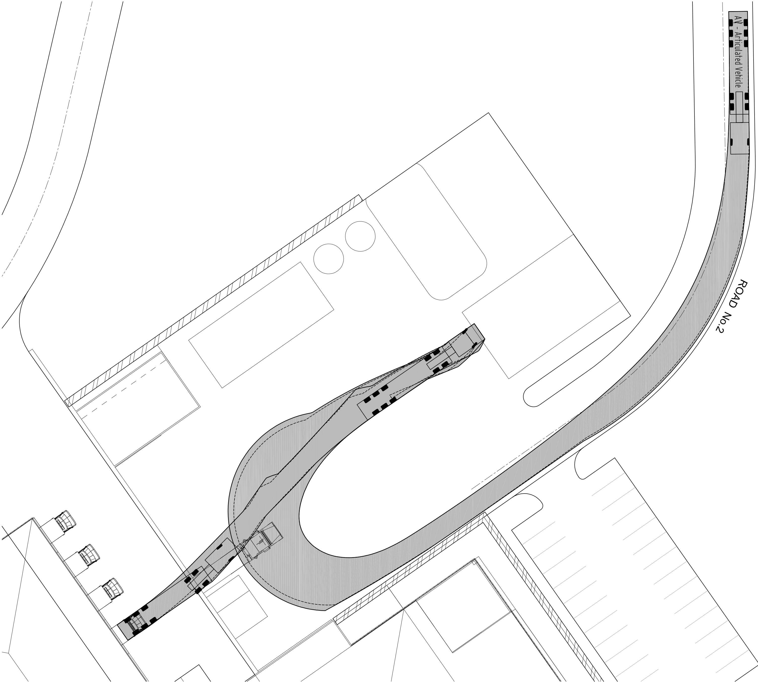
TURNING MOVEMENT - LOADING DOCK (19.0m ARTICULATED VEHICLE)
