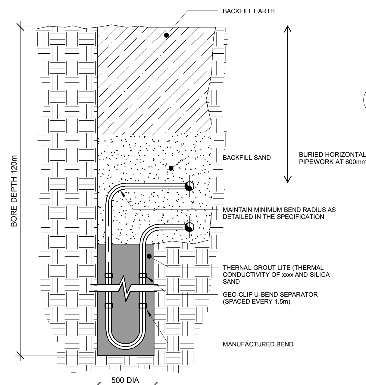
3 TYPICAL VERTICAL HEAT EXCHANGER DETAIL 1:20
