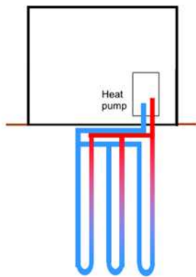
Fig 4: Closed Loop Borehole – Vertical Array
