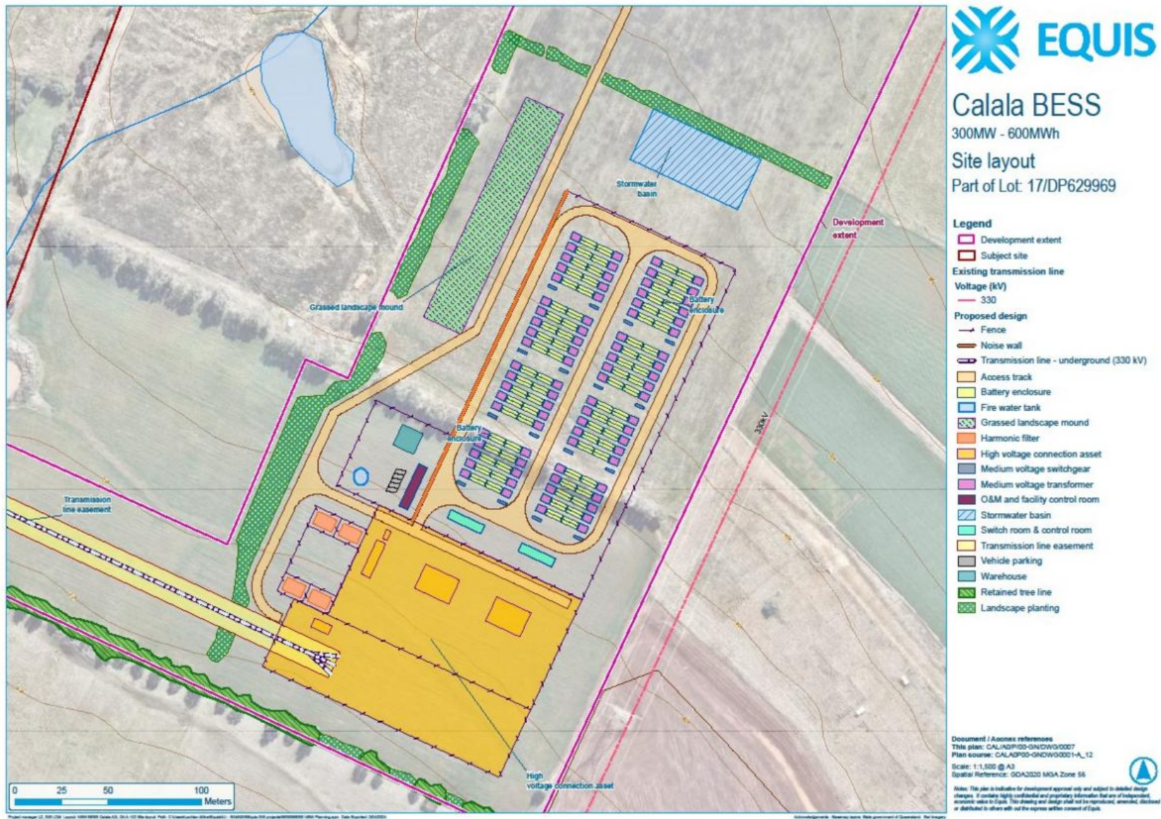
Figure 1.2 Site layout
