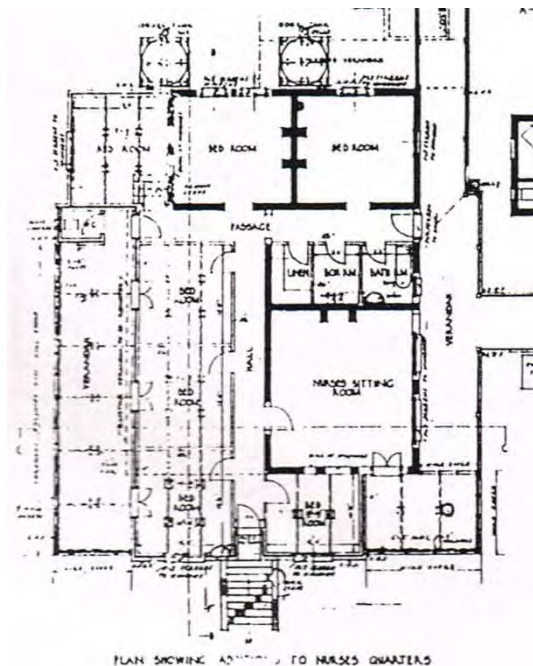
Figure 27 Plan of 1926 additions to the old 1868 hospital building to create a new nurses' residence. – Dubbo Base Hospital Archive
