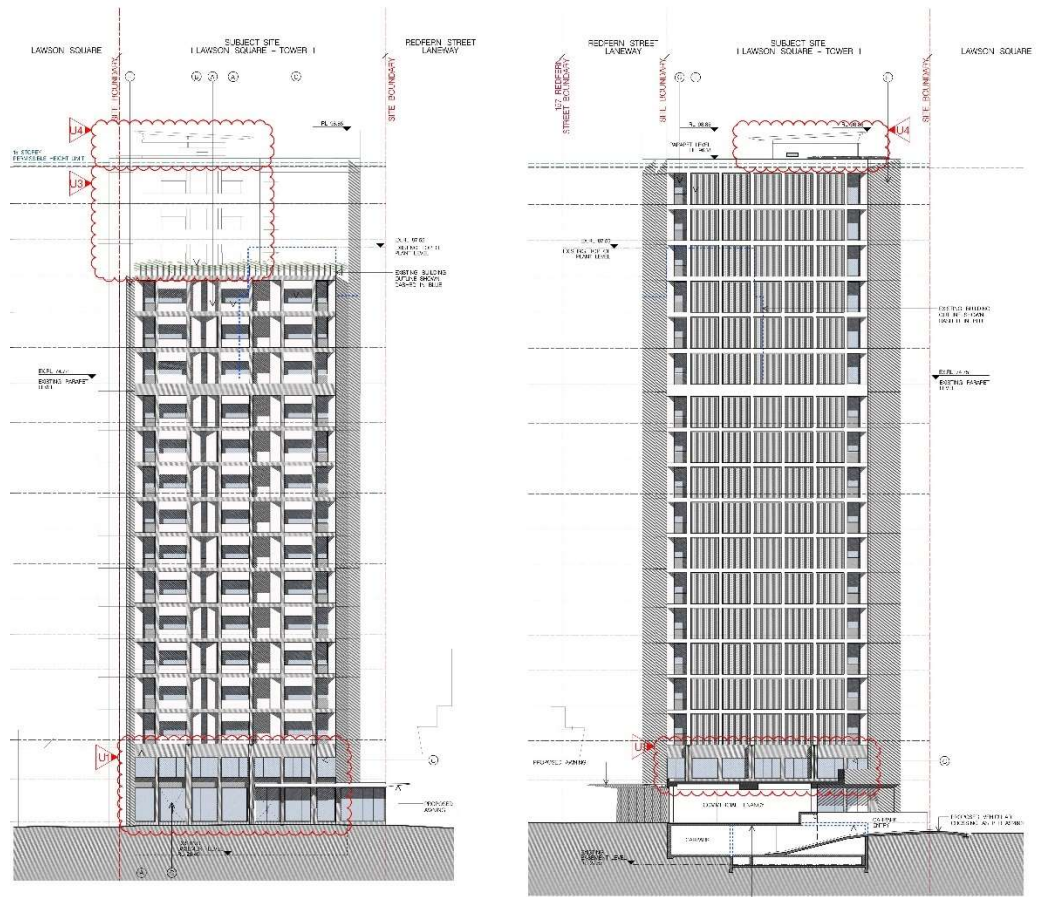
Figure (iv). East Elevation + West Elevation – Tower 1
