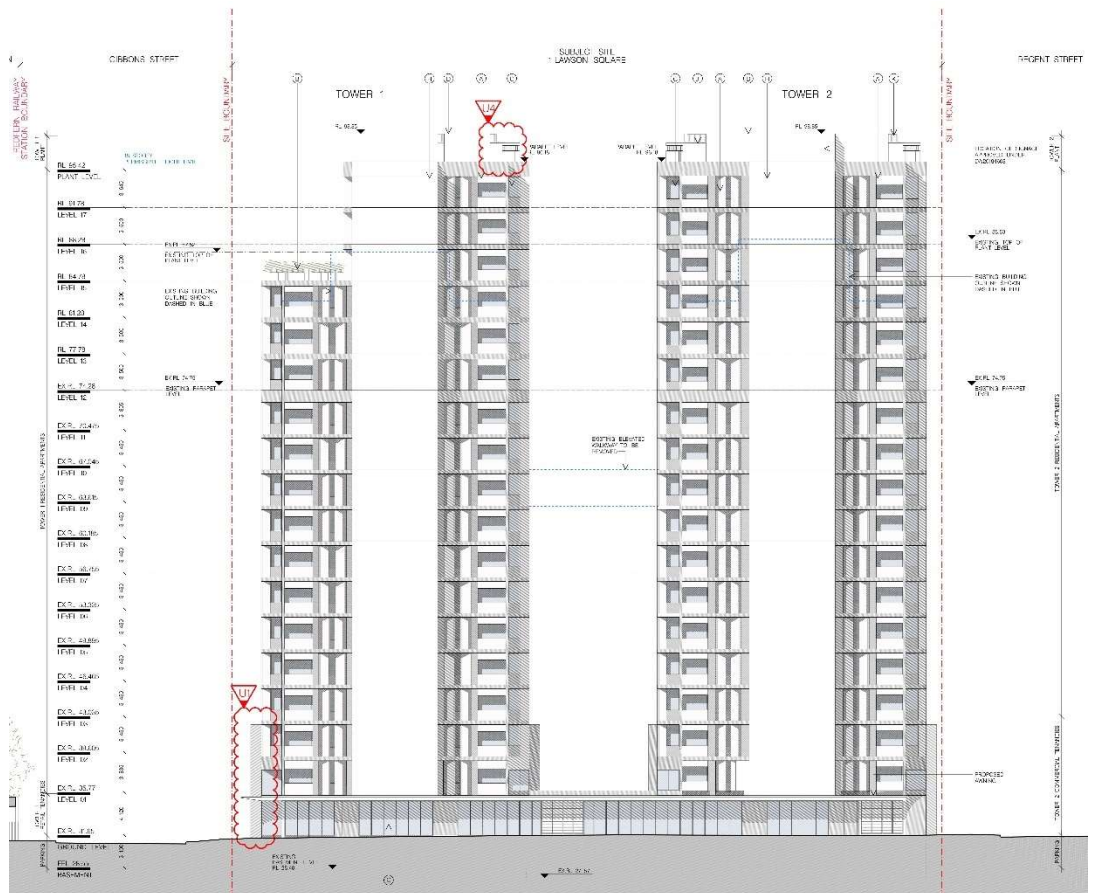
Figure (v). South Elevation
