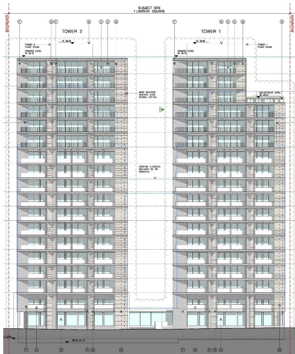
Figure (ii). North Elevation
