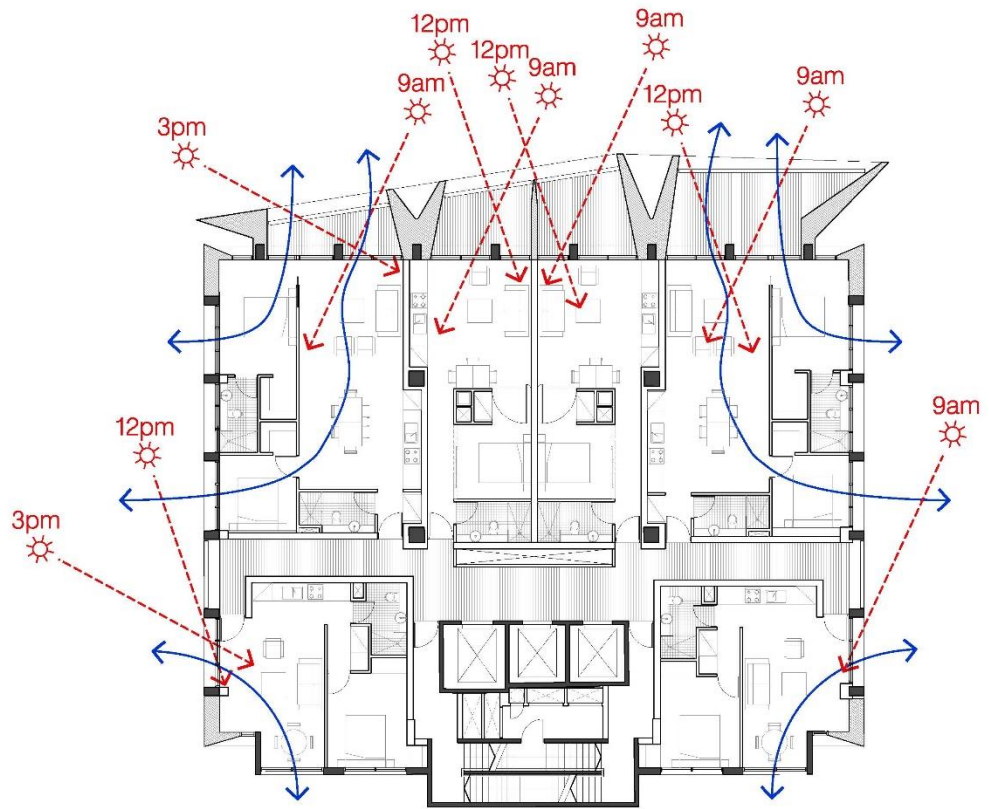
Figure (vii). Solar Access and Ventilation for June 21 – Tower 1
