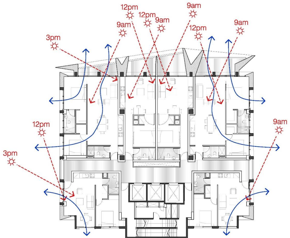
Figure (viii). Solar Access and Ventilation for June 21 – Tower 2
