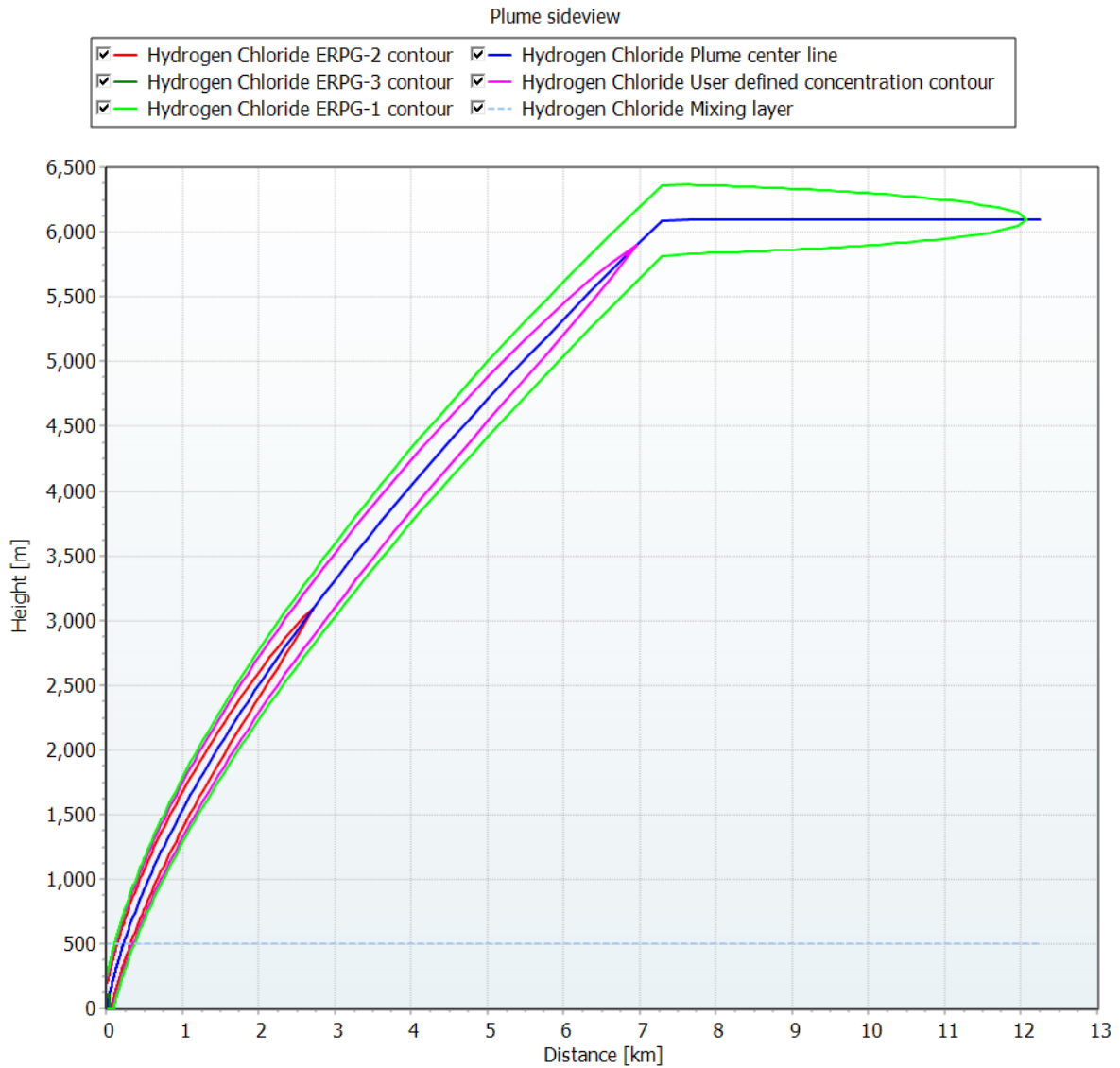
Appendix Figure B-13: Hydrogen Chloride Downwind Plume Dispersion
