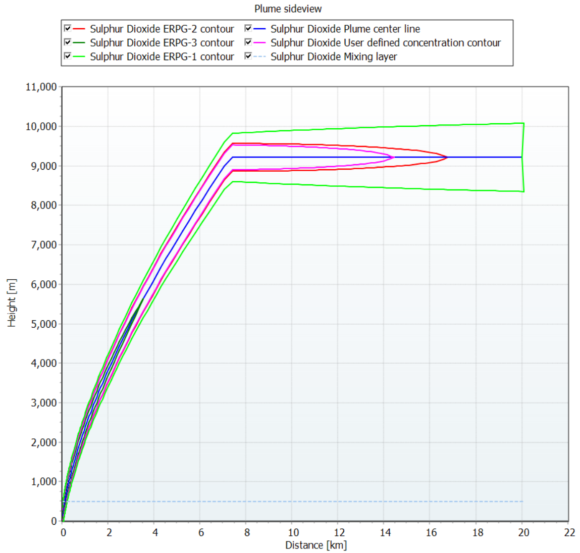
Appendix Figure B-12: Sulphur Dioxide Downwind Plume Dispersion
