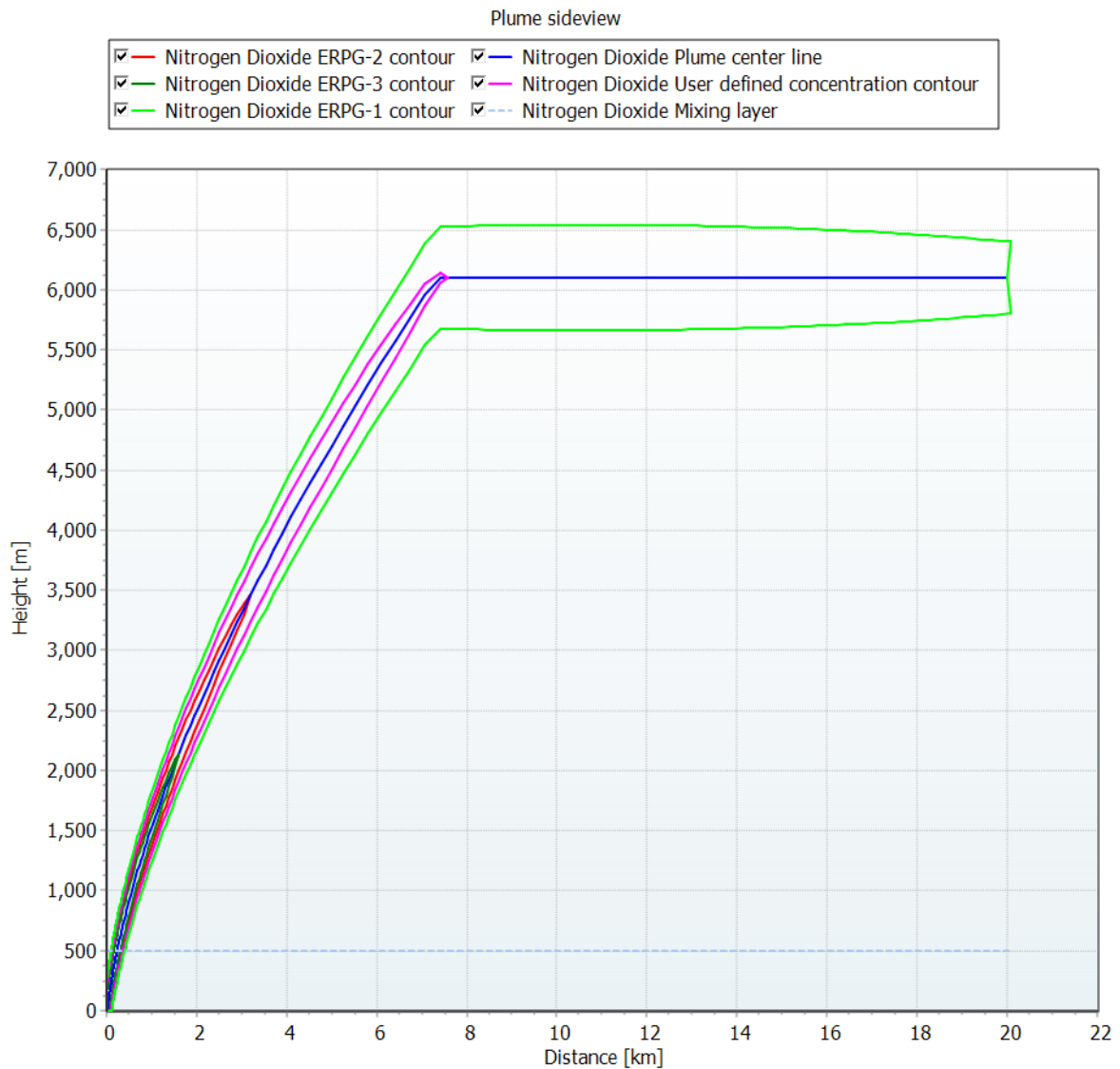
Appendix Figure B-11: Nitrogen Dioxide Downwind Plume Dispersion
