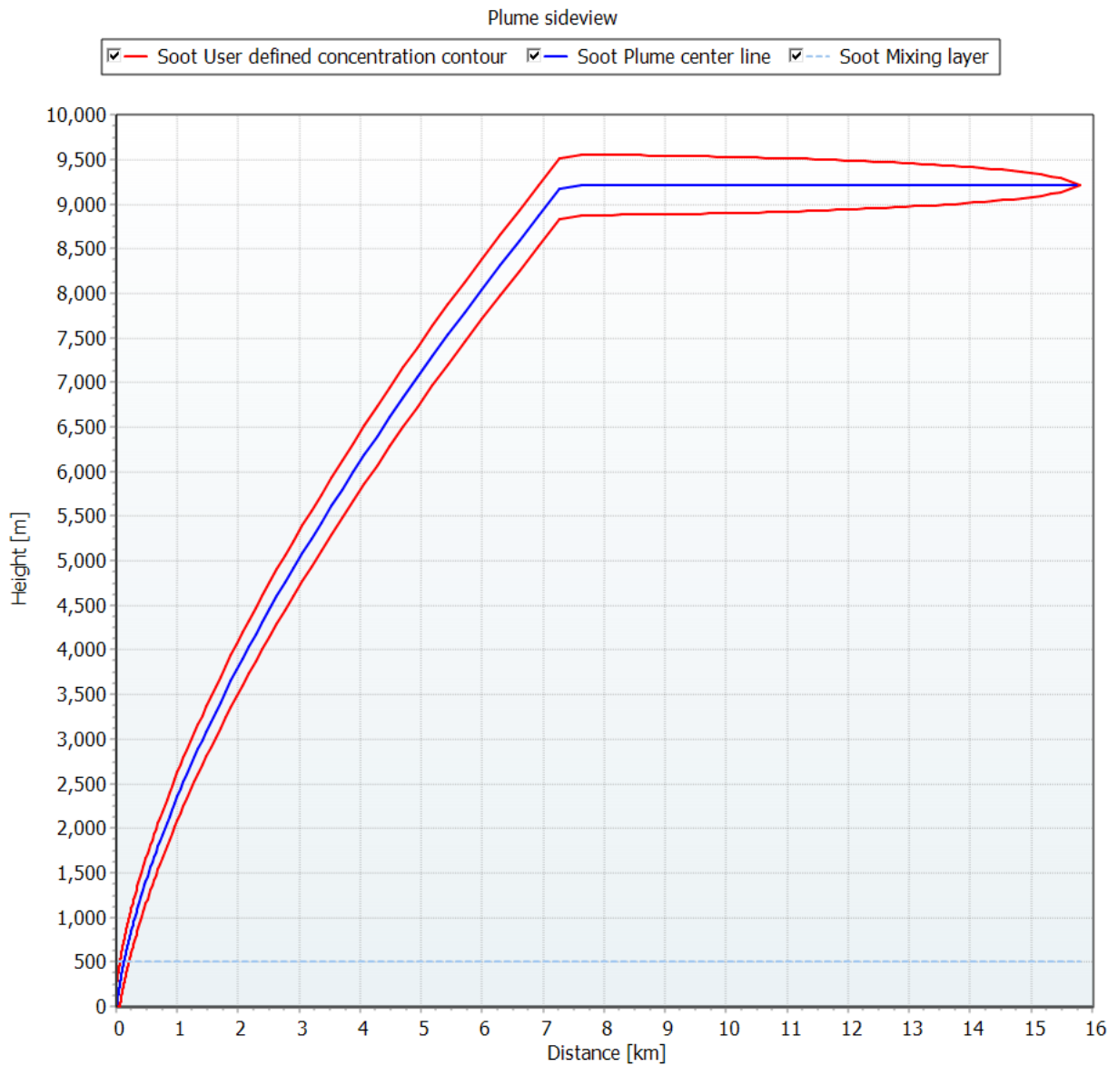
Appendix Figure B-14: Soot (Carbon) Downwind Plume Dispersion
