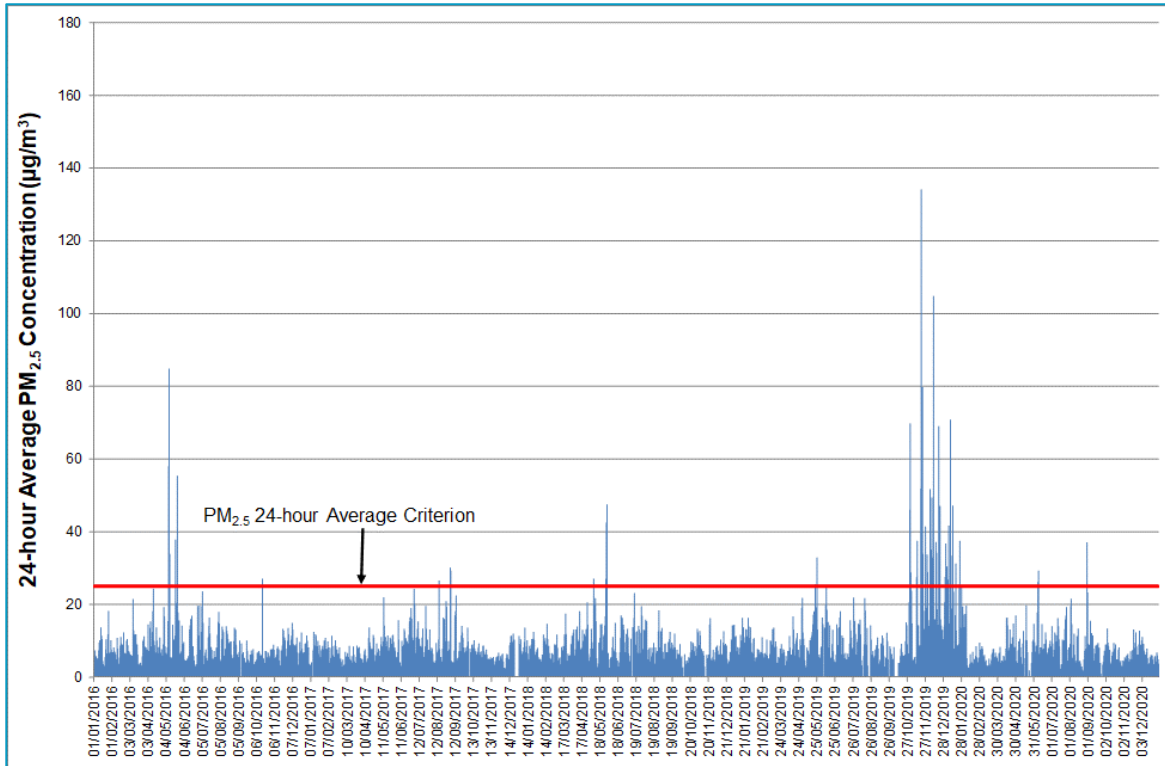
Figure 6 24-hour PM 2.5 Concentrations Recorded by Prospect AQMS (2016-2020)
