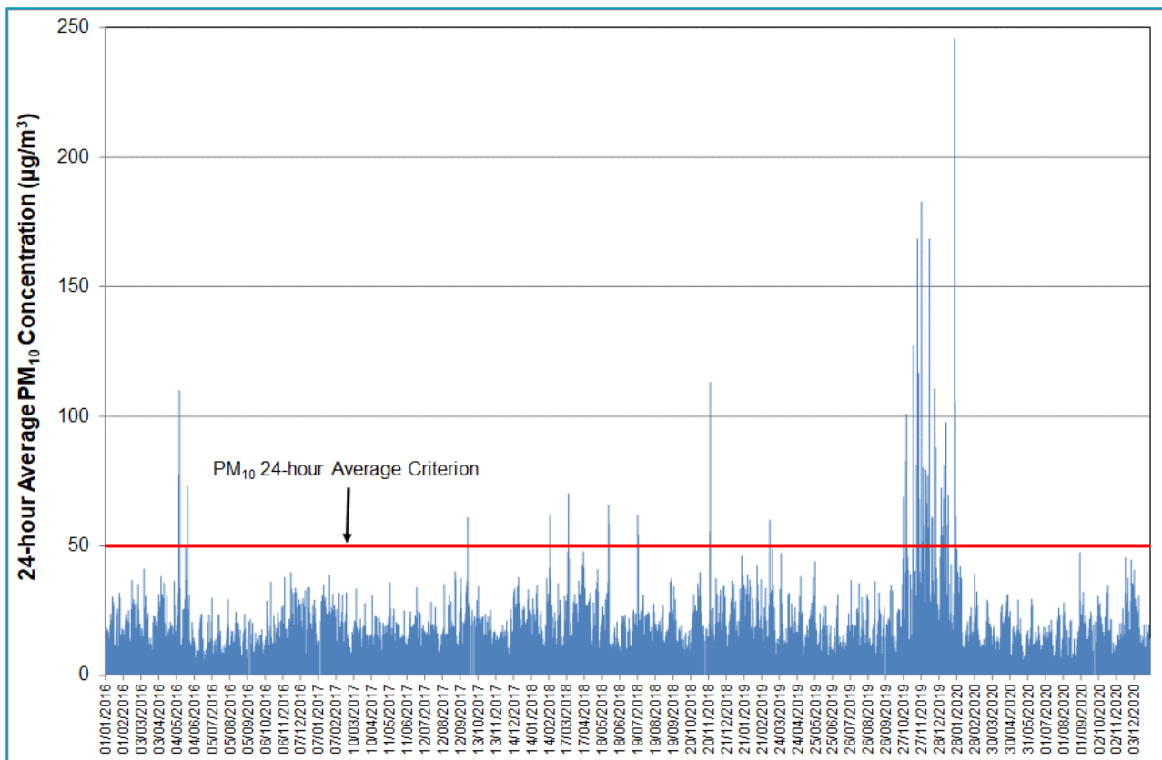
Figure 5 24-hour PM 10 Concentrations Recorded by Prospect AQMS (2016-2020)
