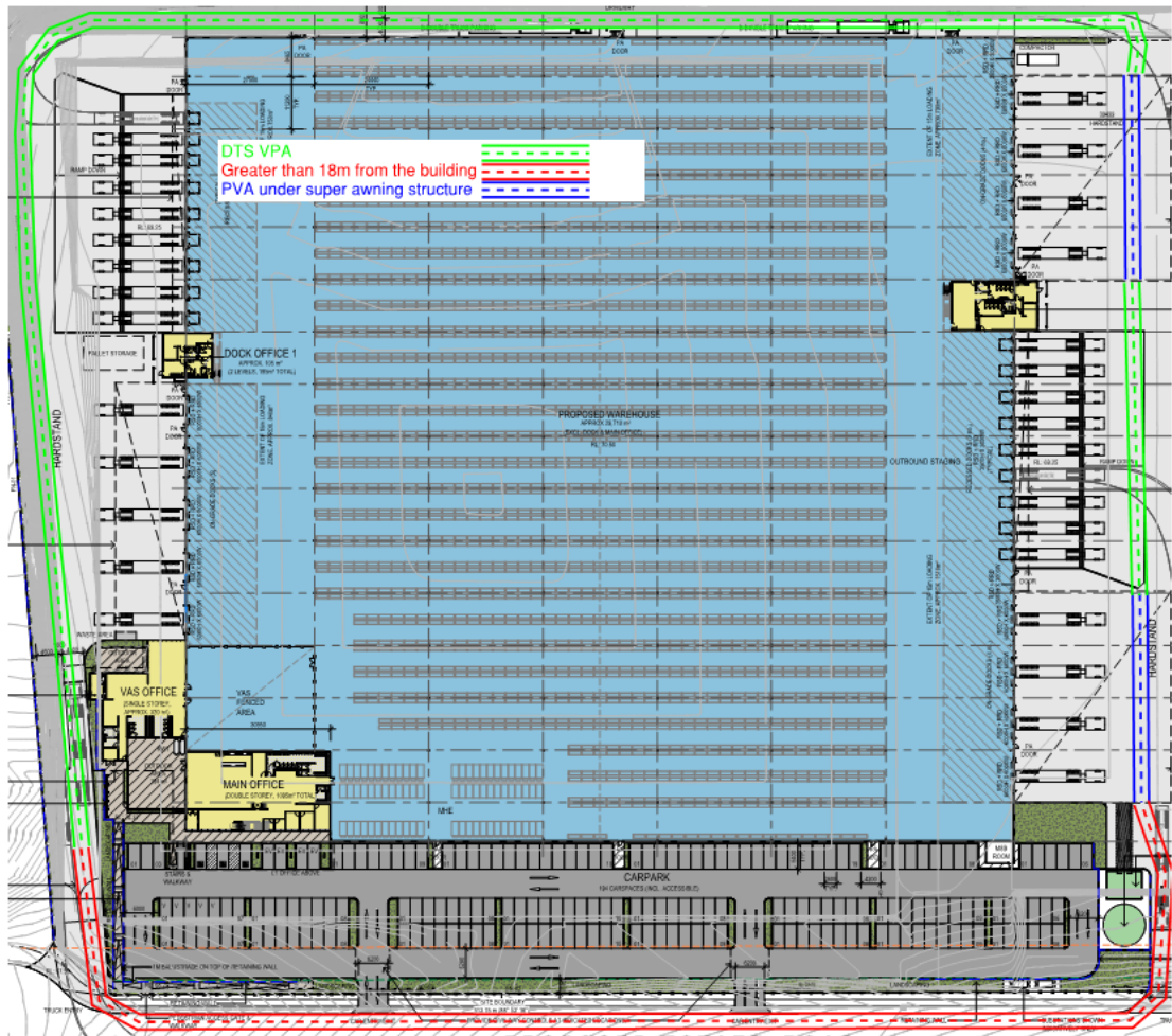
Figure 1 – Perimeter Vehicular Access per BCA C2.4.
