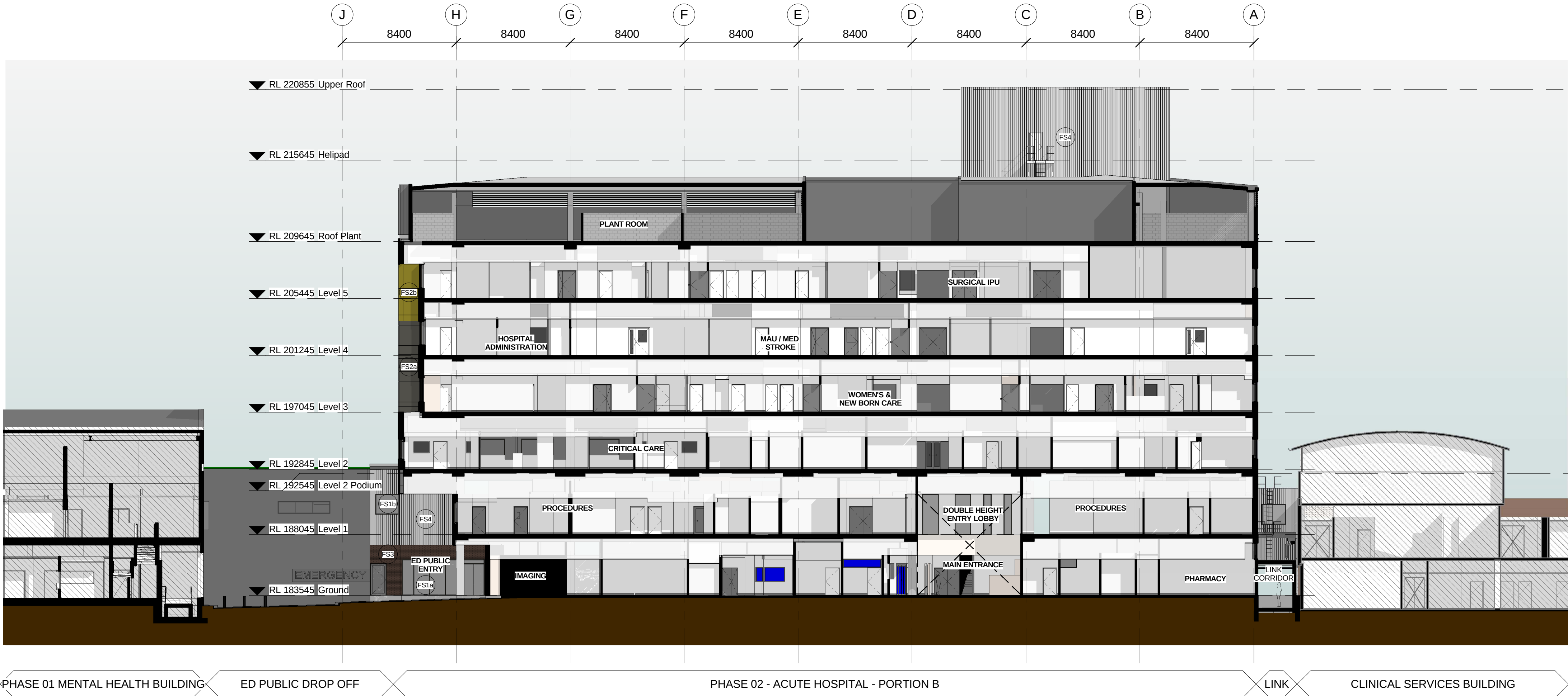
C ACUTE HOSPITAL OVERALL PRECINCT SECTION C
