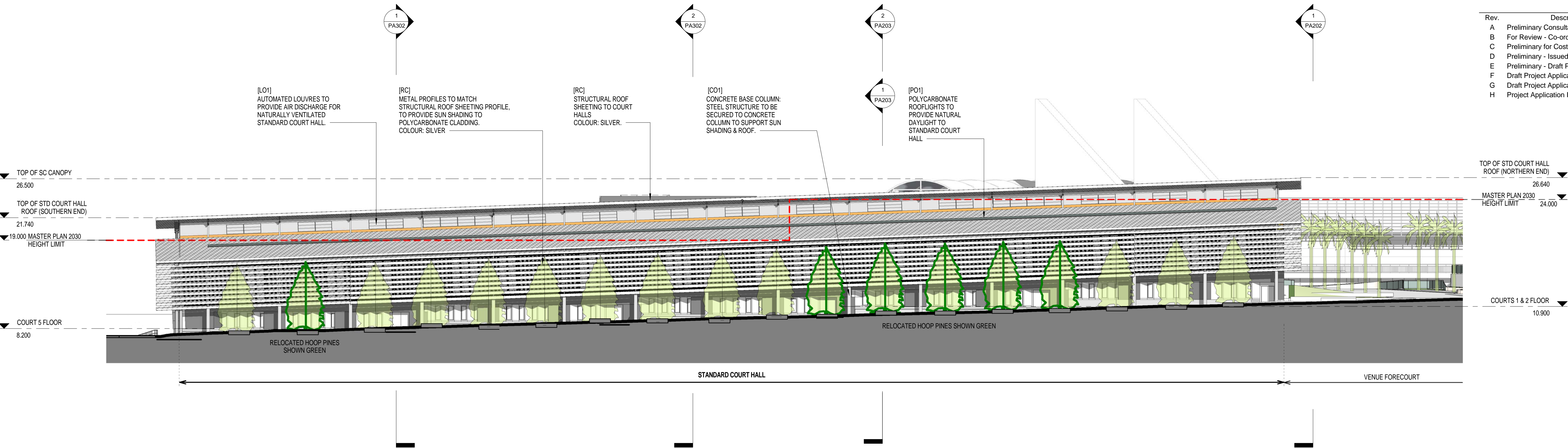
1 Olympic Boulevard Elevation 1:250
