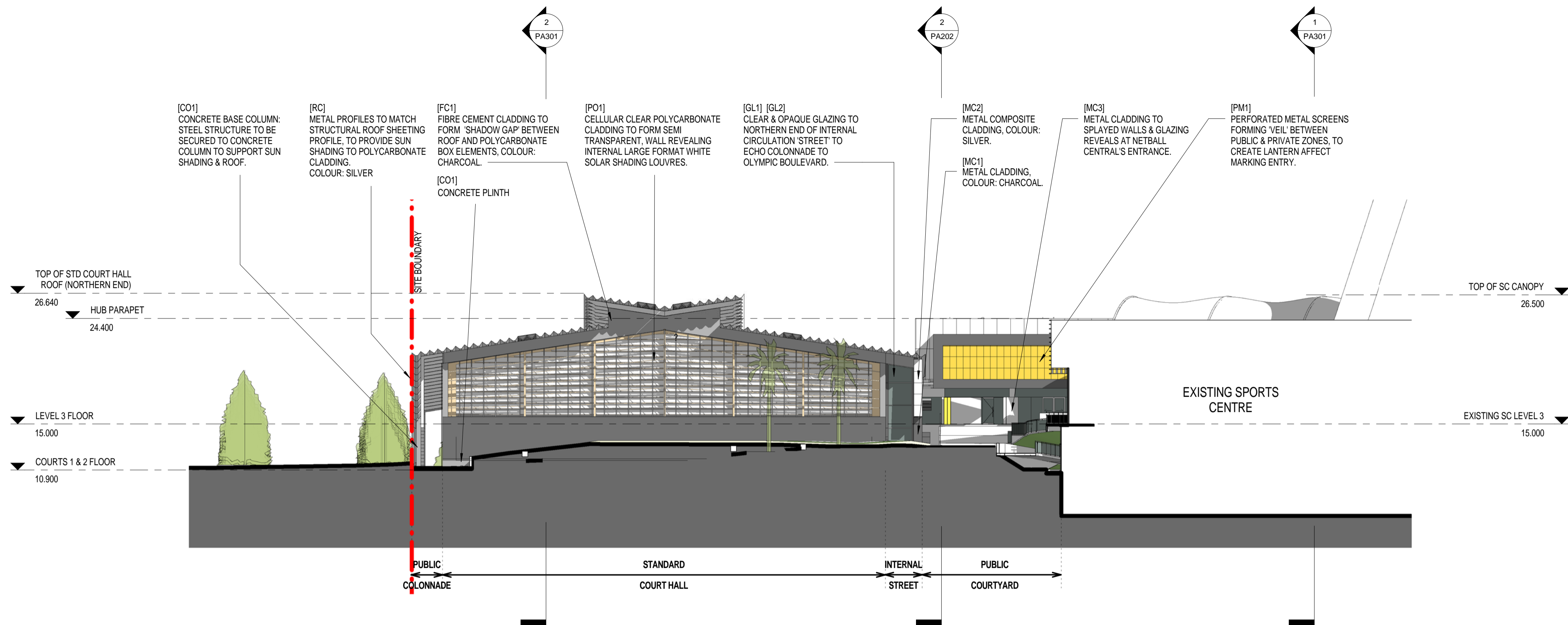
1 North Elevation 1:250
