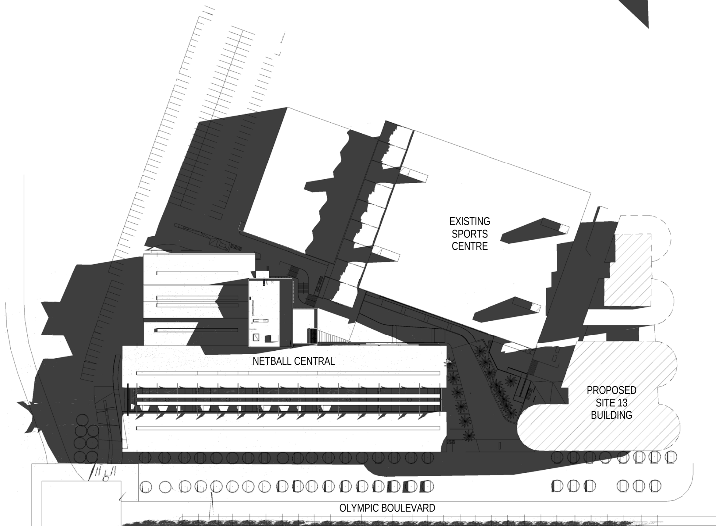
3 Shadow Diagram - 3pm June 21 1:1000
