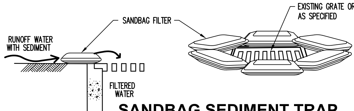
SANDBAG SEDIMENT TRAP NTS
