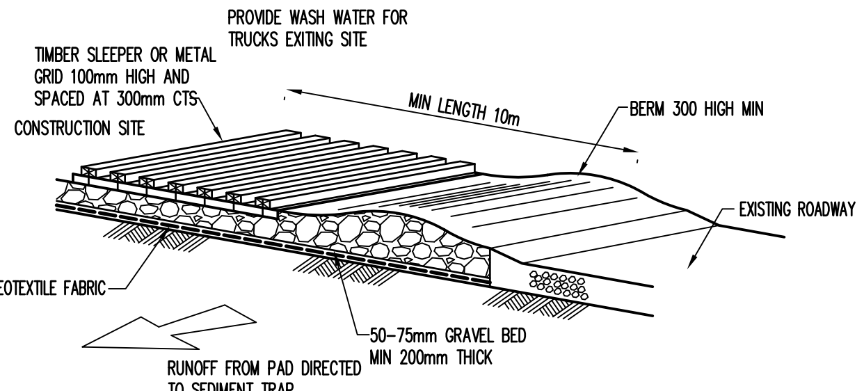
TEMPORARY CONSTRUCTION VEHICLE EXIT NTS
