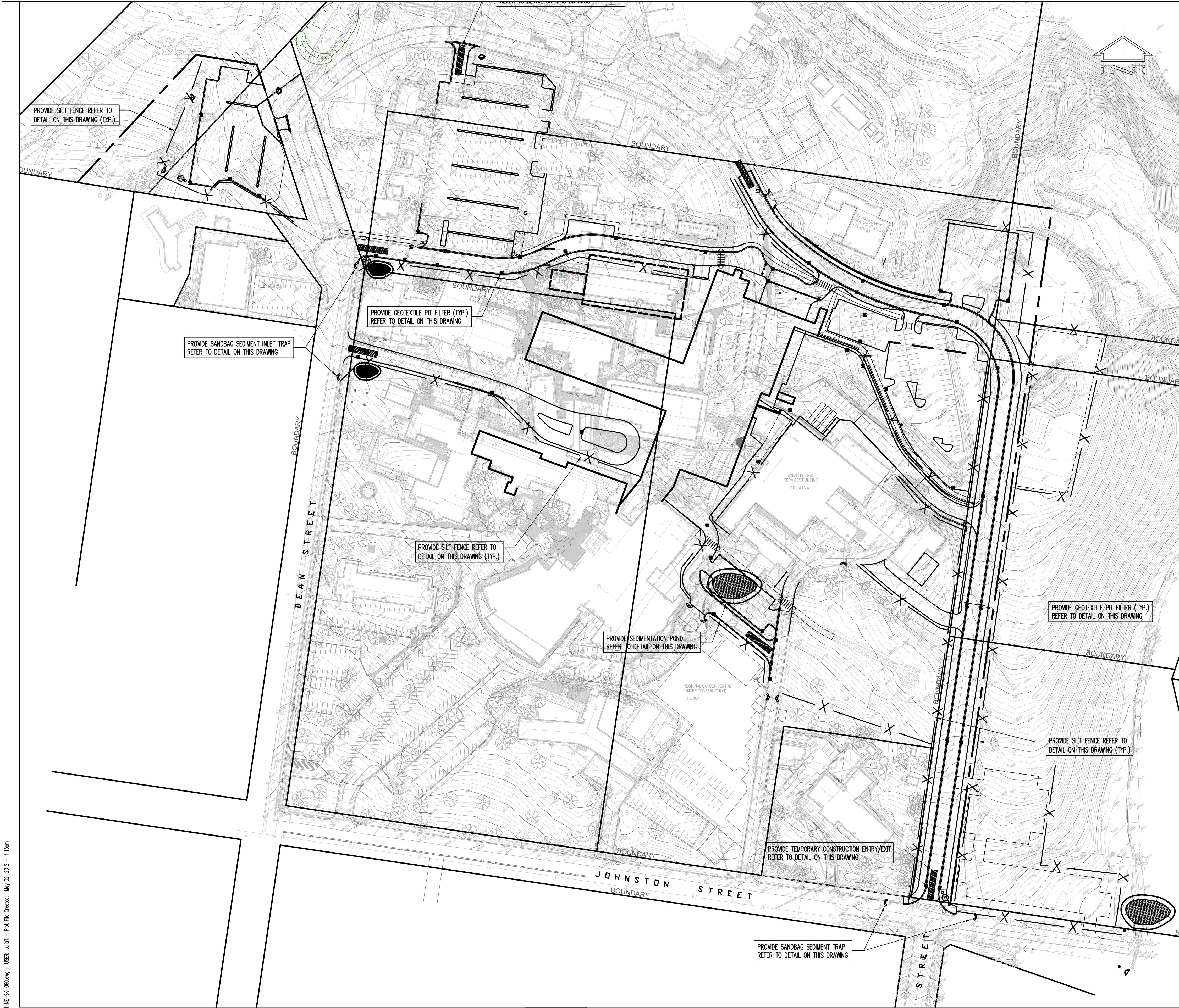
PLAN SCALE 1: 1000
