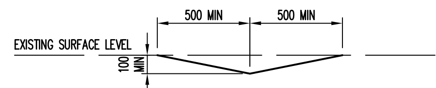
TYPICAL SECTION THROUGH CATCH DRAIN SCALE 1: 20
