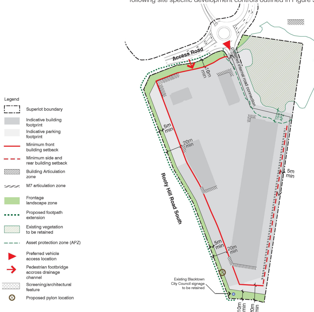
Figure 51: Development Control Plan - Lot 1 (not to scale)
