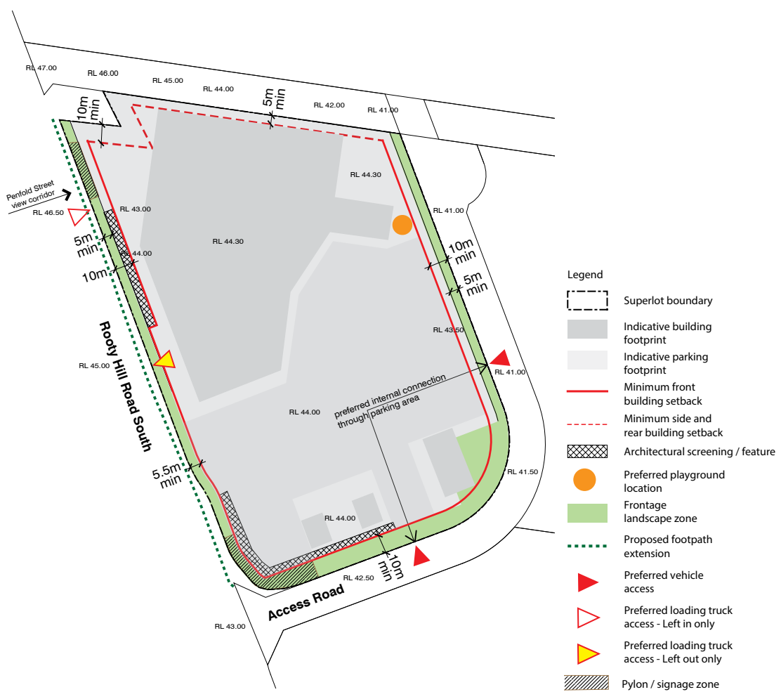
Figure 52: Development Control Plan - Lot 2 (not to scale)
