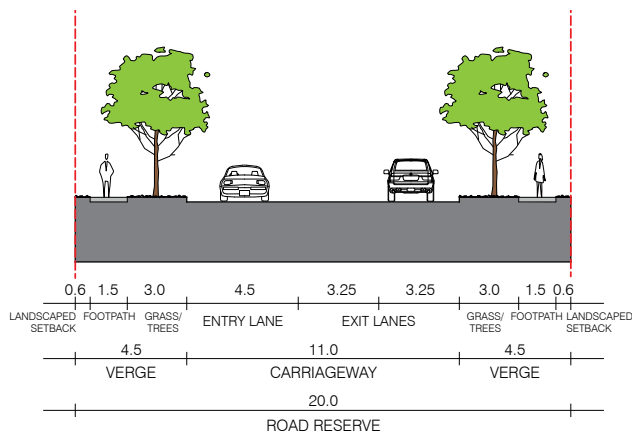
Figure 10: Street Section - Entry
