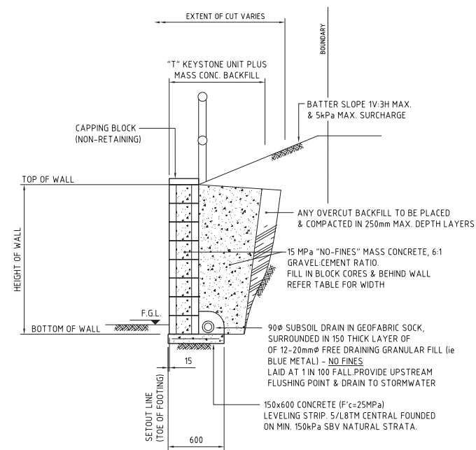
RETAINING WALL DETAIL IN CUT (‘NO-FINES’ MASS CONCRETE KEYSTONE WALL) SCALE 1:20
