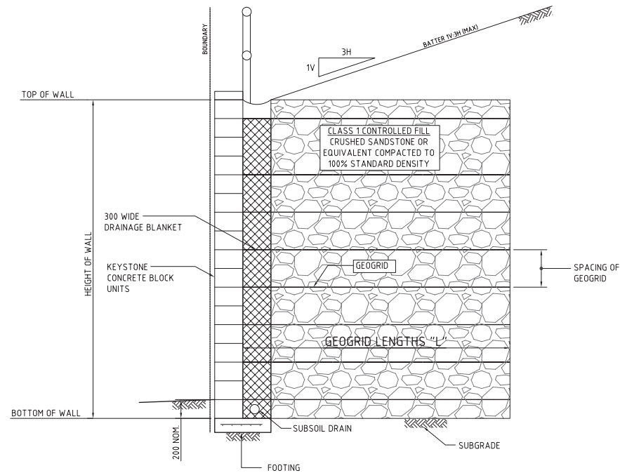
RETAINING WALL DETAIL IN FILL (REINFORCED EARTH WALL) SCALE 1:20
