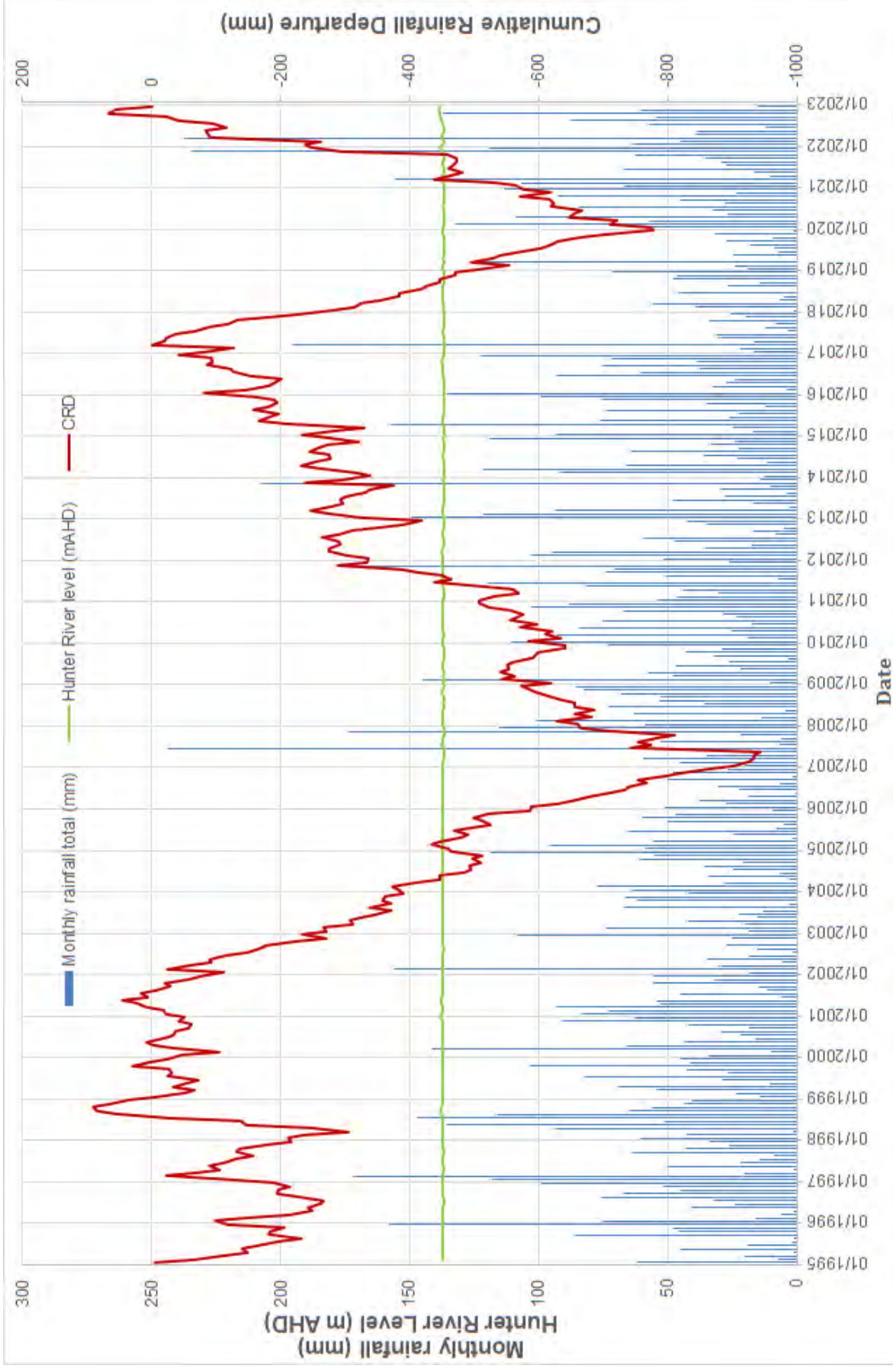
Figure 2.1 Cumulative rainfall departure (1995 to 2022) for Bengalla weather monitoring station
