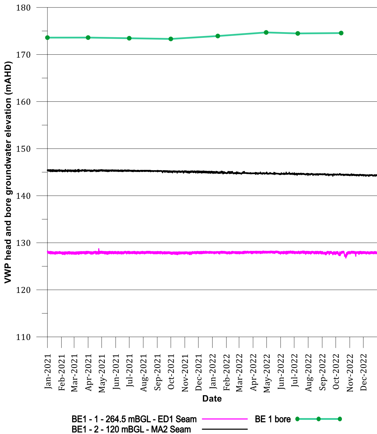
Figure 6.19 Northwest Permian VWP potentiometric heads – BE1
