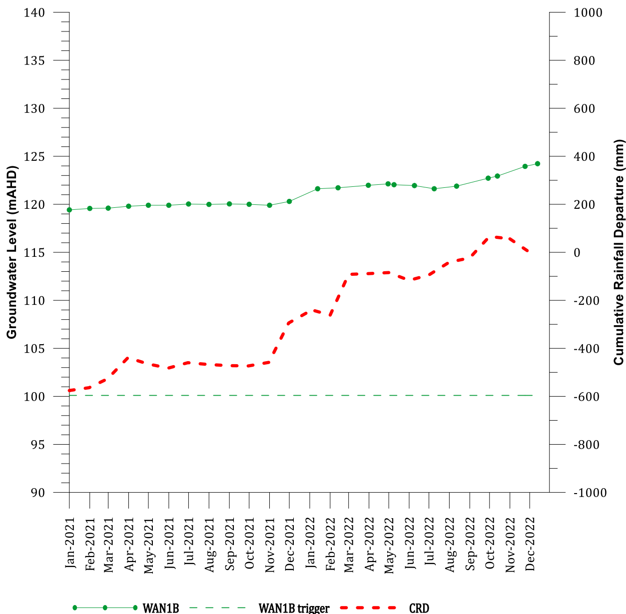
Figure 6.6 Hydrograph of shallow Permian monitoring bores
