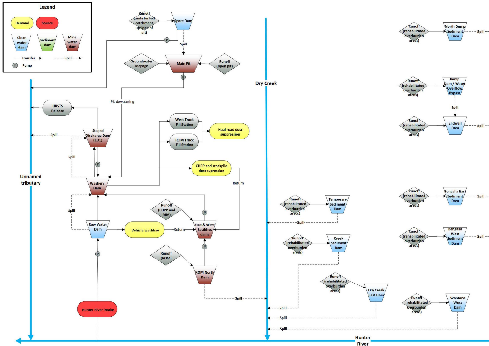
Figure 4-9 Bengalla proposed water management system schematic - Year 24
