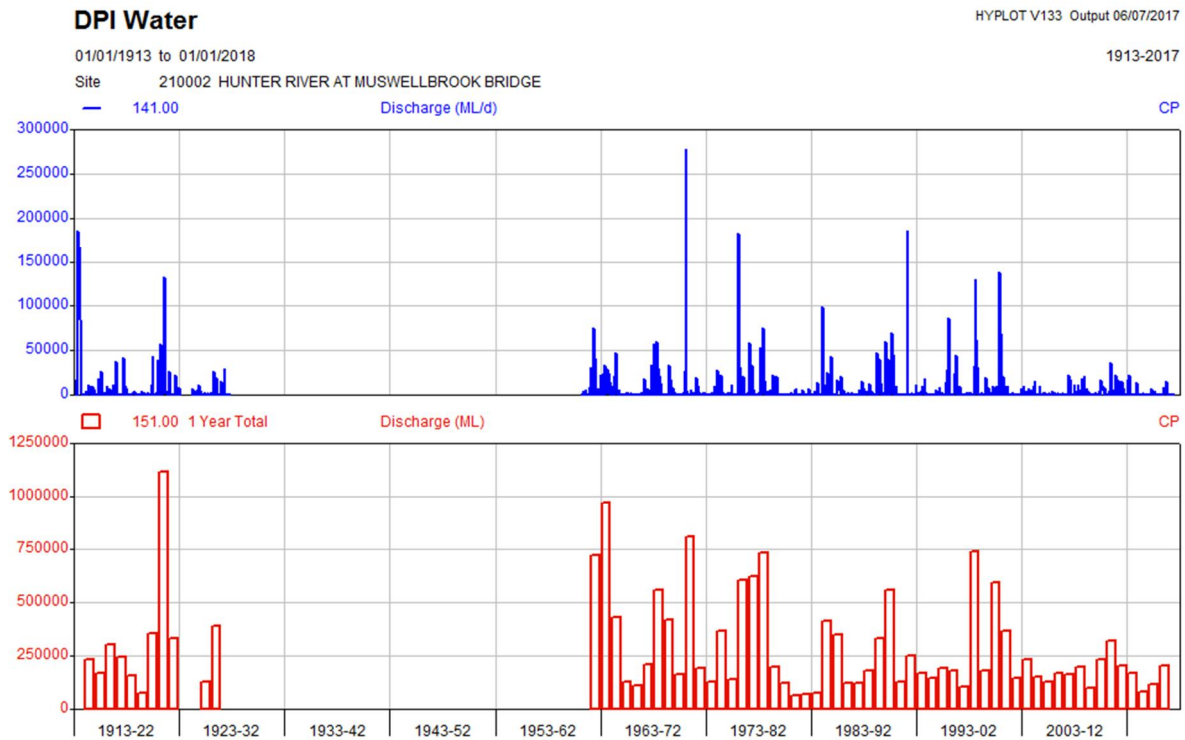
Figure 3.2 Streamflow timeseries for Hunter River at Muswellbrook Bridge (Station No 210002) for 1913 to 2017 (Source: DPI Water 'real-time data' website)
