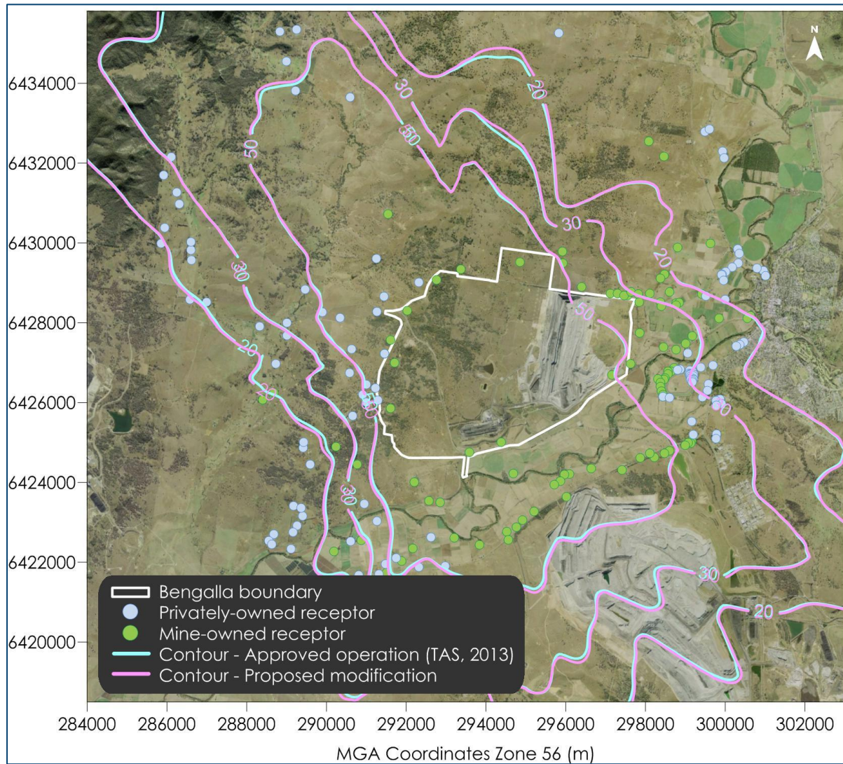
Figure 10: Comparison of predicted maximum incremental 24-hour average PM_{10} concentrations for proposed Modification as per AQIA (TAS, 2013) –Year 24 ( \mu g/m^3 )
