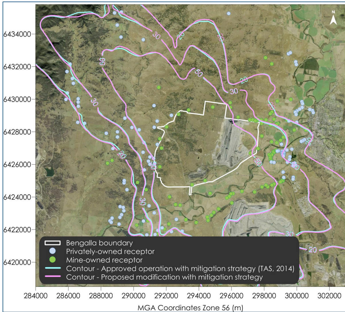
Figure 11: Comparison of predicted maximum incremental 24-hour average PM_{10} concentrations for proposed Modification including consideration of mitigation strategy (TAS, 2014) –Year 24 ( \mu g/m^3 )
