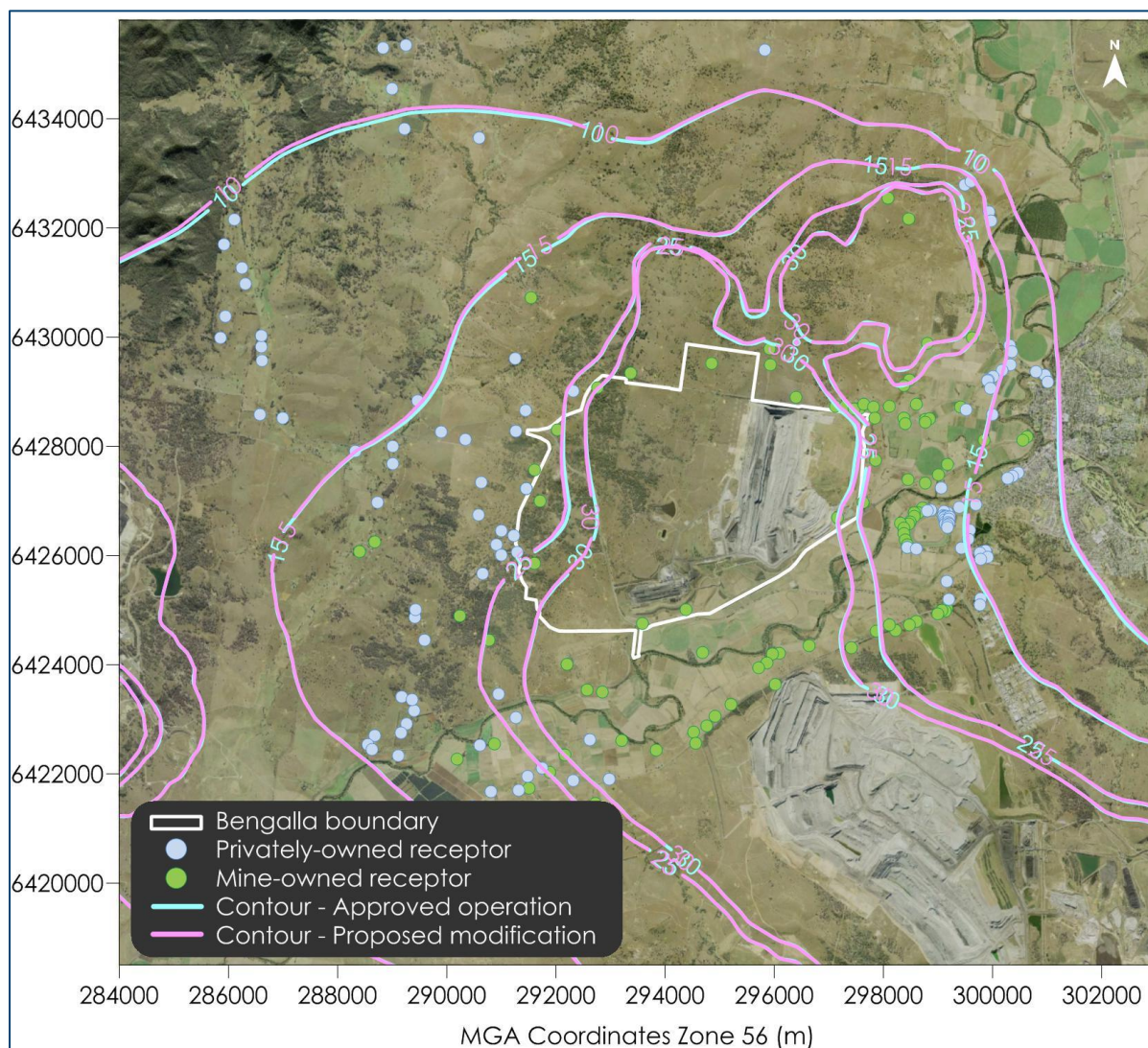
Figure 19: Comparison of cumulative predicted annual average PM 10 concentrations (Bengalla and other sources) – Year 4 (µg/m 3 )
