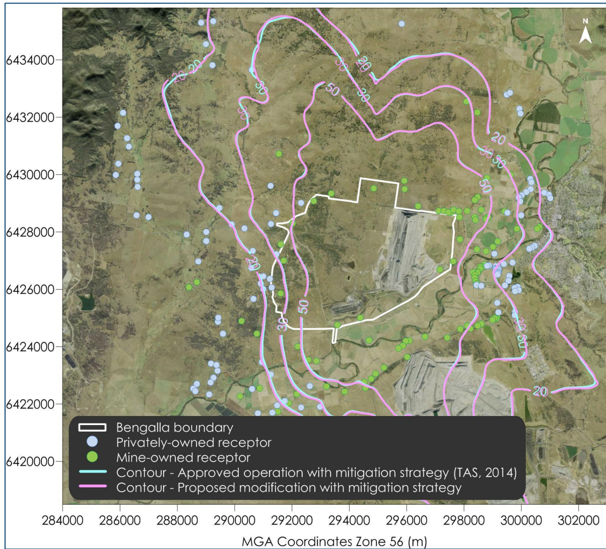
Figure 4: Comparison of predicted maximum incremental 24-hour average PM_{10} concentrations for proposed Modification including consideration of mitigation strategy (TAS, 2014) –Year 4 ( \mu g/m^3 )
