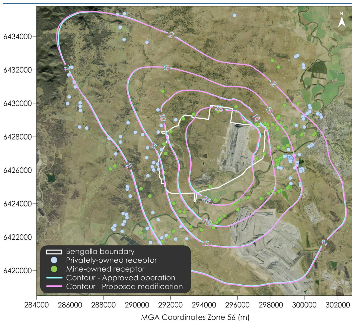
Figure 5: Comparison of predicted incremental annual average PM_{10} concentrations –Year 4 ( \mu g/m^3 )
