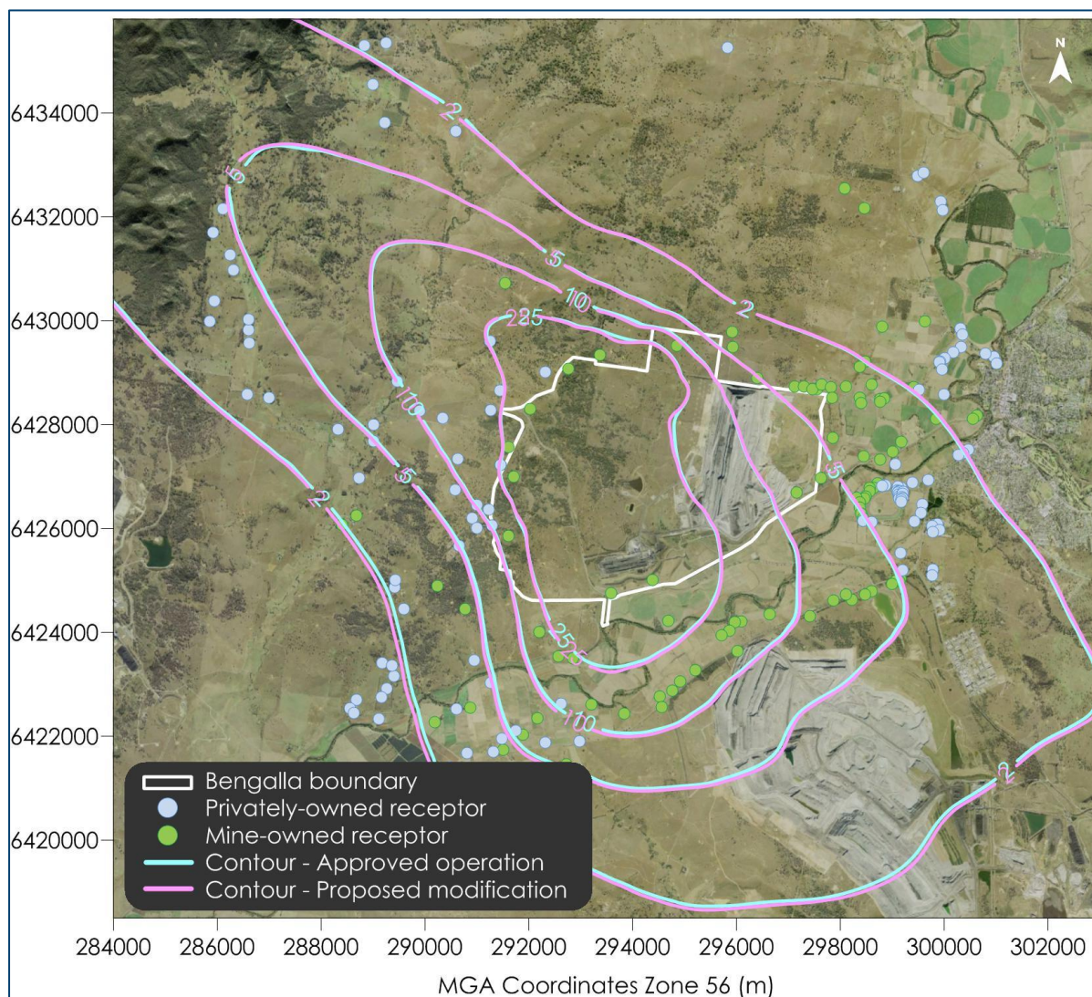
Figure 12: Comparison of predicted incremental annual average PM_{10} concentrations –Year 24 ( \mu g/m^3 )
