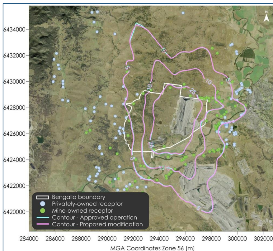
Figure 6: Comparison of predicted maximum incremental 24-hour average PM_{2.5} concentrations – Year 4 ( \mu g/m^3 )
