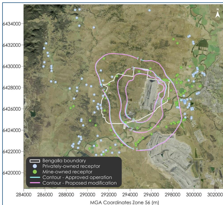
Figure 7: Comparison of predicted incremental annual average PM_{2.5} concentrations –Year 4 ( \mu g/m^3 )
