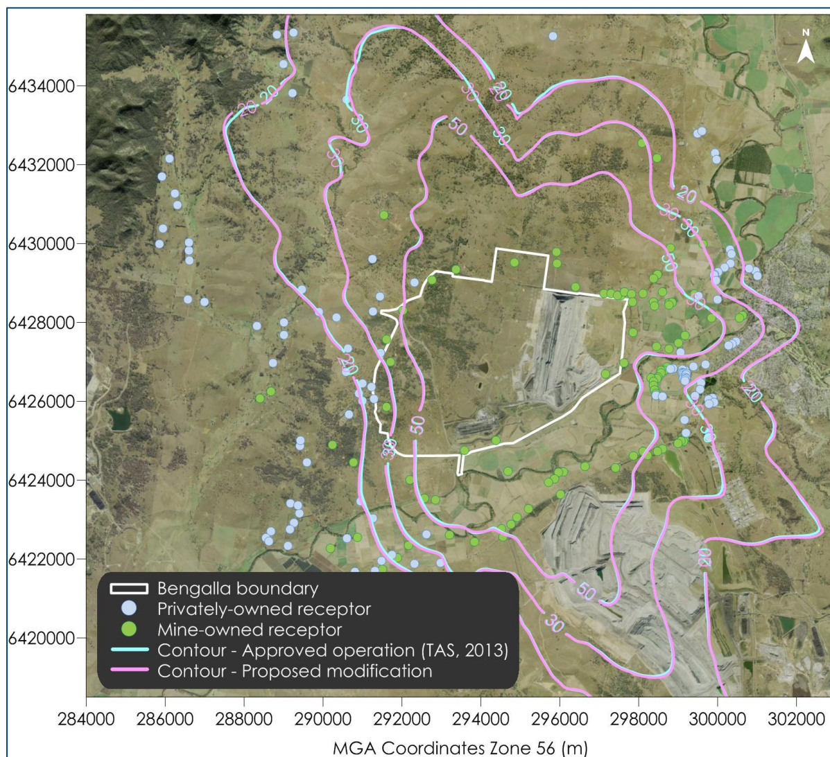
Figure 3: Comparison of predicted maximum incremental 24-hour average PM_{10} concentrations for proposed Modification as per MOD2 (TAS, 2016) –Year 4 ( \mu g/m^3 )
