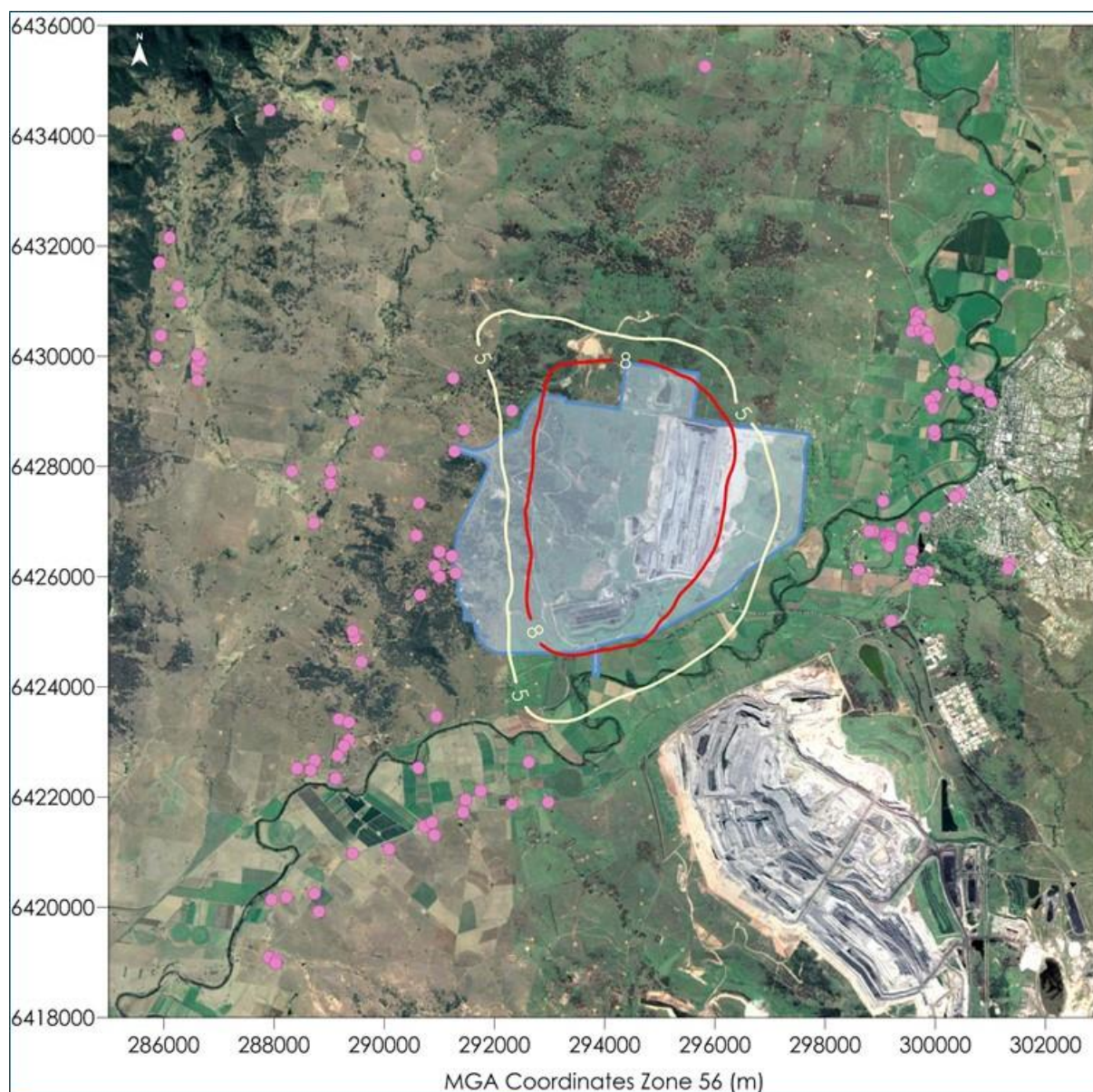
Figure C-23: Predicted annual average PM 2.5 concentrations due to emissions from Bengalla and other sources in Year 15 (µg/m 3 )
