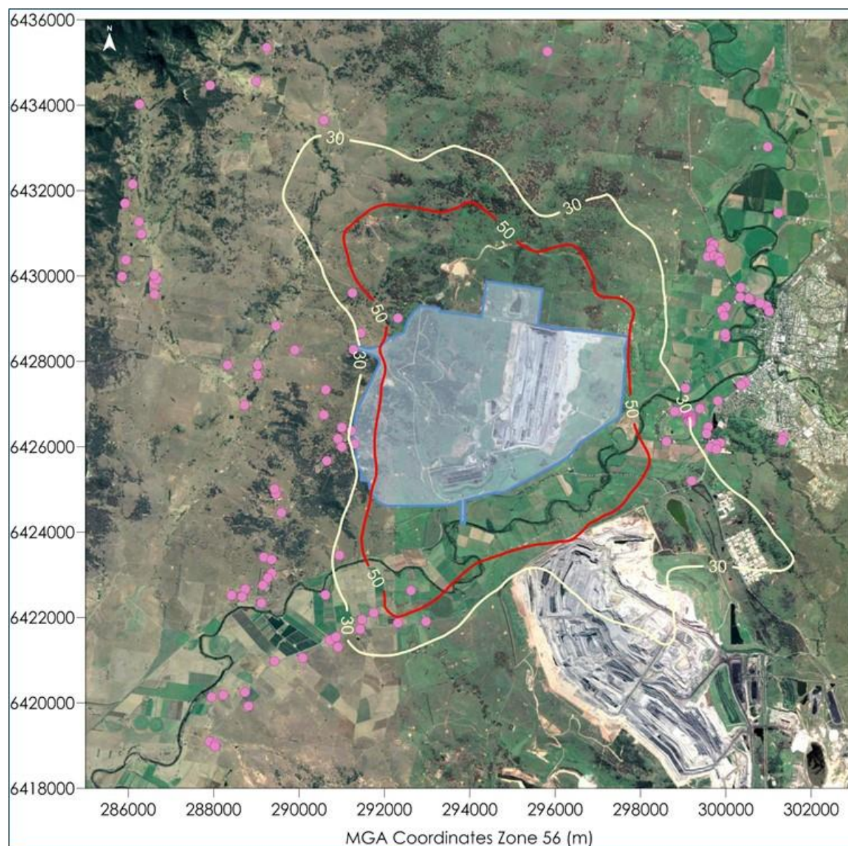
Figure C-24: Predicted maximum 24-hour average PM_{10} concentrations due to emissions from Bengalla in Year 15 ( \mu g/m^3 )
