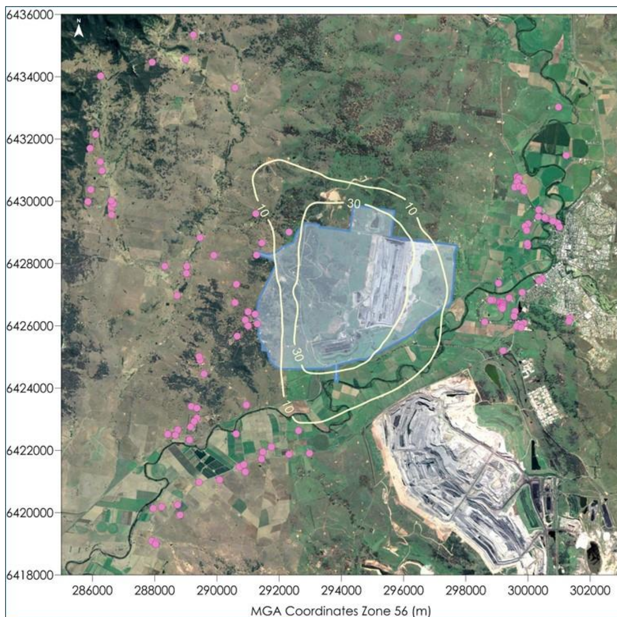
Figure C-25: Predicted annual average PM_{10} concentrations due to emissions from Bengalla in Year 15 ( \mu g/m^3 )
