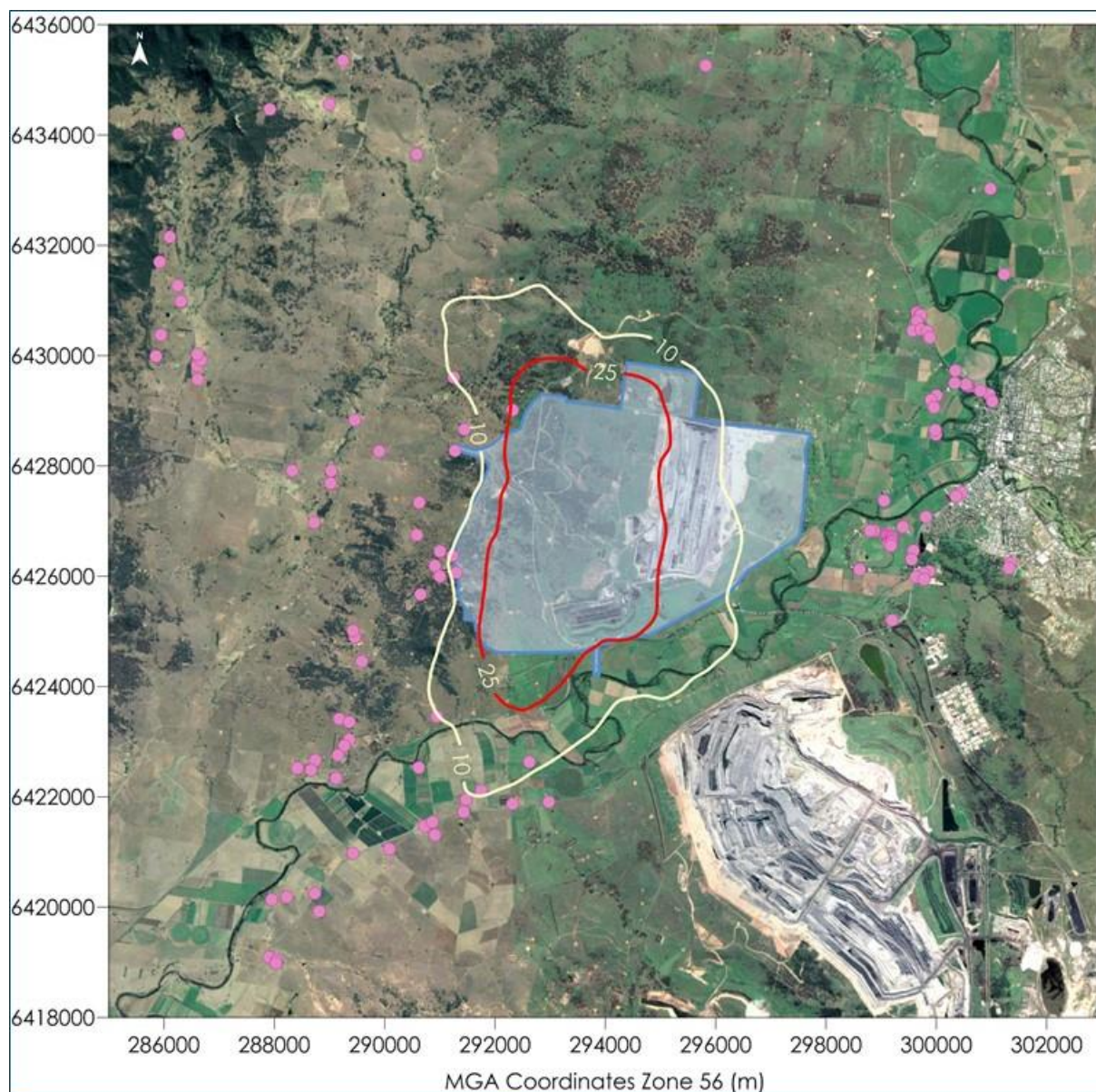
Figure C-31: Predicted maximum 24-hour average PM_{2.5} concentrations due to emissions from Bengalla in Year 24 ( \mu g/m^3 )
