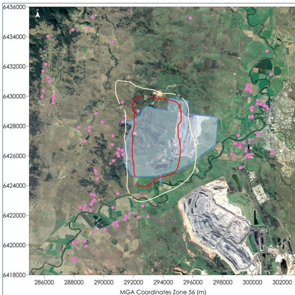
Figure C-33: Predicted annual average PM_{2.5} concentrations due to emissions from Bengalla and other sources in Year 24 ( \mu g/m^3 )
