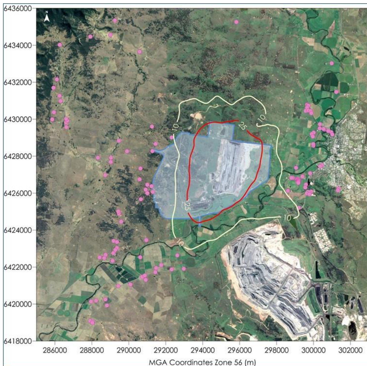
Figure C-11: Predicted maximum 24-hour average PM_{2.5} concentrations due to emissions from Bengalla in Year 8 ( \mu g/m^3 )
