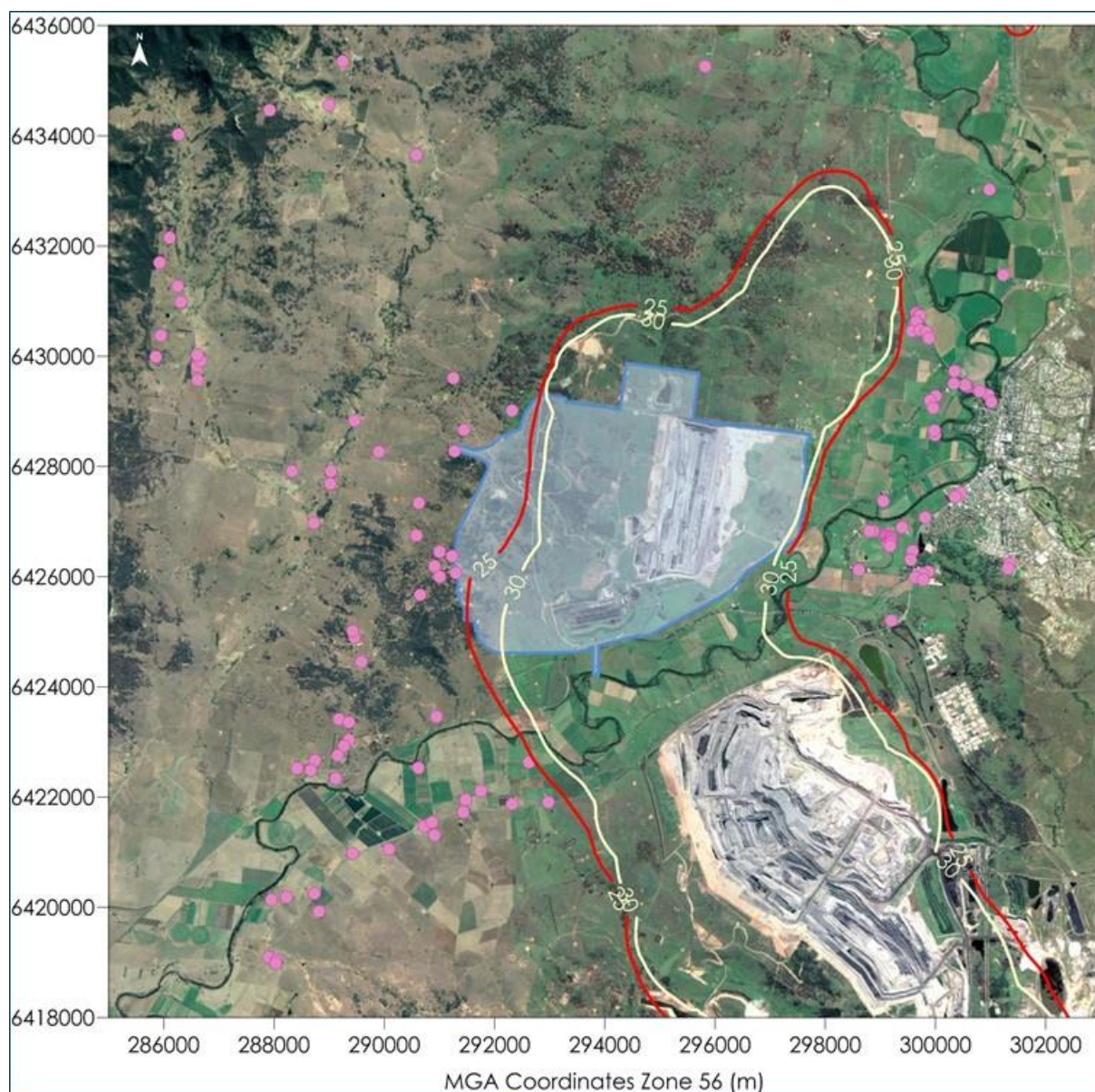
Figure C-6: Predicted annual average PM 10 concentrations due to emissions from Bengalla and other sources in Year 4 ( \mu\text{g}/\text{m}^3 )
