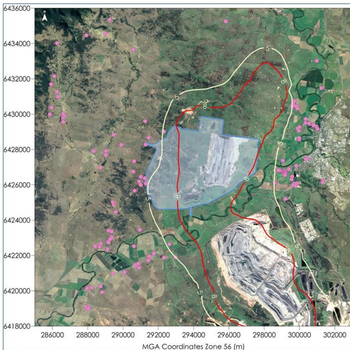
Figure C-3: Predicted annual average PM 2.5 concentrations due to emissions from Bengalla and other sources in Year 4 (µg/m 3 )
