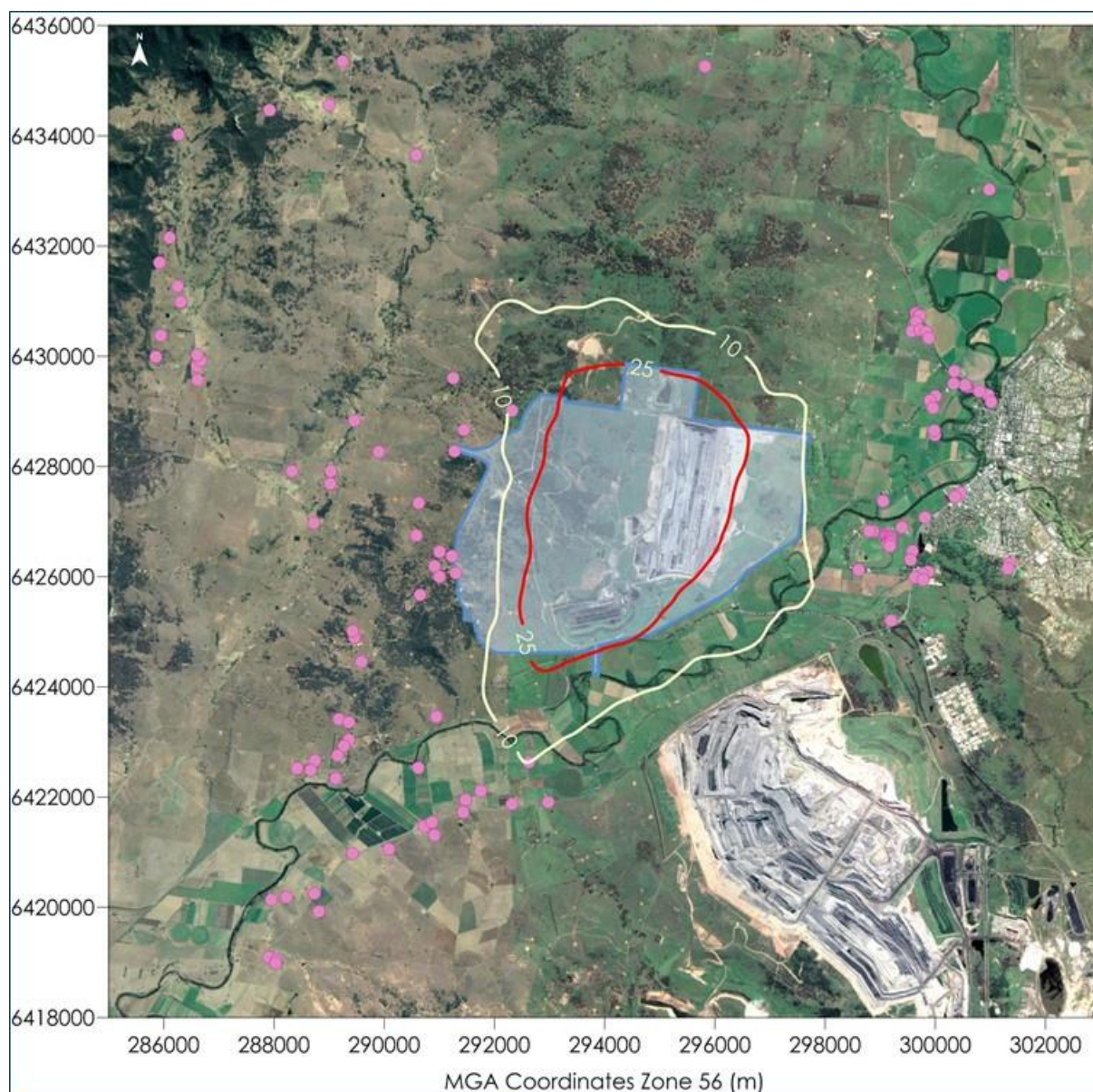
Figure C-21: Predicted maximum 24-hour average PM 2.5 concentrations due to emissions from Bengalla in Year 15 (µg/m 3 )
