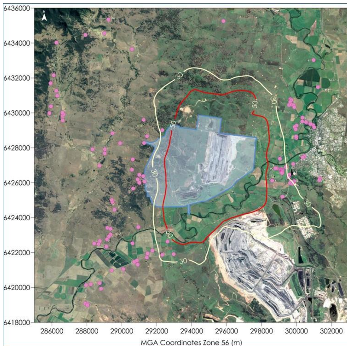
Figure C-4: Predicted maximum 24-hour average PM 10 concentrations due to emissions from Bengalla in Year 4 (µg/m 3 )
