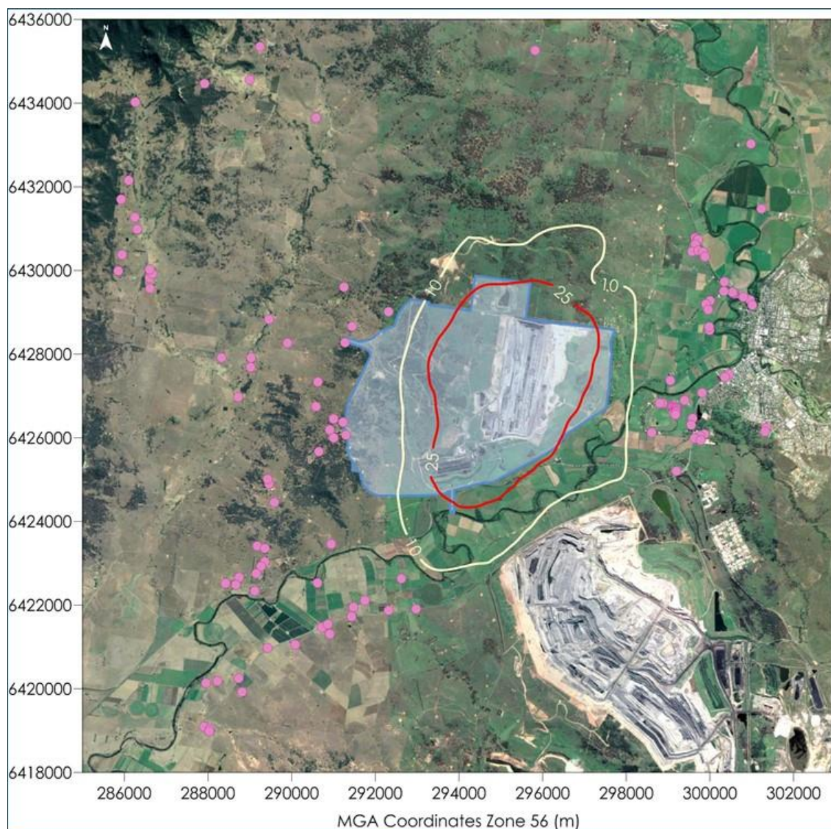
Figure C-1: Predicted maximum 24-hour average PM 2.5 concentrations due to emissions from Bengalla in Year 4 (µg/m 3 )
