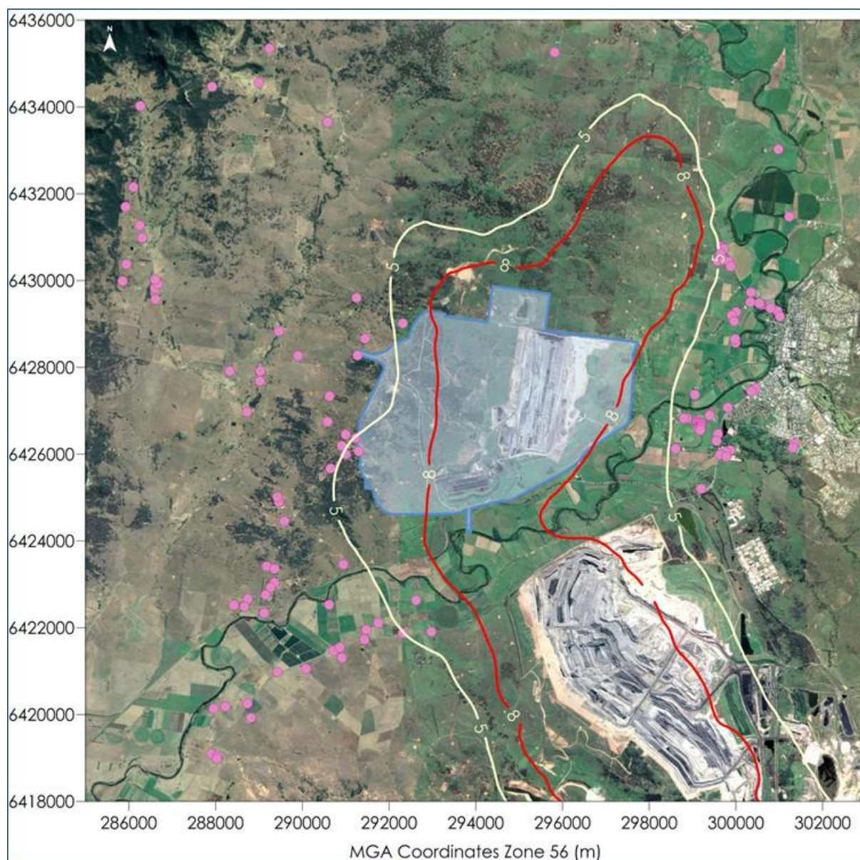
Figure C-13: Predicted annual average PM_{2.5} concentrations due to emissions from Bengalla and other sources in Year 8 ( \mu g/m^3 )
