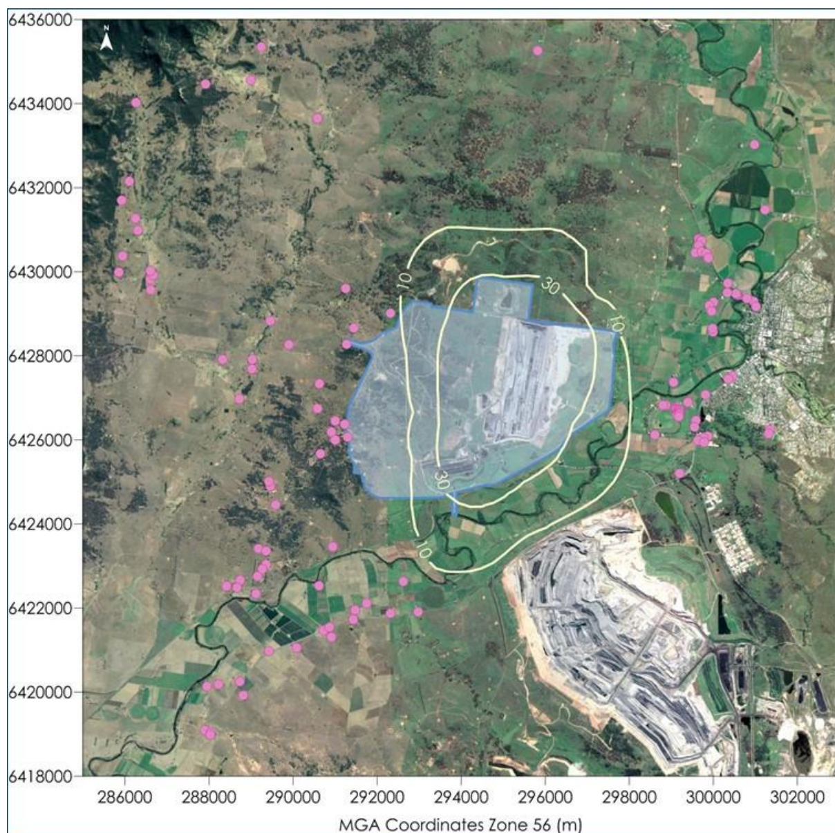
Figure C-5: Predicted annual average PM 10 concentrations due to emissions from Bengalla in Year 4 ( \mu\text{g}/\text{m}^3 )
