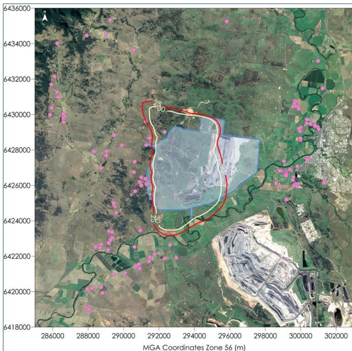
Figure C-36: Predicted annual average PM 10 concentrations due to emissions from Bengalla and other sources in Year 24 ( \mu\text{g}/\text{m}^3 )
