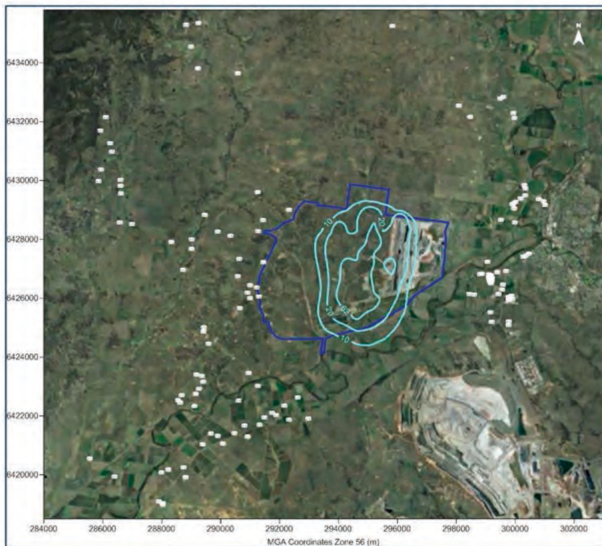
Figure G-4: Predicted annual average NO 2 concentrations from the Project in Year 4 (µg/m 3 )
