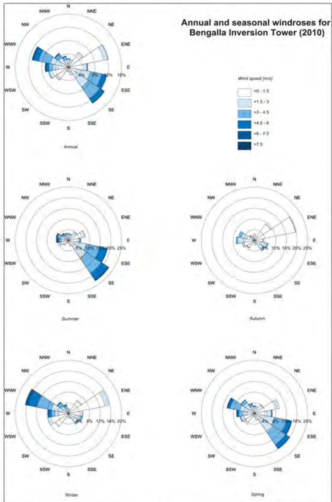
Figure 6-5: Annual and seasonal windroses for Bengalla inversion tower at 10m (2010)
