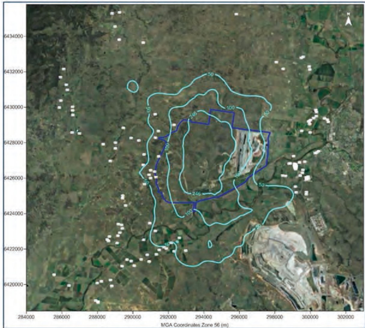
Figure G-7: Predicted 1-hour average NO 2 concentrations from the Project in Year 15 (µg/m 3 )
