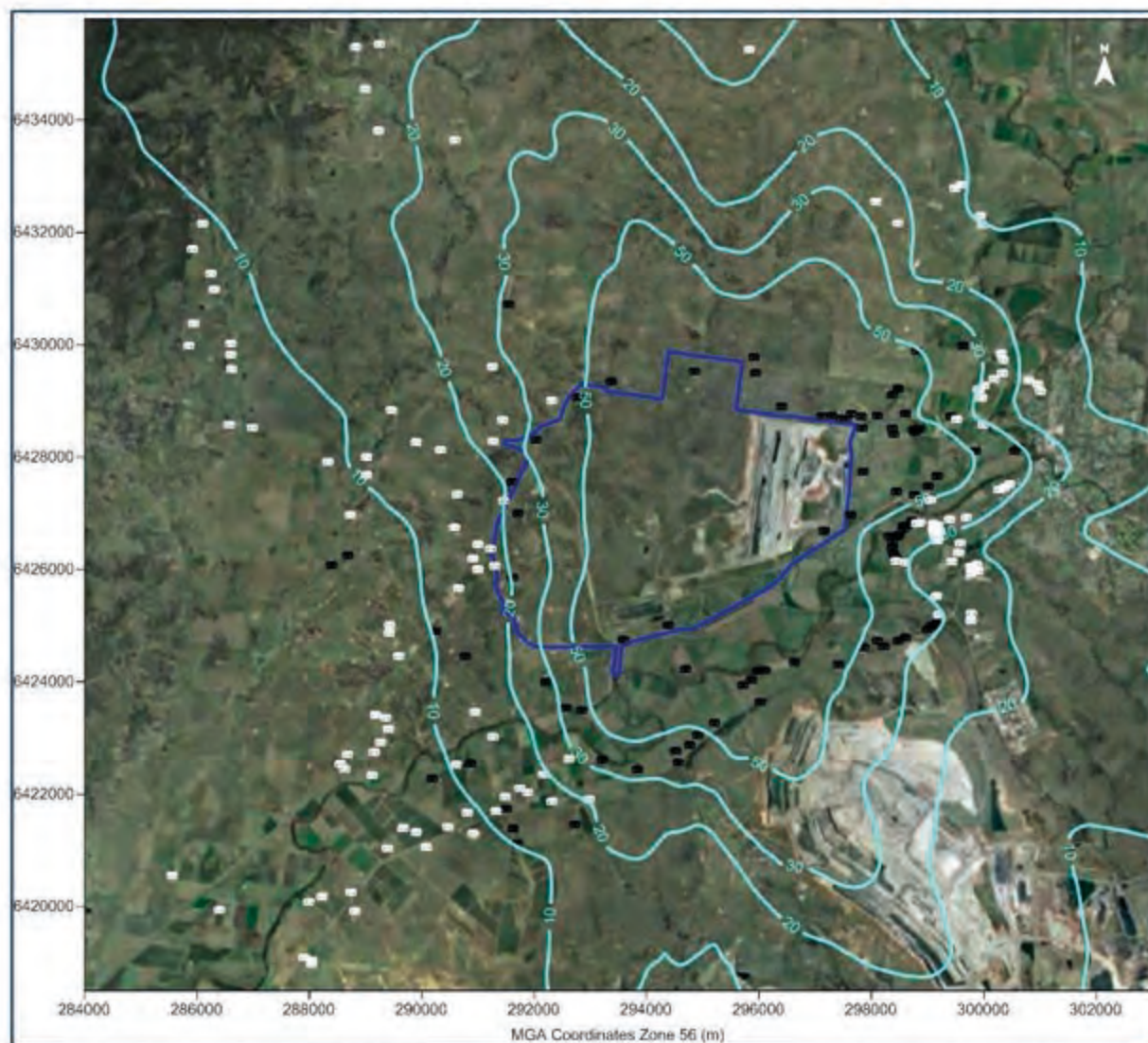
Figure E-3: Predicted maximum 24-hour average PM 10 concentrations due to emissions from the Project in Year 1 (µg/m³)
