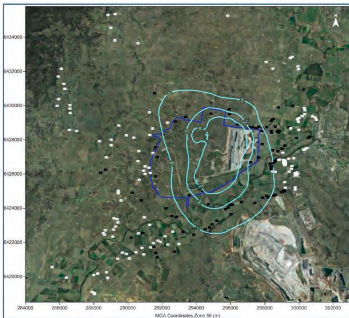
Figure E-2: Predicted annual average PM 2.5 concentrations due to emissions from the Project in Year 1 (µg/m 3 )
