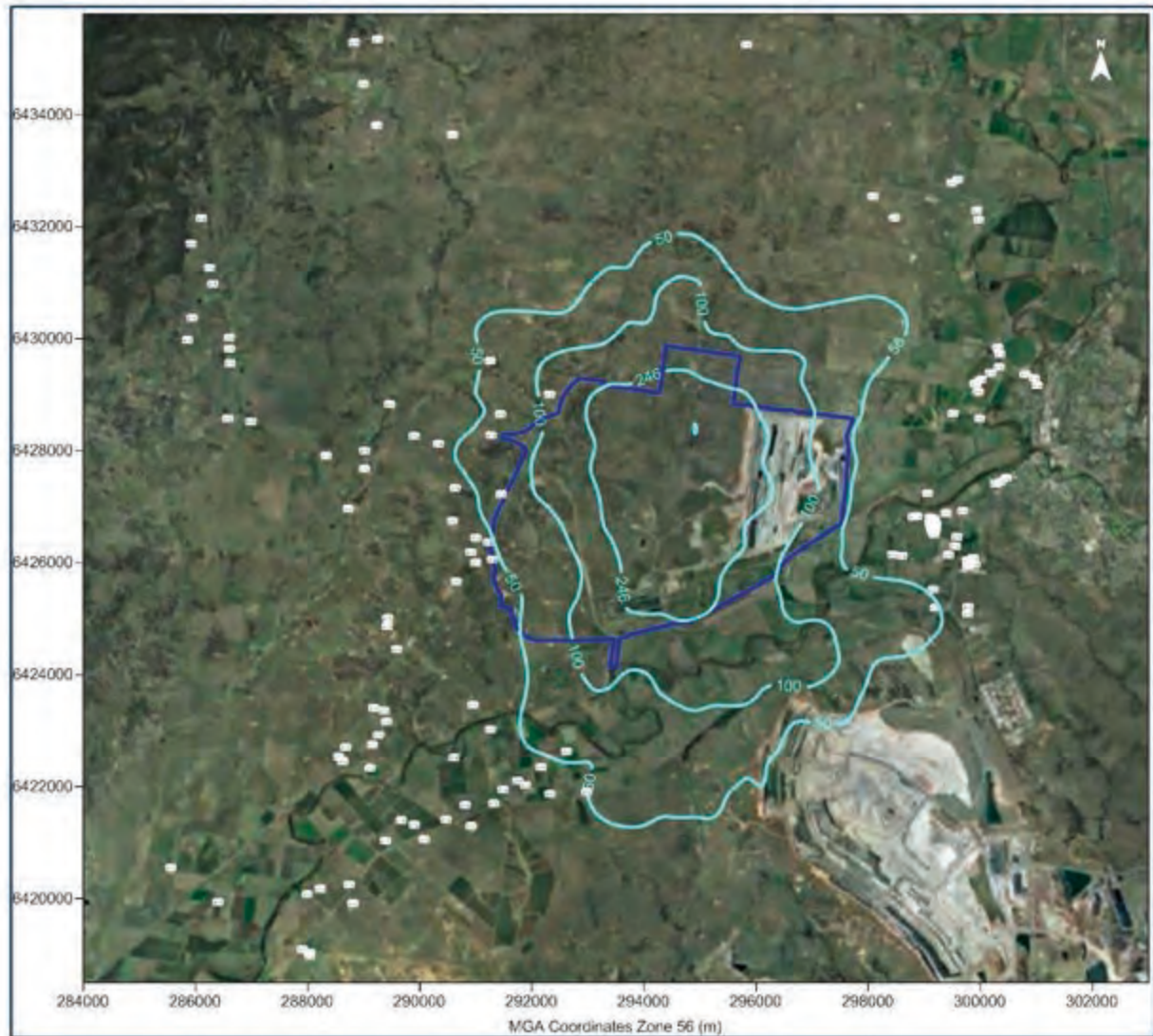
Figure G-5: Predicted 1-hour average \text{NO}_2 concentrations from the Project in Year 8 ( \mu\text{g}/\text{m}^3 )
