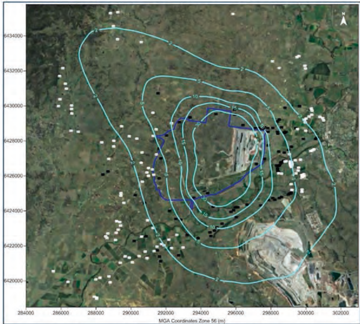
Figure E-4: Predicted annual average PM 10 concentrations due to emissions from the Project in Year 1 ( \mu\text{g}/\text{m}^3 )
