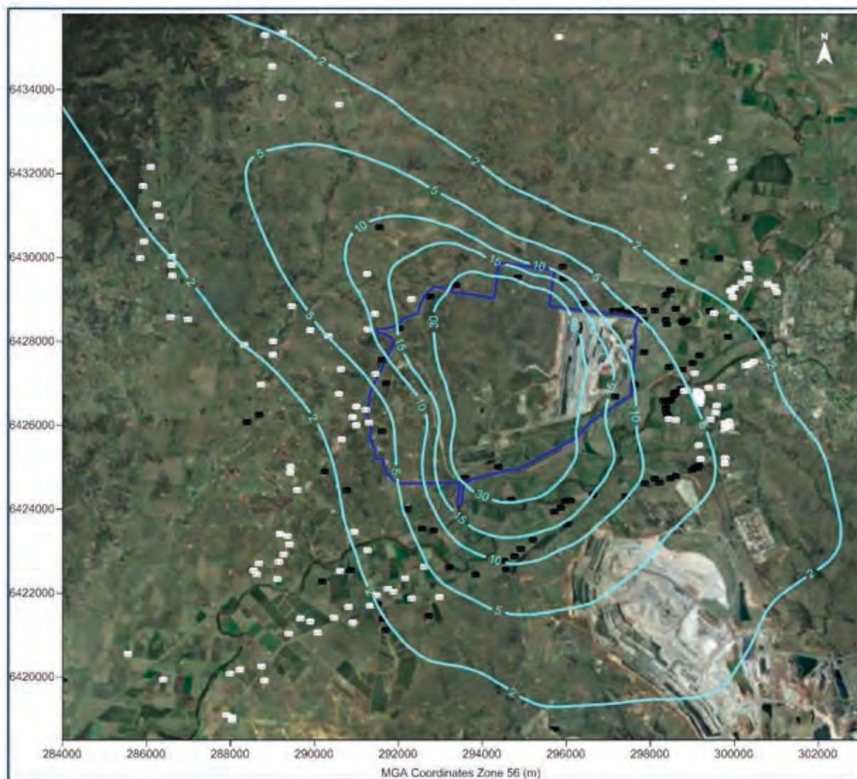
Figure E-22: Predicted annual average PM_{10} concentrations due to emissions from the Project in Year 8 ( \mu\text{g}/\text{m}^3 )
