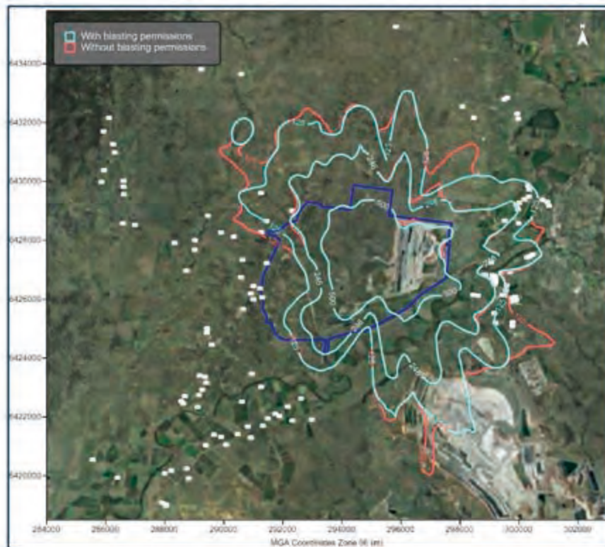
Figure H-11: Predicted maximum 1-hour average blast emissions from the Project in Year 1 - 17:00 (NO 2 concentrations µg/m³)
