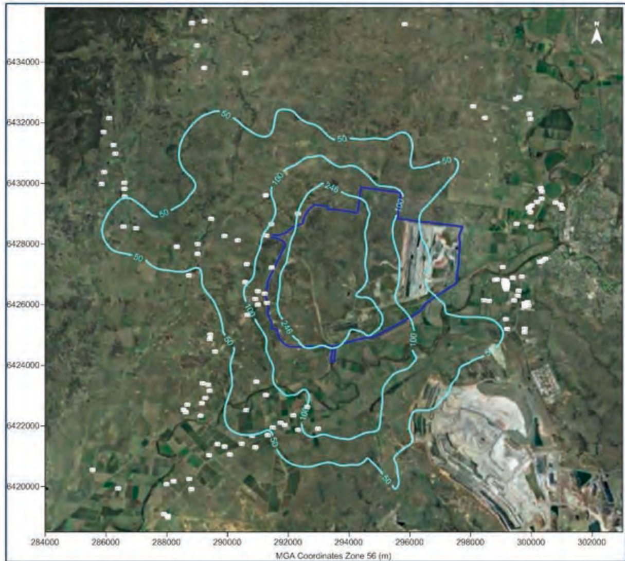
Figure G-9: Predicted 1-hour average NO 2 concentrations from the Project in Year 24 (µg/m 3 )
