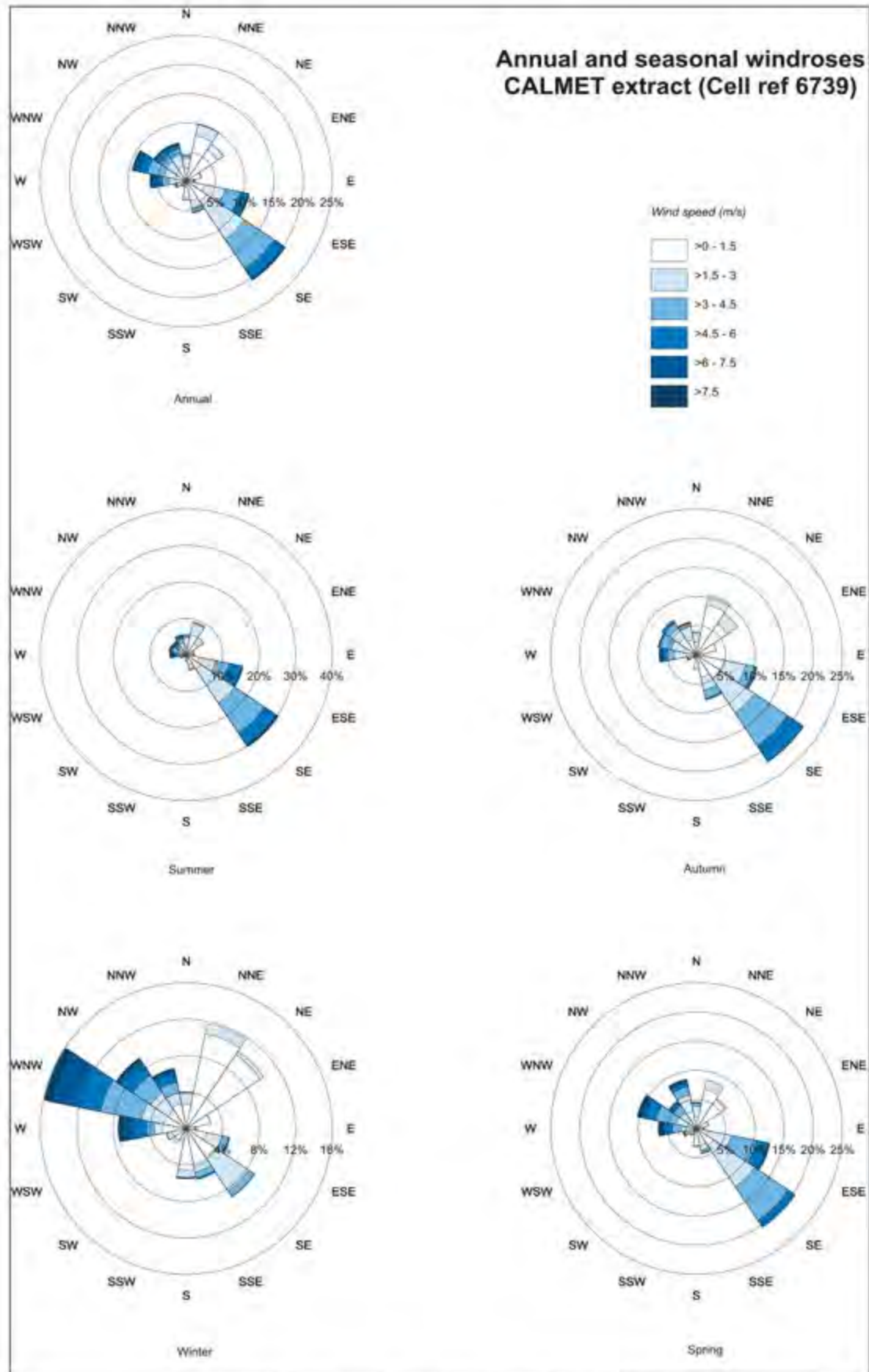
Figure 8-3: Windroses from CALMET extract (Cell Ref 6739)
