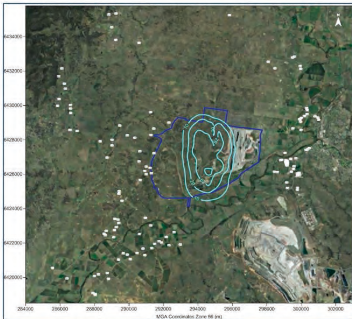
Figure G-6: Predicted annual average NO 2 concentrations from the Project in Year 8 (µg/m 3 )
