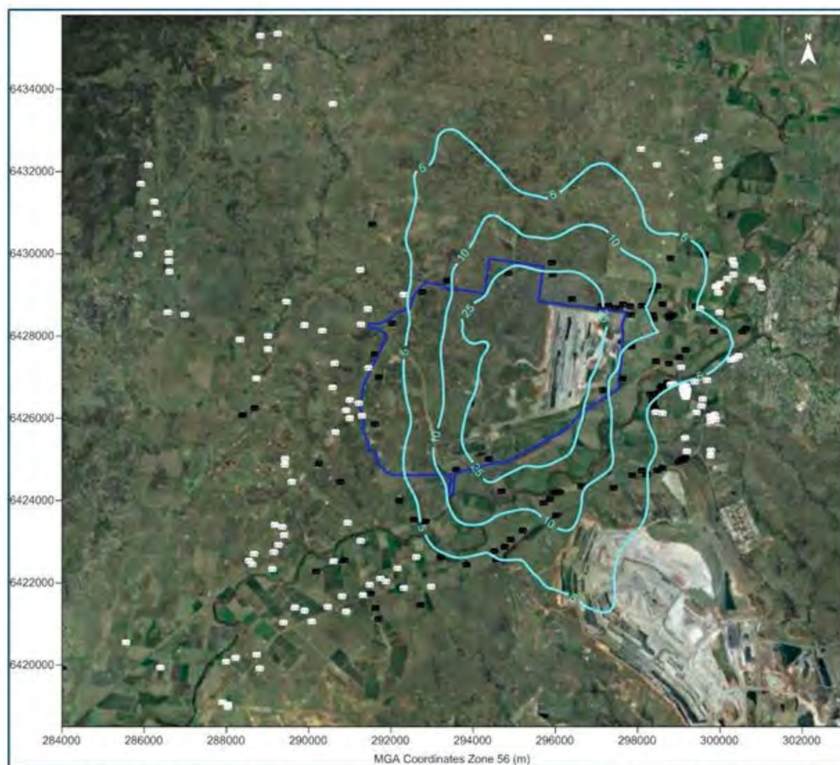
Figure E-1: Predicted maximum 24-hour average PM 2.5 concentrations due to emissions from the Project in Year 1 (µg/m³)
