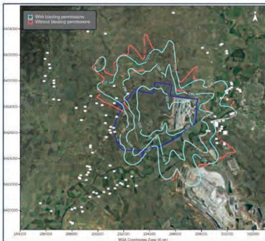
Figure H-22: Predicted maximum 1-hour average blast emissions from the Project in Year 4 - 17:00 (NO 2 concentrations µg/m³)
