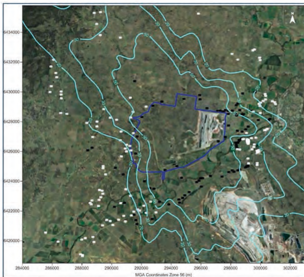
Figure E-21: Predicted maximum 24-hour average PM 10 concentrations due to emissions from the Project in Year 8 (µg/m³)
