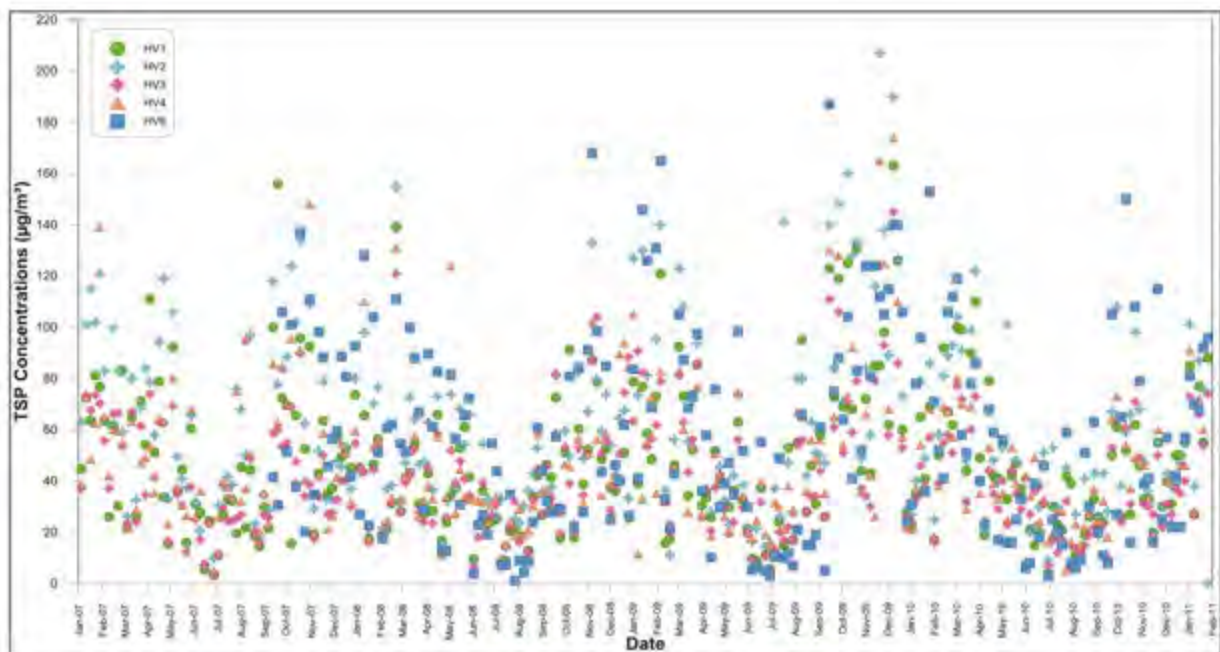
Figure 6-10: HVAS 24-hour average TSP concentrations at BMC monitors
