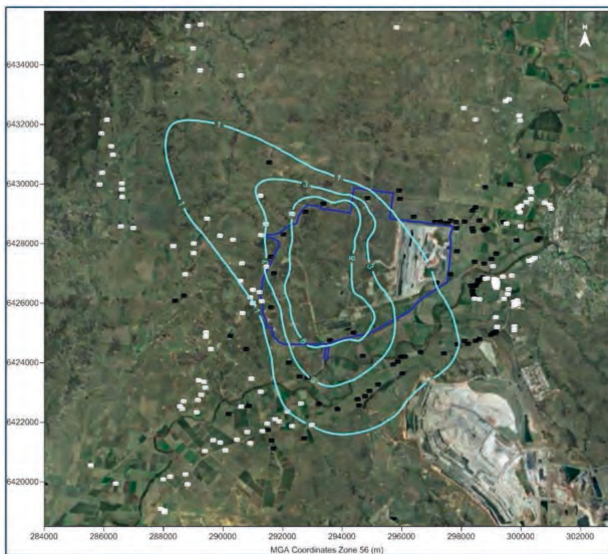
Figure E-38: Predicted annual average PM_{2.5} concentrations due to emissions from the Project in Year 24 ( \mu g/m^3 )
