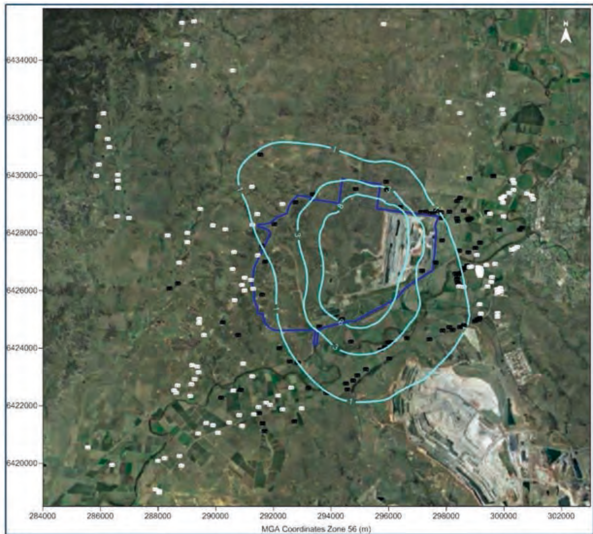
Figure E-11: Predicted annual average PM_{2.5} concentrations due to emissions from the Project in Year 4 ( \mu g/m^3 )
