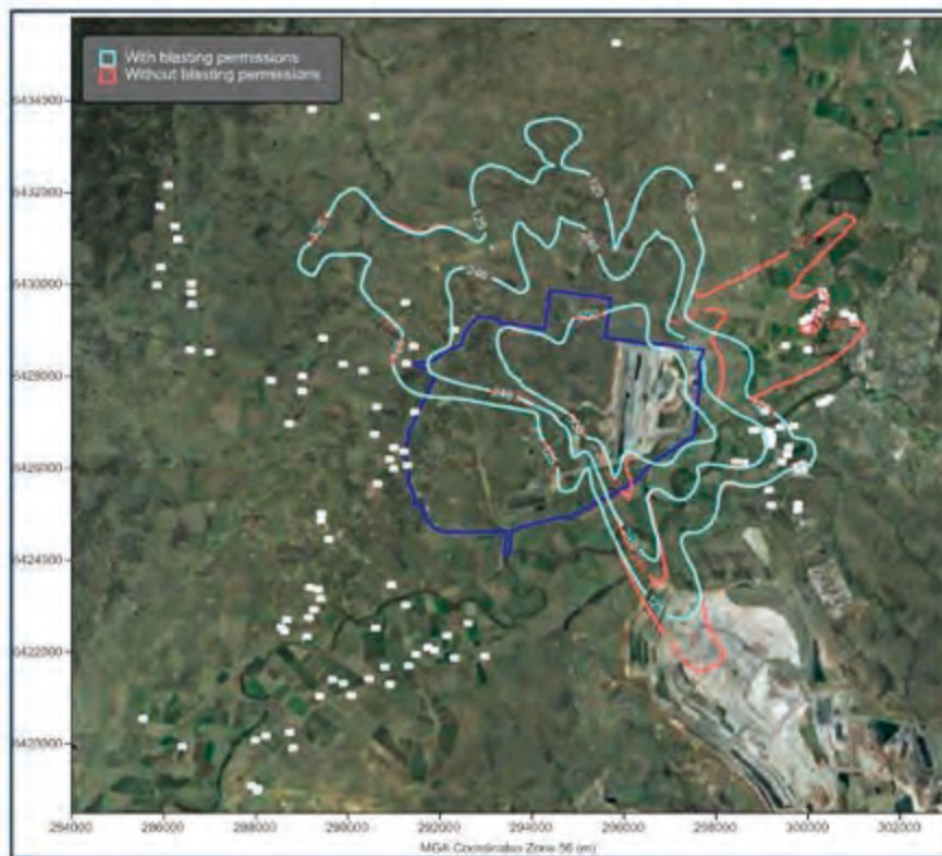
Figure H-10: Predicted maximum 1-hour average blast emissions from the Project in Year 1 - 16:00 (NO 2 concentrations µg/m³)
