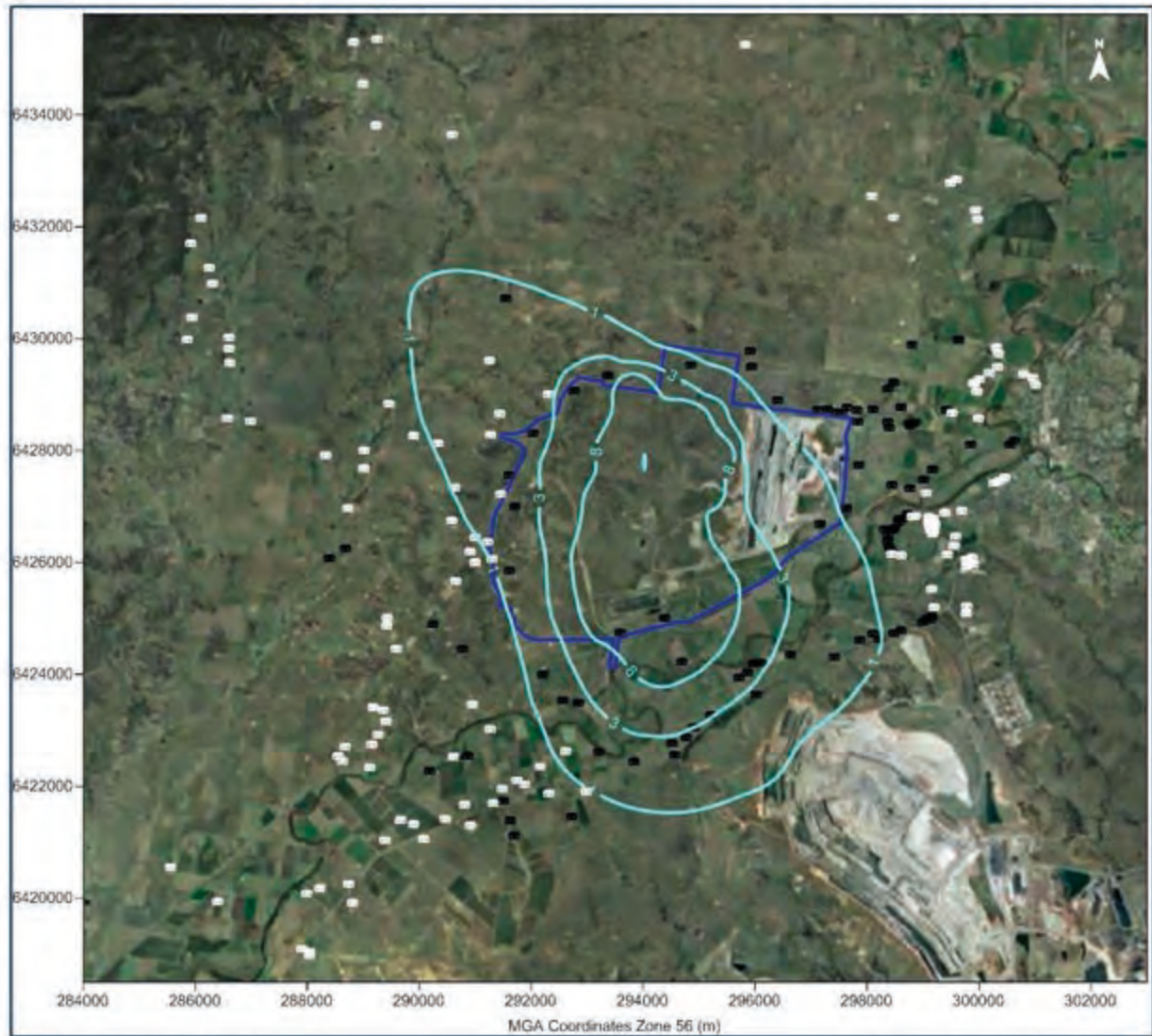
Figure E-29: Predicted annual average PM 2.5 concentrations due to emissions from the Project in Year 15 (µg/m 3 )
