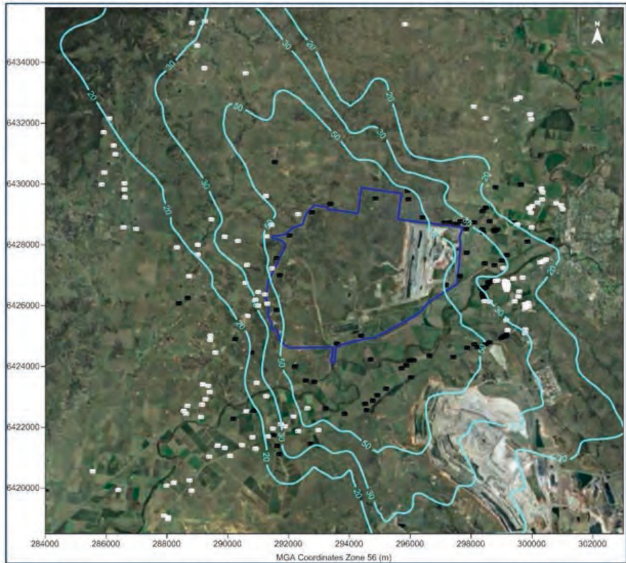
Figure E-30: Predicted maximum 24-hour average PM_{10} concentrations due to emissions from the Project in Year 15 ( \mu g/m^3 )
