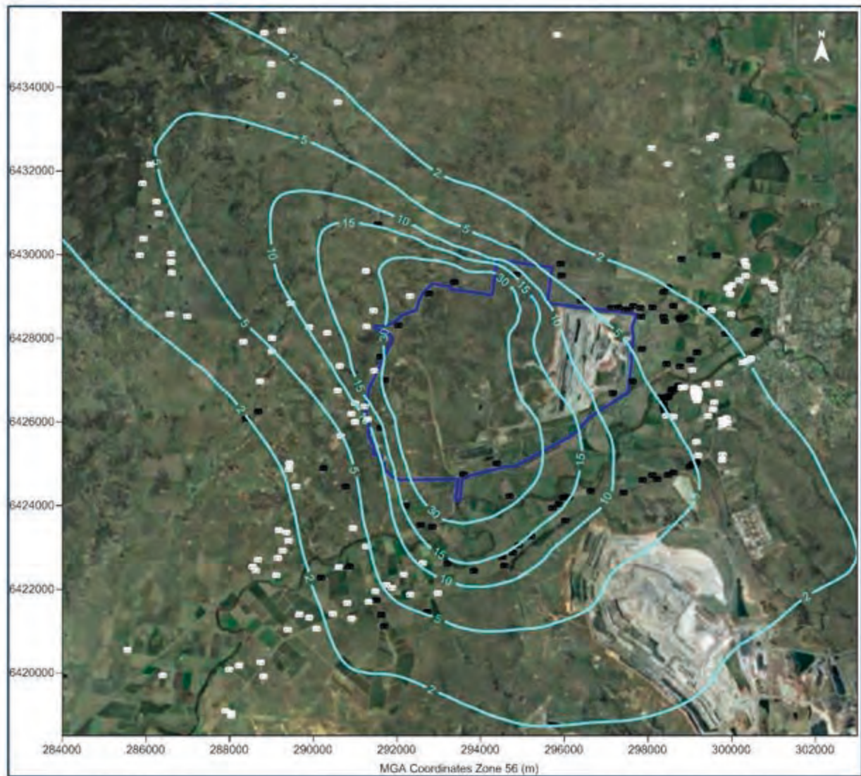
Figure E-40: Predicted annual average PM 10 concentrations due to emissions from the Project in Year 24 ( \mu\text{g}/\text{m}^3 )
