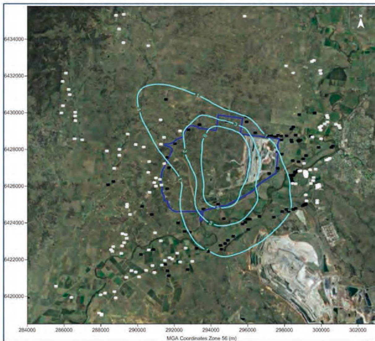
Figure E-20: Predicted annual average PM 2.5 concentrations due to emissions from the Project in Year 8 (µg/m 3 )
