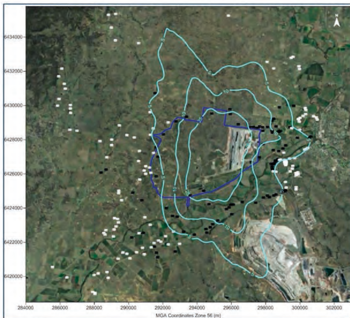
Figure E-10: Predicted maximum 24-hour average PM 2.5 concentrations due to emissions from the Project in Year 4 (µg/m³)
