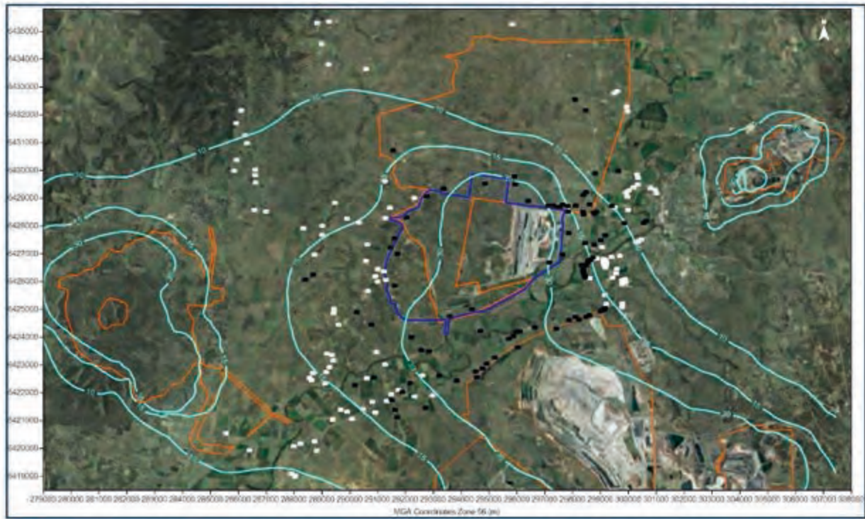
Figure E-5: Predicted annual average PM_{10} concentrations due to emissions from the Project and other sources in Year 1 ( \mu\text{g}/\text{m}^3 )
