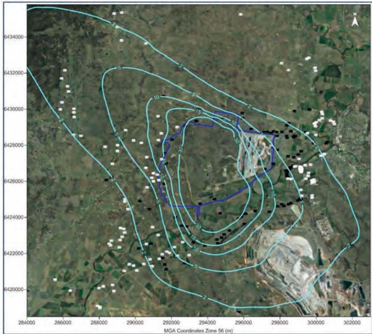
Figure E-31: Predicted annual average PM 10 concentrations due to emissions from the Project in Year 15 (µg/m 3 )
