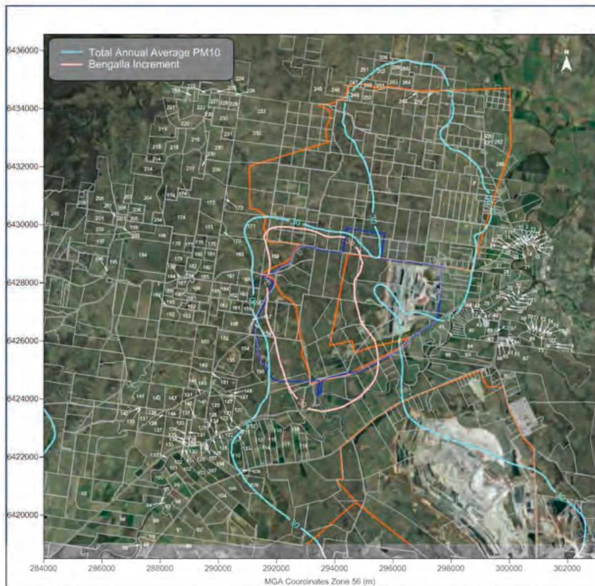
Figure E-50: Predicted annual average \text{PM}_{10} concentrations for properties due to emissions from the Project and other sources in Year 24 ( \mu\text{g}/\text{m}^3 )
