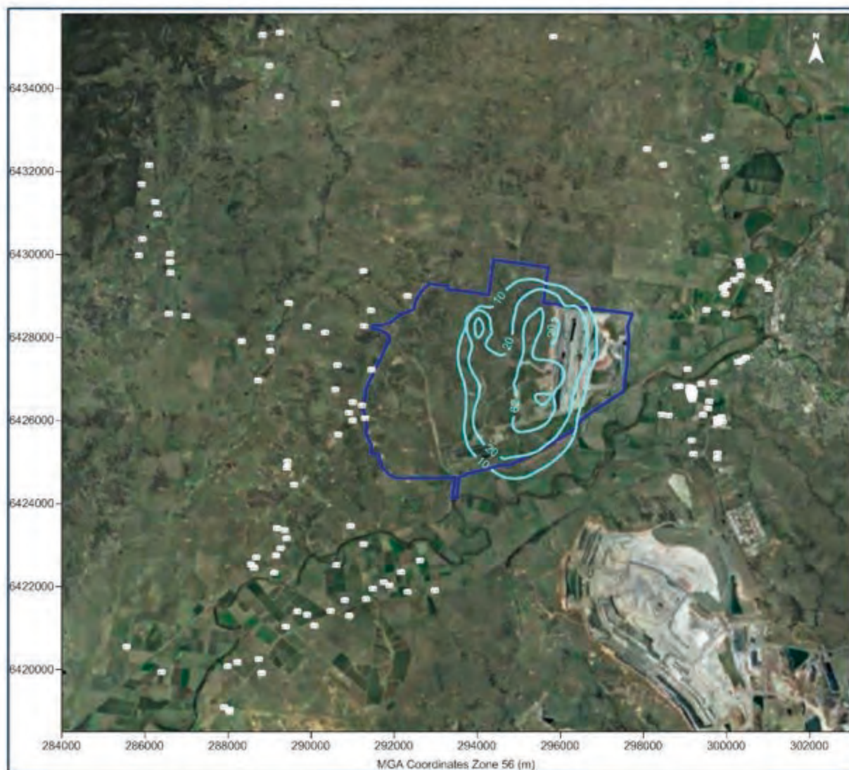
Figure G-2: Predicted annual average NO 2 concentrations from the Project in Year 1 (µg/m 3 )
