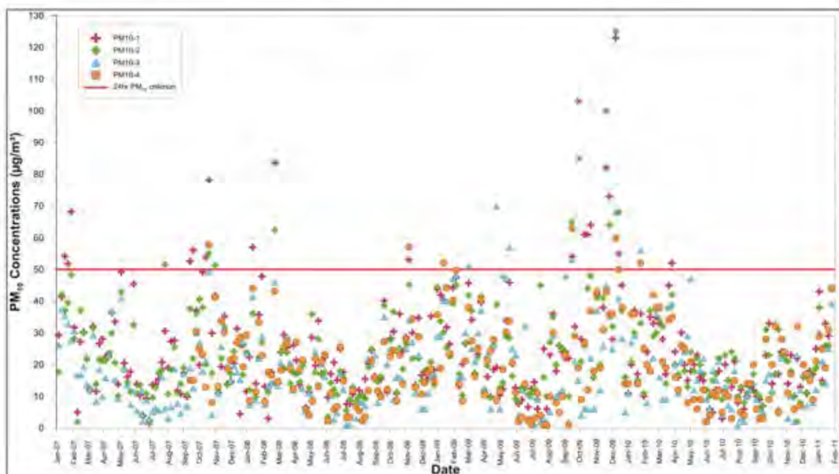
Figure 6-9: HVA5 24-hour average PM_{10} concentrations at BMC monitors
