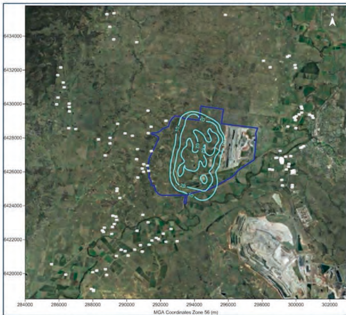
Figure G-8: Predicted annual average NO 2 concentrations from the Project in Year 15 ( \mu\text{g}/\text{m}^3 )
