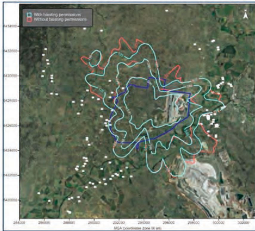
Figure H-33: Predicted maximum 1-hour average blast emissions from the Project in Year 8 - 17:00 ( \text{NO}_2 concentrations \mu\text{g}/\text{m}^3 )
