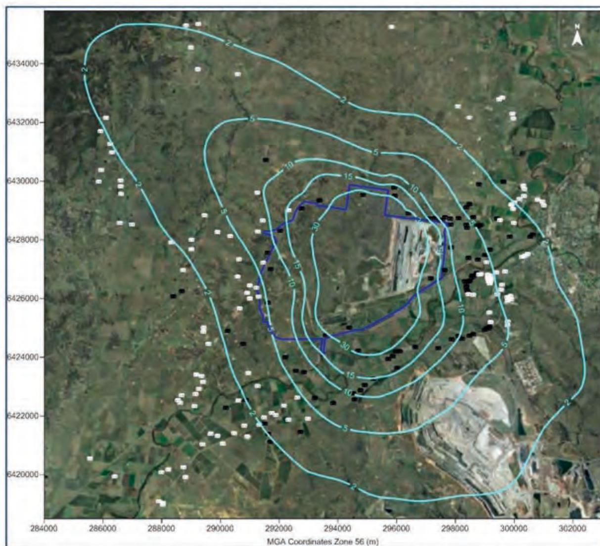
Figure E-13: Predicted annual average PM 10 concentrations due to emissions from the Project in Year 4 (µg/m 3 )
