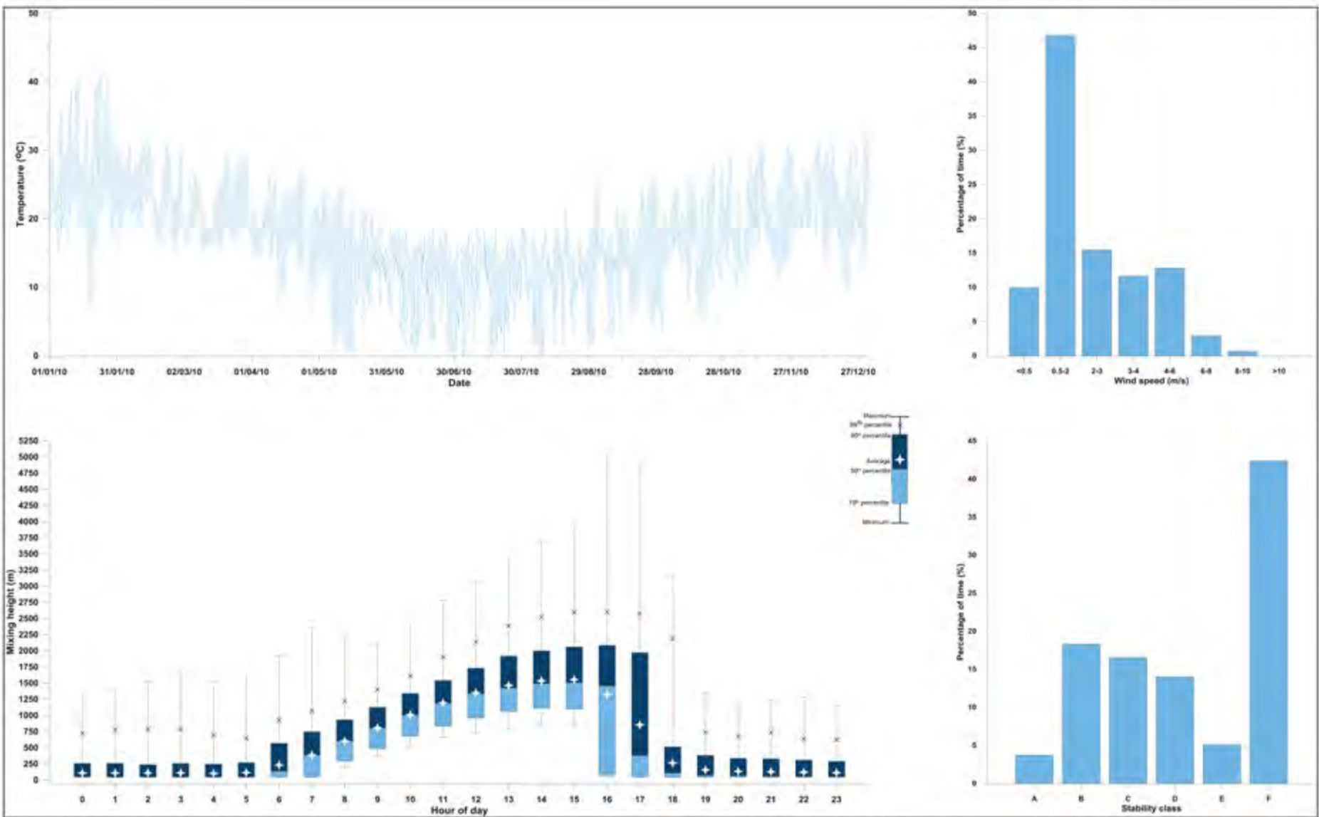
Figure 8-4: Meteorological analysis of CALMET extract (Cell Ref 6739)
