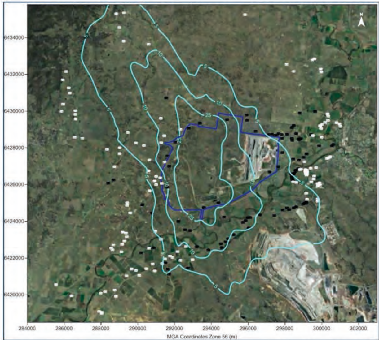
Figure E-37: Predicted maximum 24-hour average PM 2.5 concentrations due to emissions from the Project in Year 24 (µg/m 3 )
