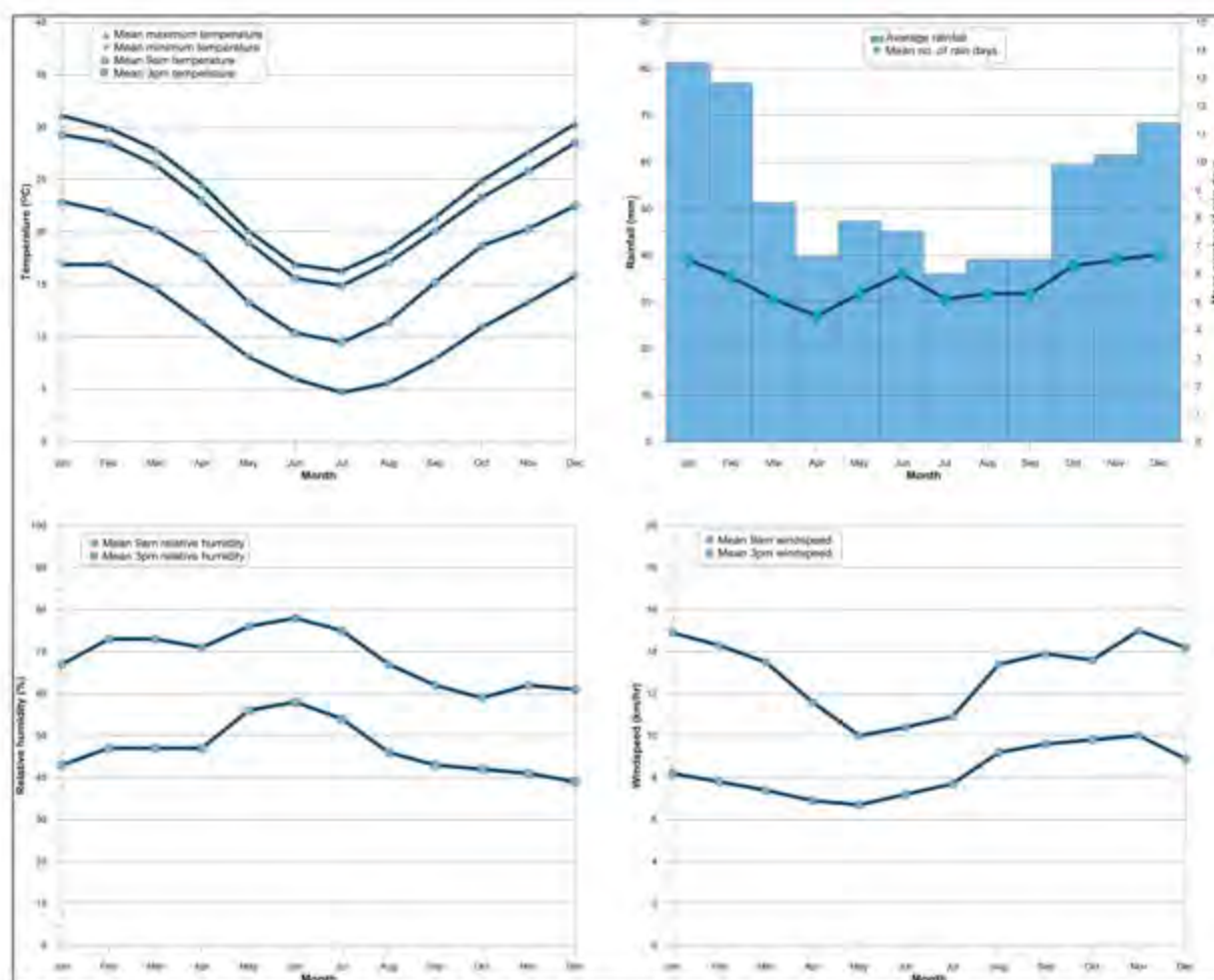
Figure 6-2: Monthly climate statistics summary - Scone SCS
