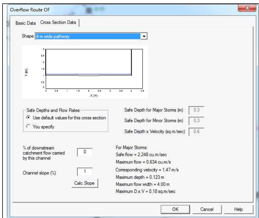
Figure 3.2 – Critical Overland Flow Path across Wicks/Waterloo Intersection
