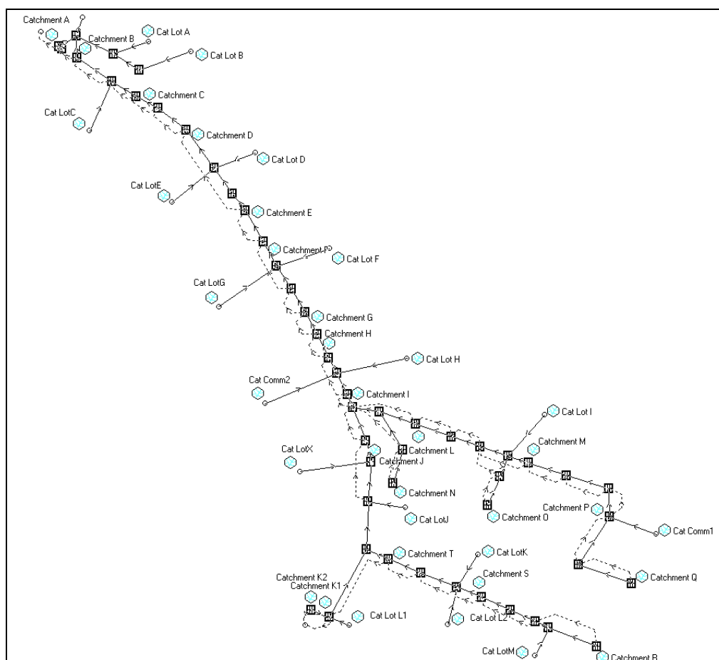
Figure 5.1 – M2 Site DRAINS Network Diagram
