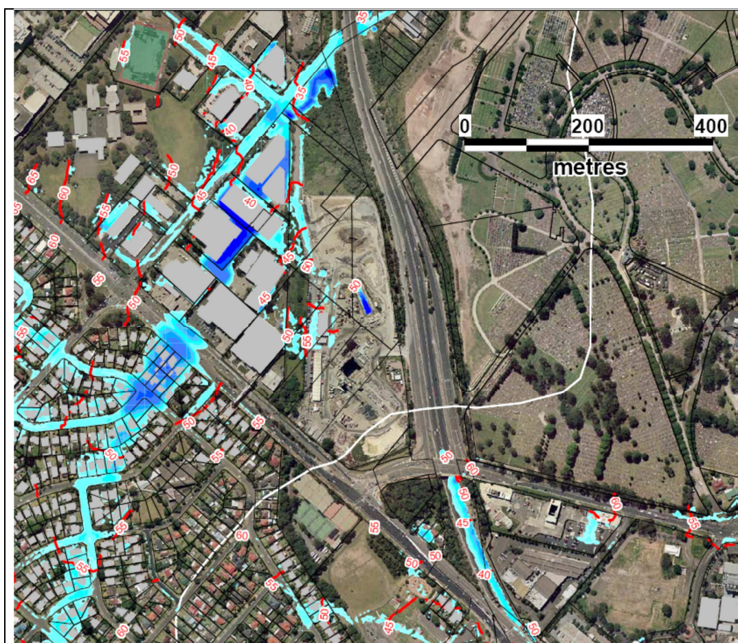
Figure 3.3 – Simulation of 100 Year ARI Flood (Bewsher, April 2010)
