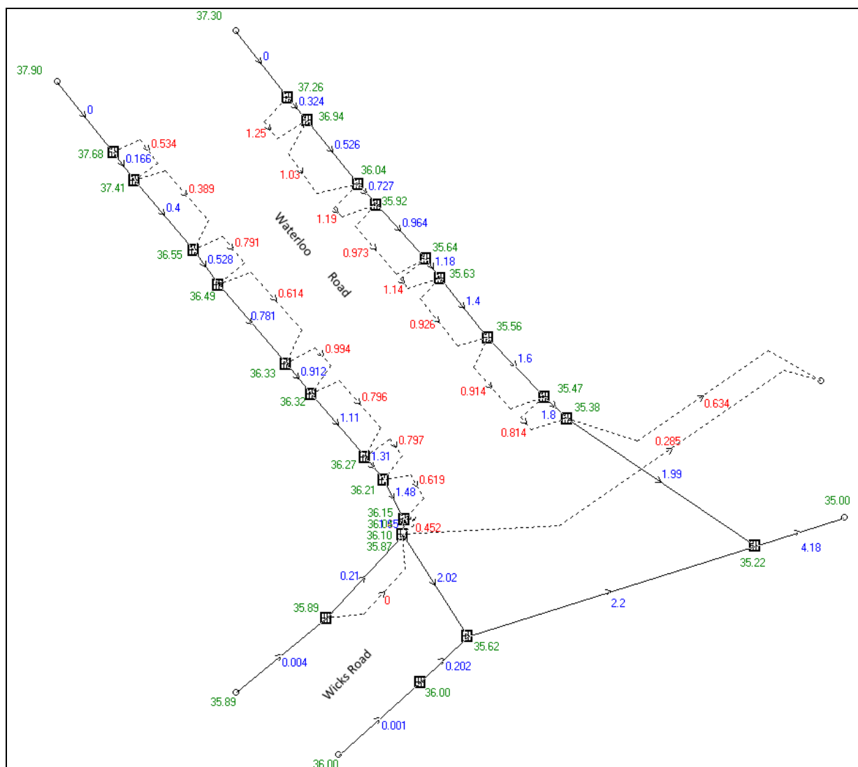
Figure 3.1 – DRAINS Network Diagram
