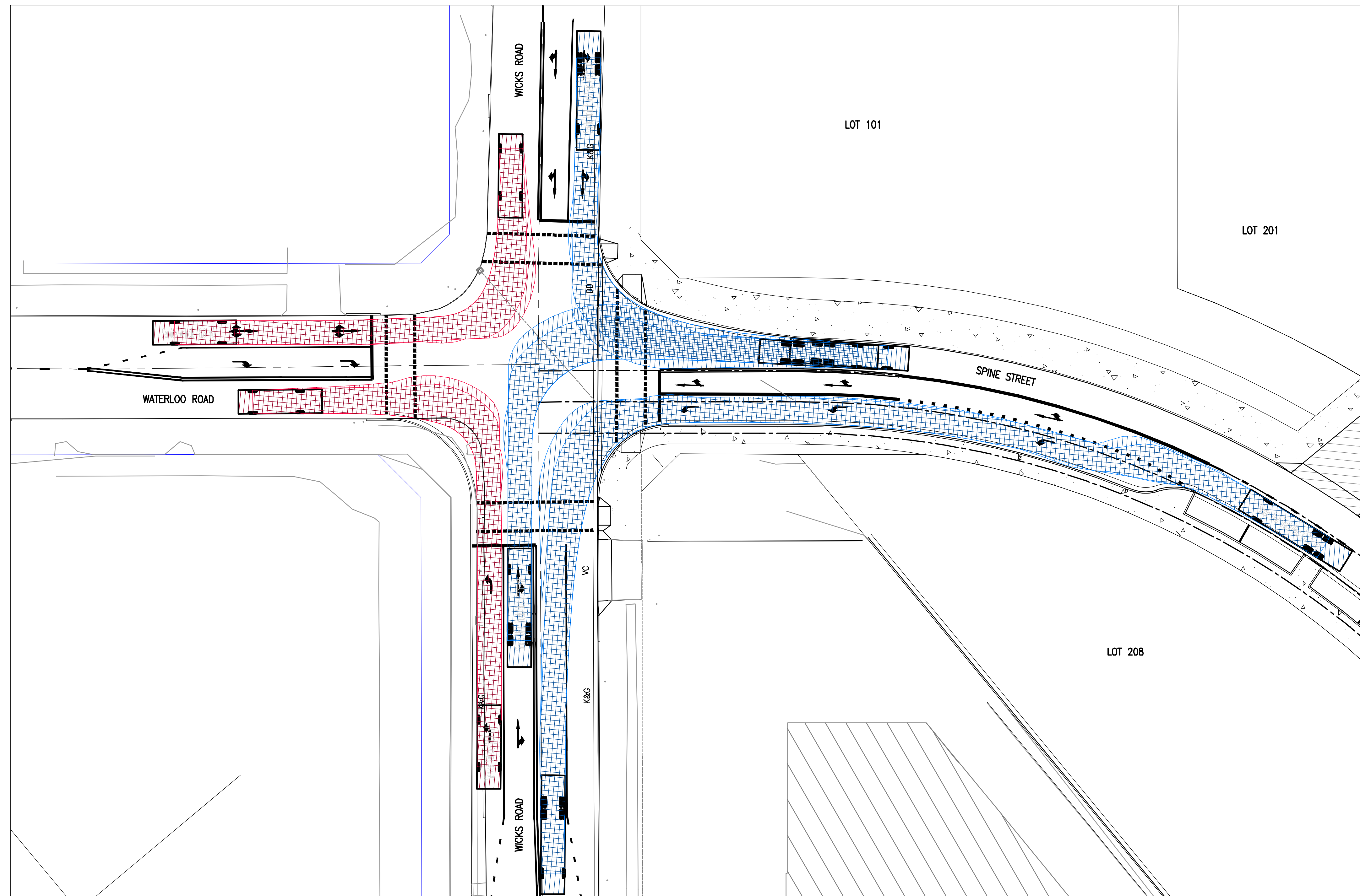
VEHICLE SWEEP PATHS – VIEW 1 WICKS, WATERLOO AND SPINE STREET INTERSECTION
