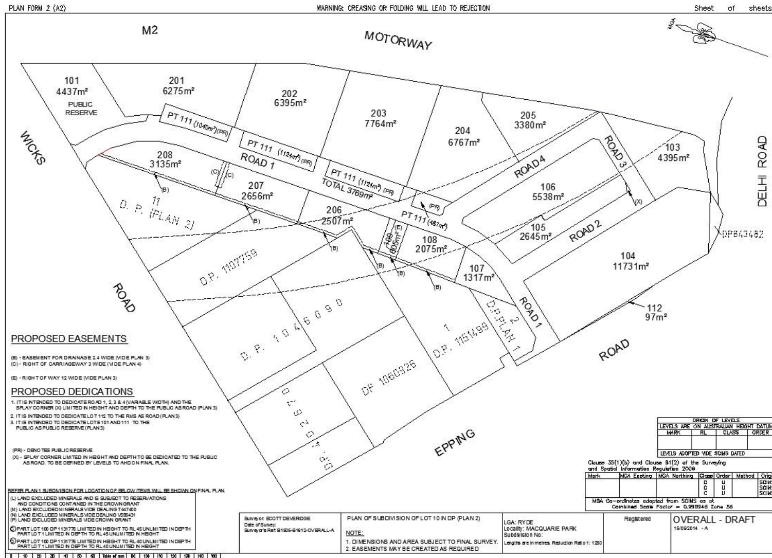
Figure 2: Allotment Subdivision Plan for the M2 Site (figure provided by client)
