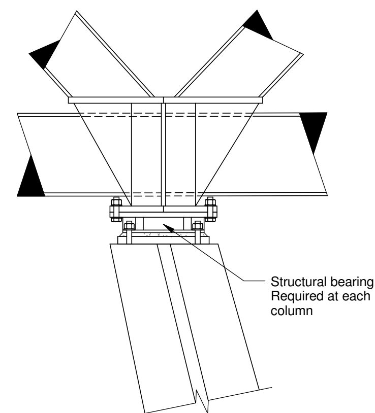
Bearing Detail Scale: 1 : 15
