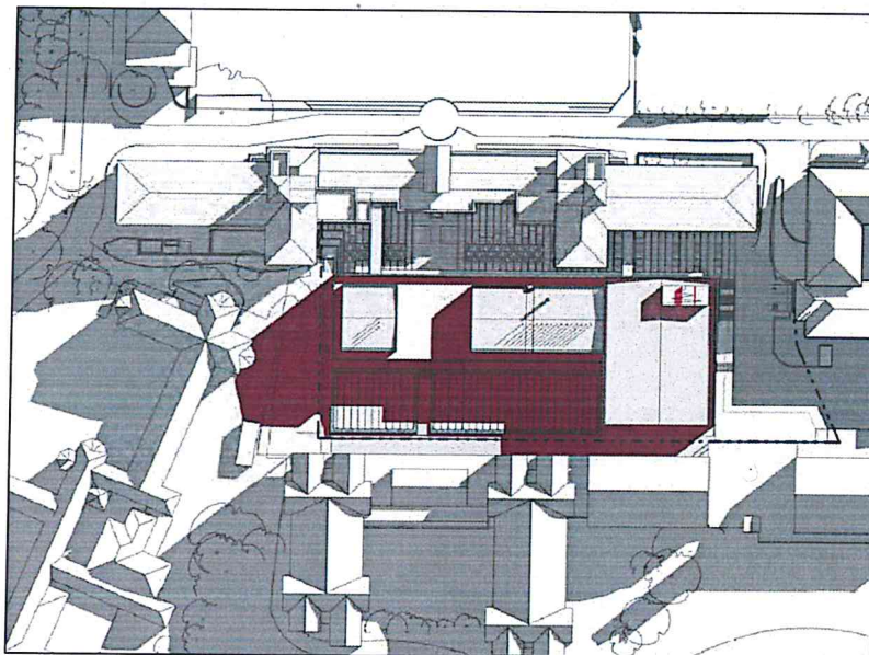
Figure 18: Winter 9:00 am Shadow Diagram
