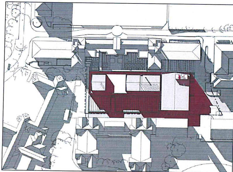
Figure 20: Winter 3:00 pm Shadow Diagram
