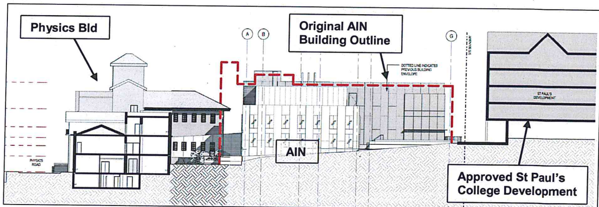
Figure 8: North-South Section (Original Proposal Outlined Red)
