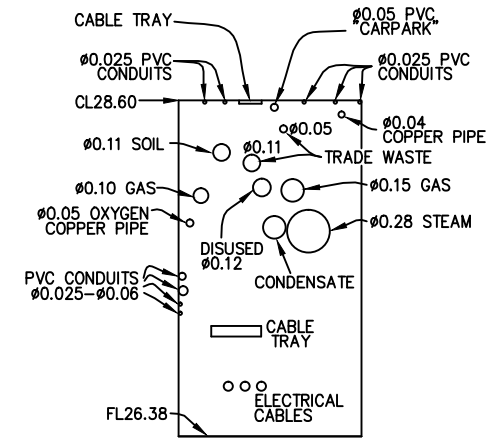
SECTION C-C SERVICE TUNNEL NEAR COFFEE SHOP 1:50
